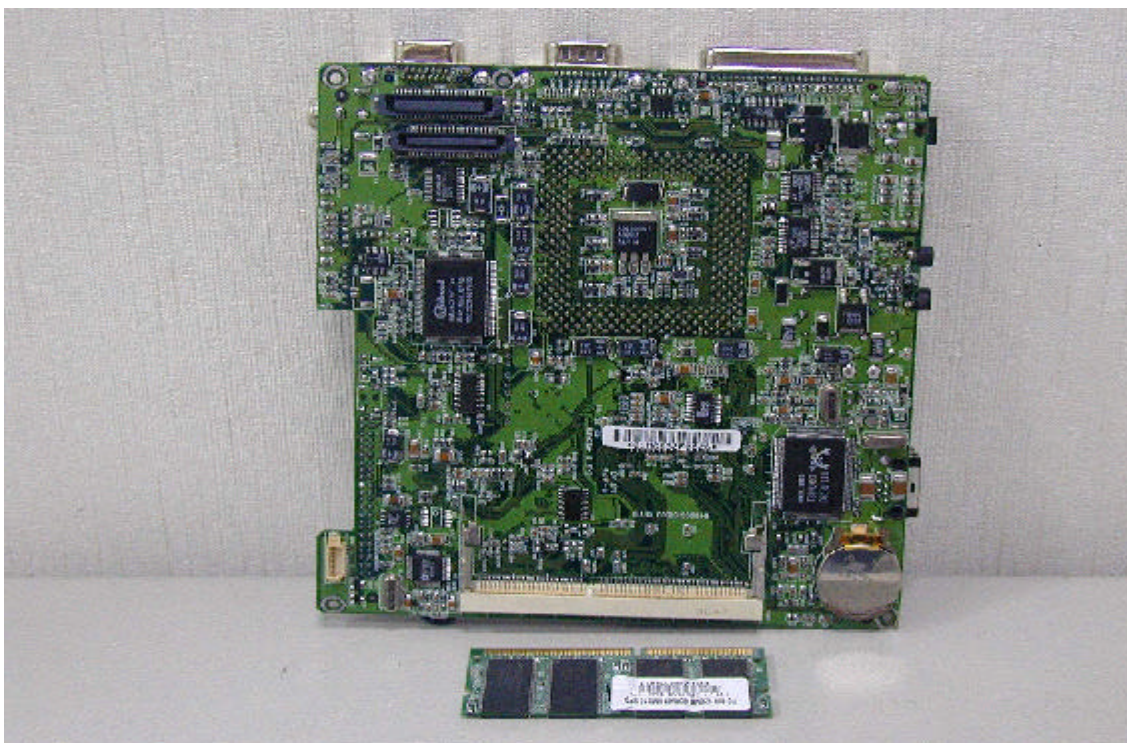
Solder Side View of Main Board
