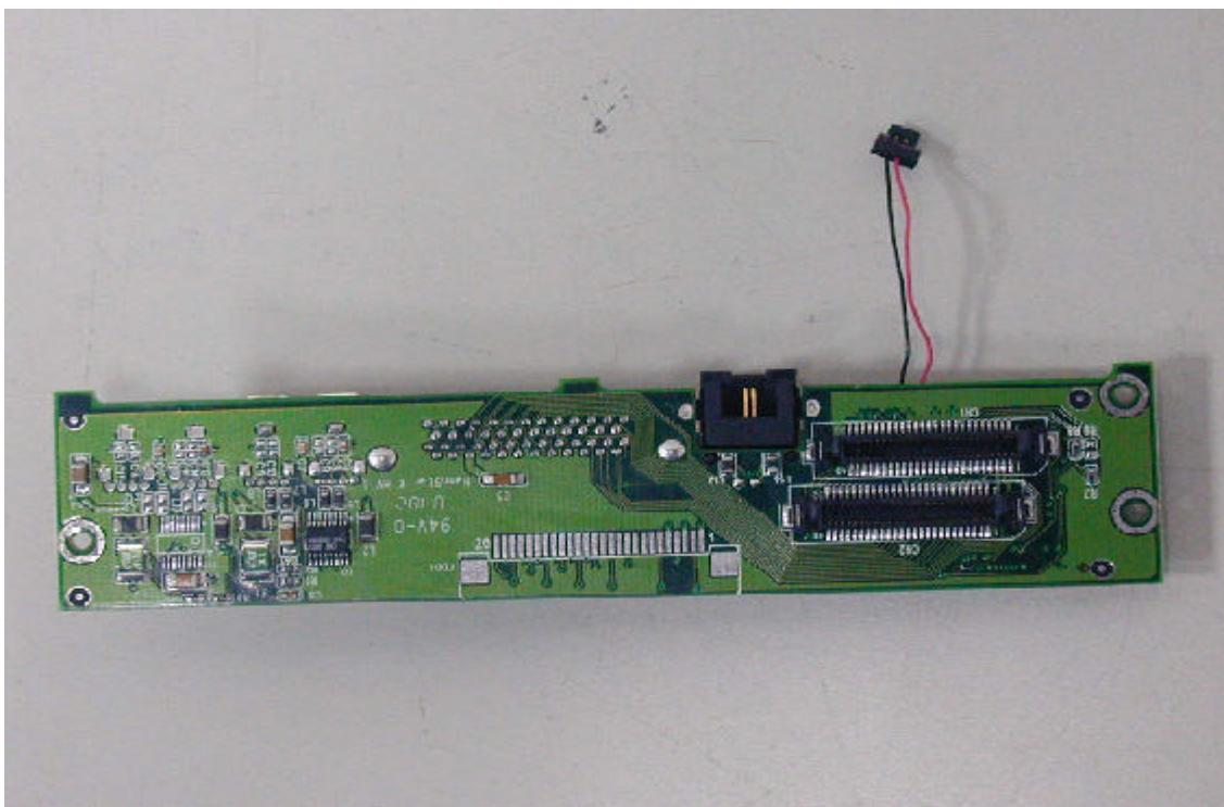
Solder Side View of 1394 Connector
