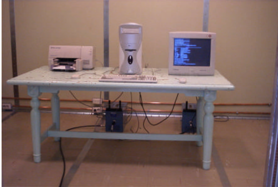
Photograph 2 : Setup for Conducted Emissions
