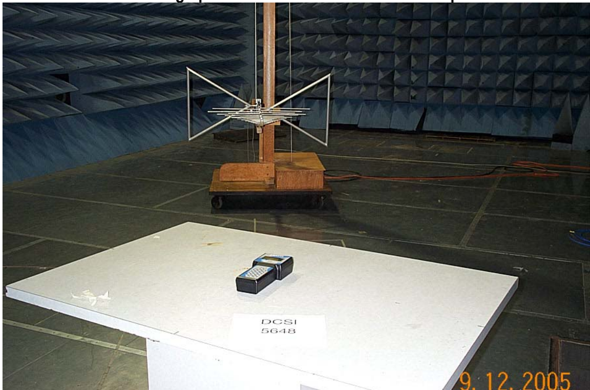
Photograph of Radiated Emissions Test Setup
