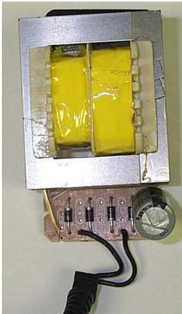
Power Supply Board: Component Side
