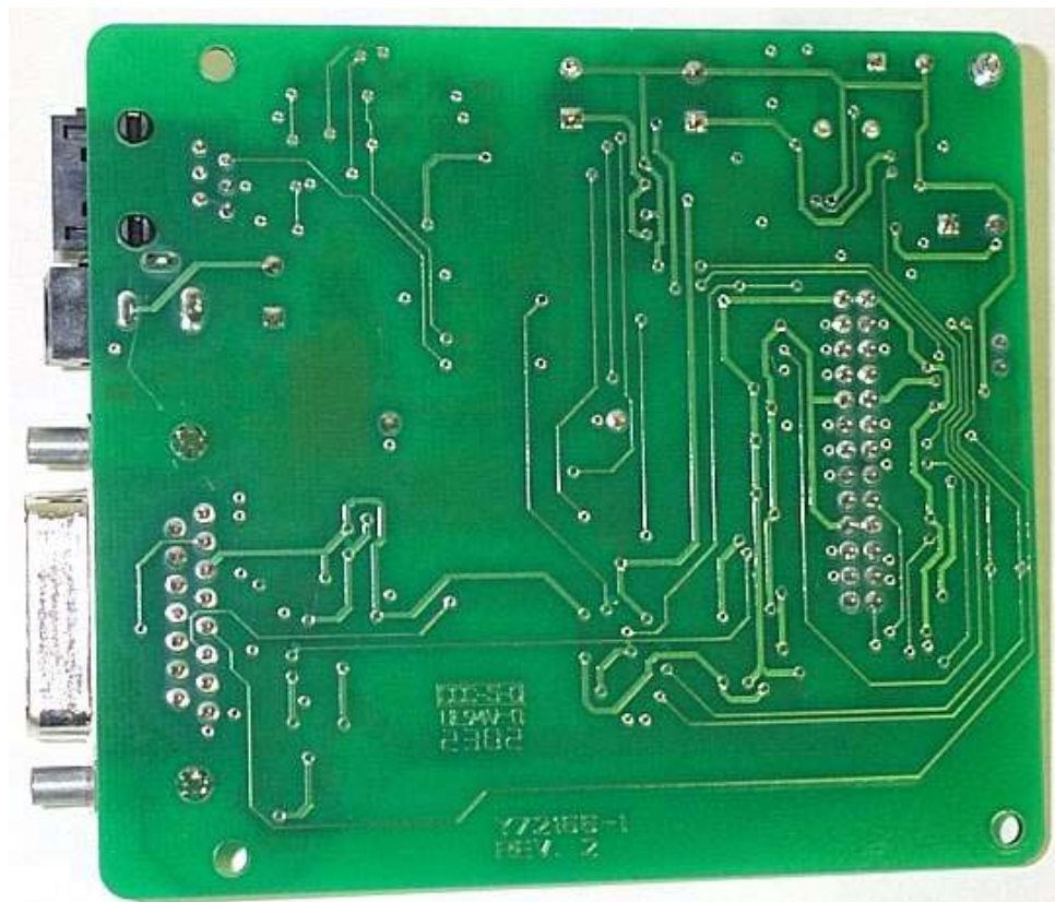
Interface PCB Foil Side
