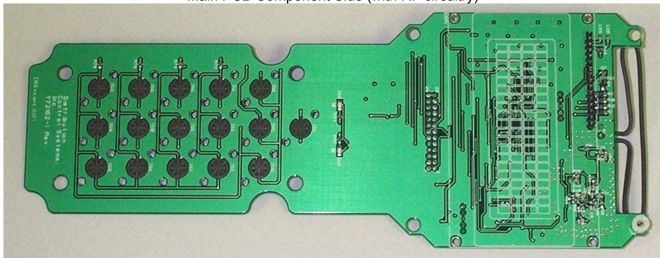
Main PCB Foil Side (with RF circuitry)
