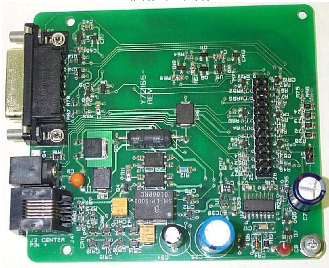
Interface PCB Component Side
