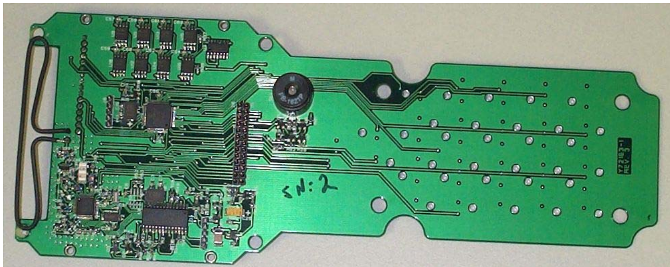
Main PCB Component Side (with RF circuitry)
