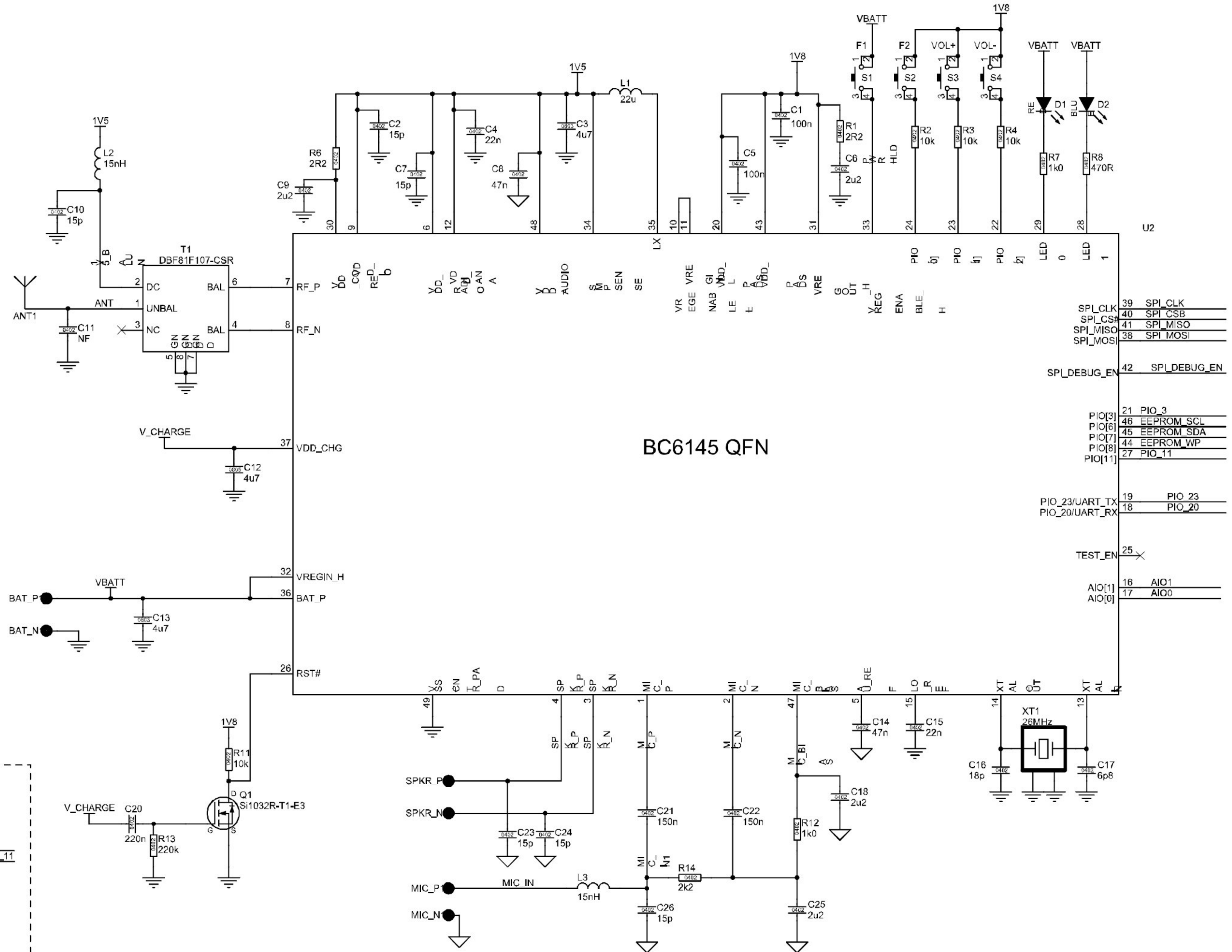
Figure 10.1: Example Application Schematic
