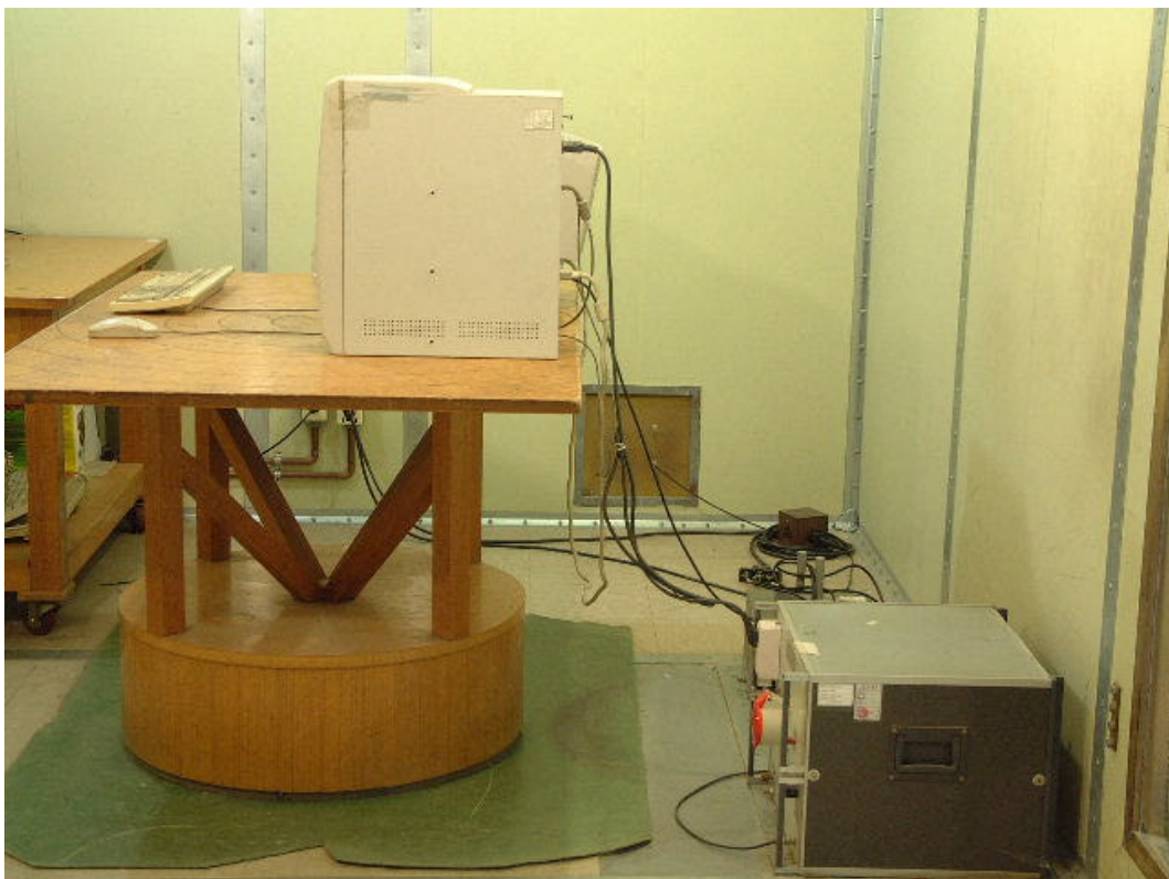
LINE CONDUCTED SETUP PHOTOGRAPH - REAR VIEW
