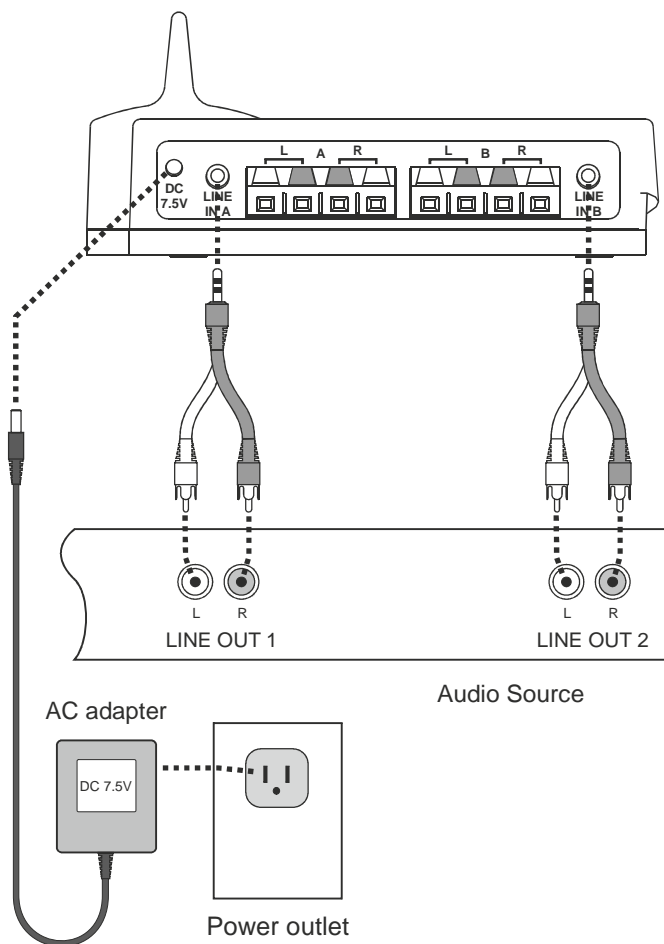
Example 1: Using the transmitter line-level audio inputs
