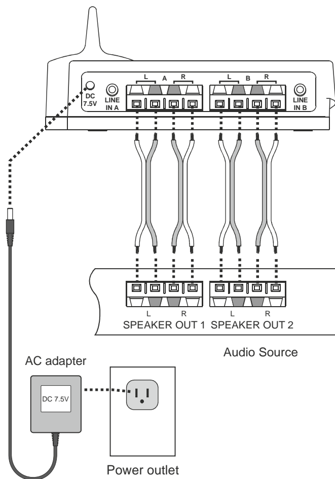
Example 2: Using the transmitter speaker-level audio inputs
