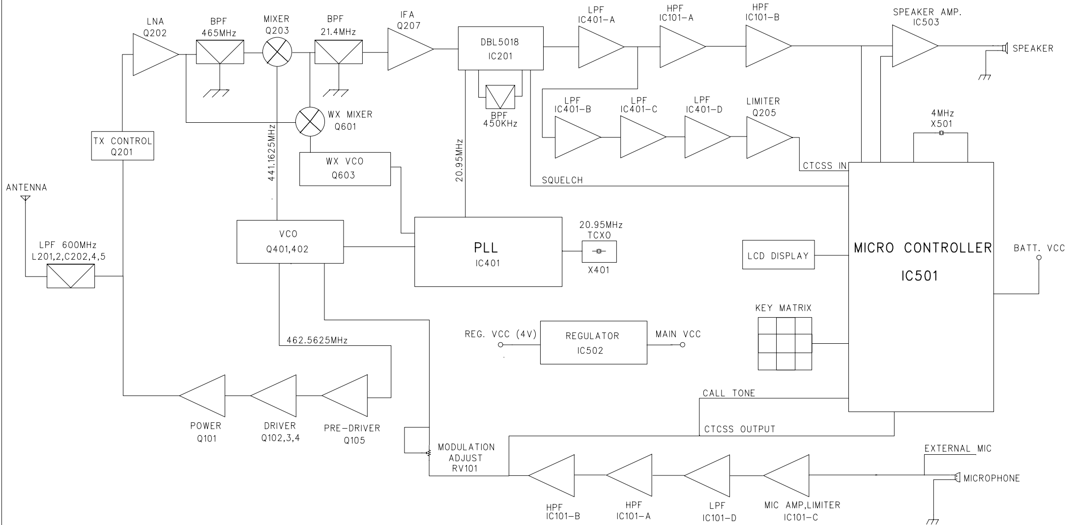
BLOCK DIAGRAM
