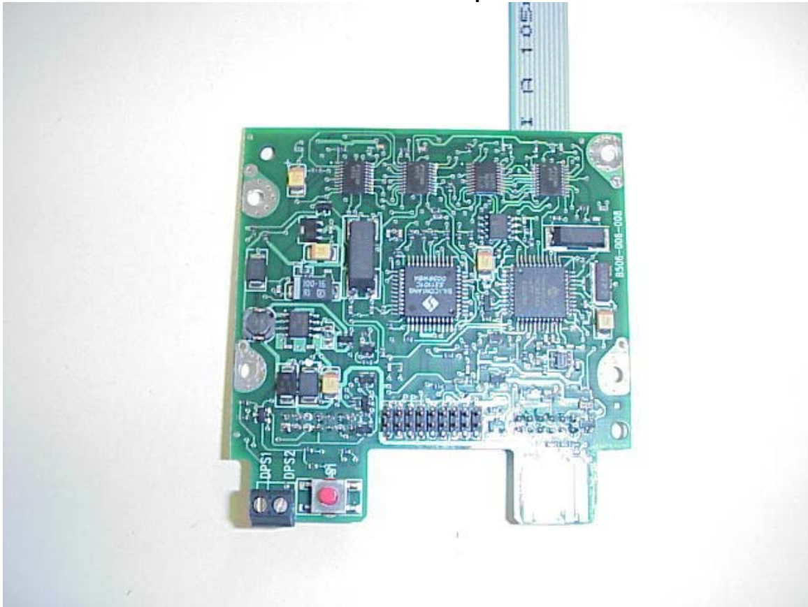
WPR Baseband PCB Component side
