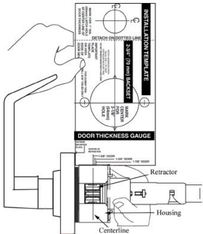
Figure 2-27 – Door Thickness Adjustment
