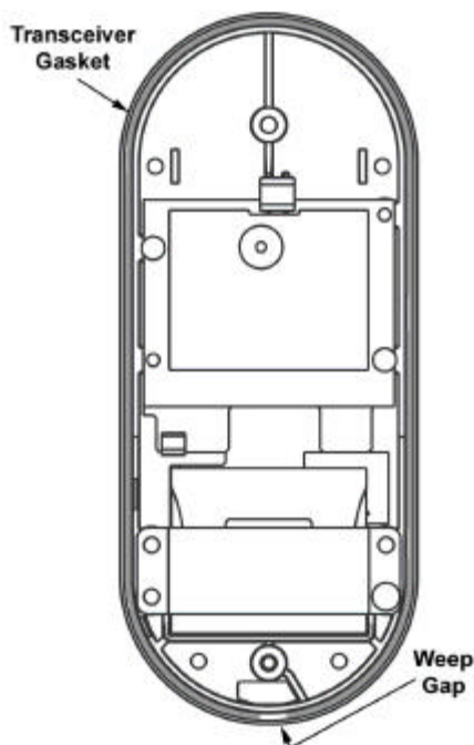
Figure 2-36 – MIRL Transceiver Gasket
