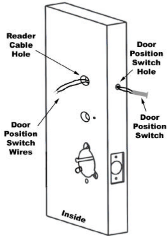
Figure 2-12 – Installing the Door Position Switch
