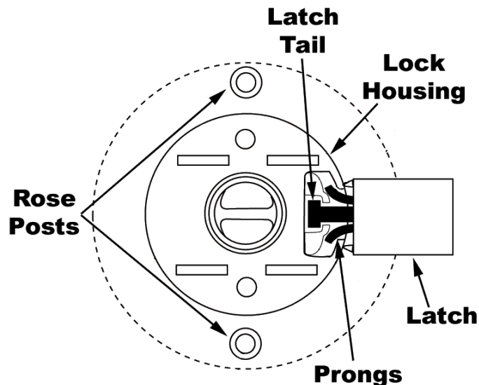
Figure 2-30 – Engaging Retractor & Latch
