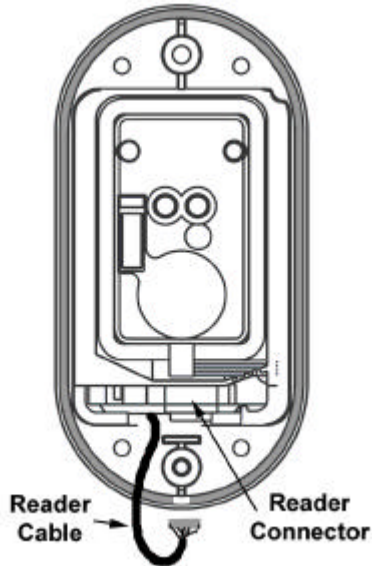
Figure 2-23 – Reader Cable Connection
