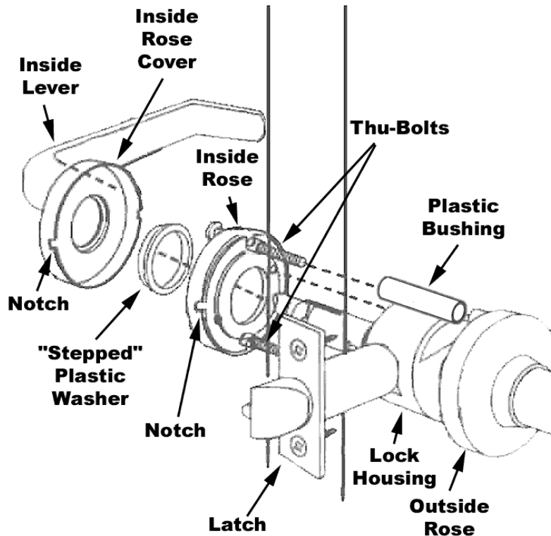
Figure 2-32 – Installing Inside Rose, Thru-Bolts and Cover
