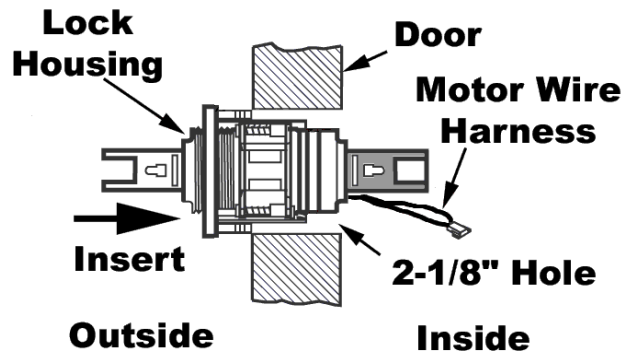
Figure 2-29 – Inserting Lock Housing into the 2-1/8" Hole
