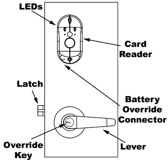
Figure 1-3 – Locked Side of the MIRL
