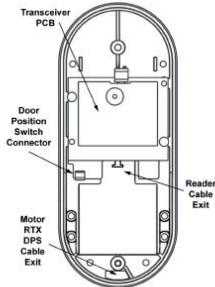
Figure 2-18 – Connecting the Door Position Switch Wires
