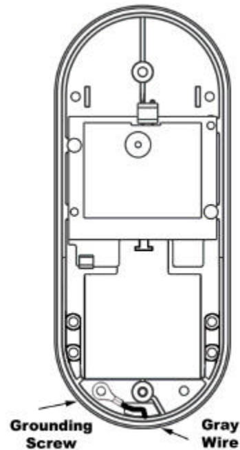
Figure 2-16 – Mounting Transceiver Base Plate Figure 2-17 – Transceiver Grounding Screw
