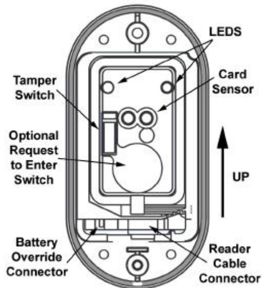
Figure 2-20 – Reader Base Plate Components
