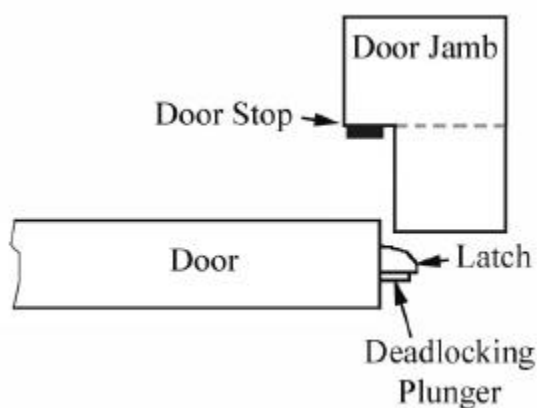
Figure 2-11 – Latch Orientation on Door Edge
