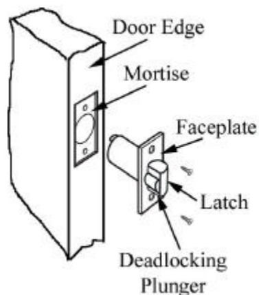
Figure 2-10 – Mortising Latch on Door Edge
