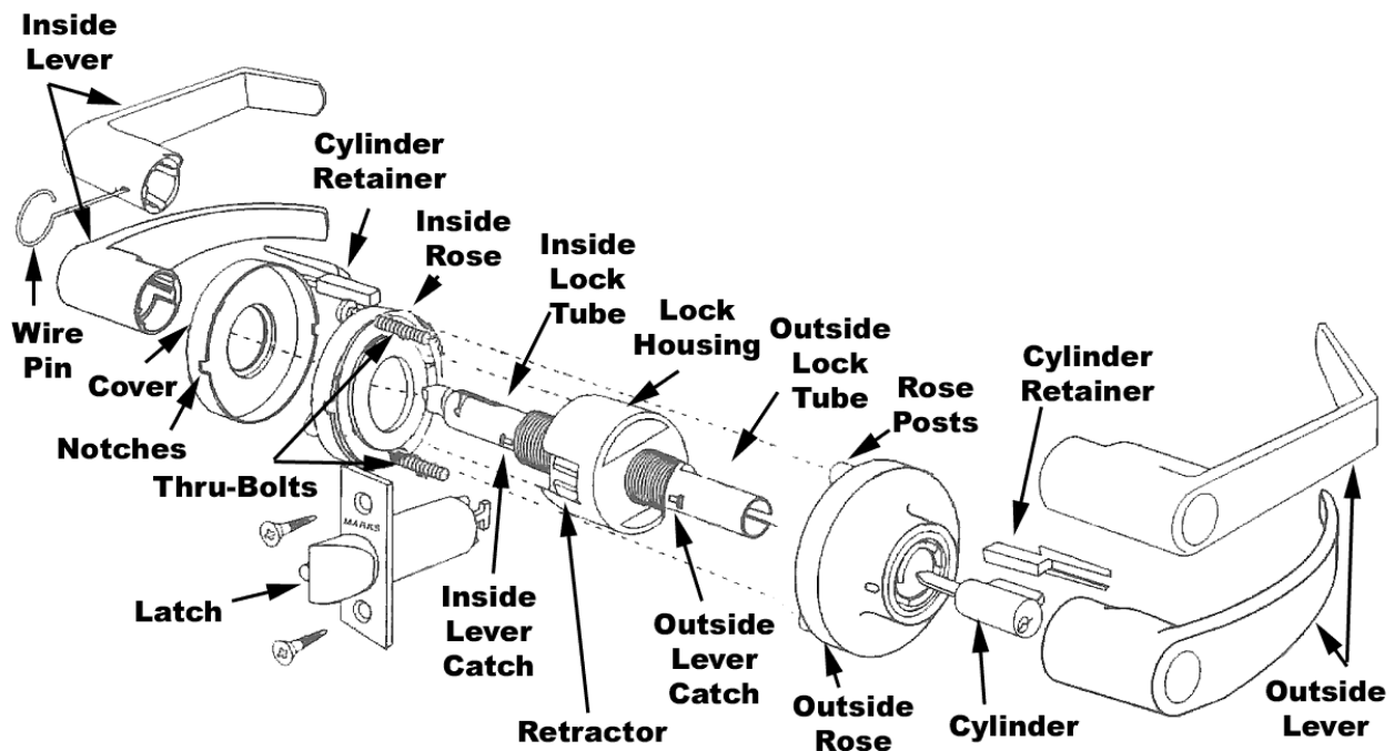
Figure 2-28 – Exploded Lock Hardware
