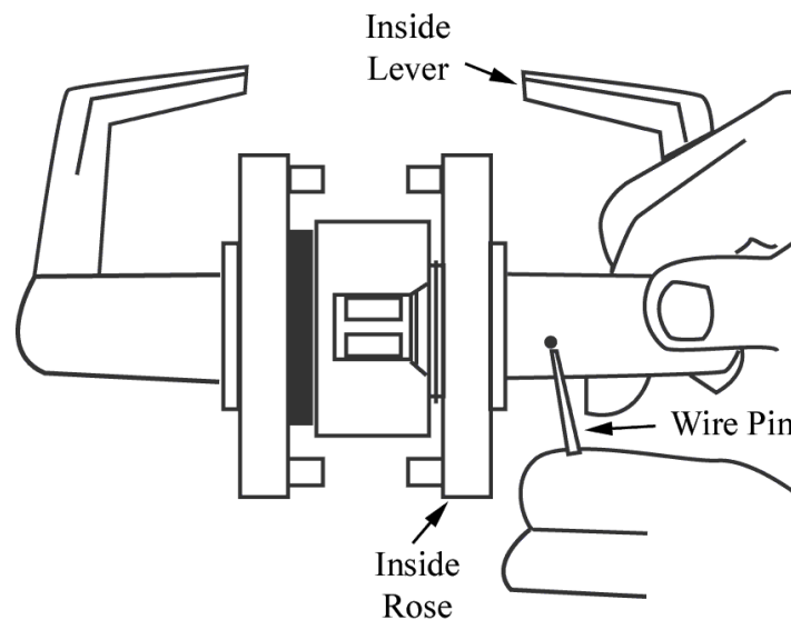
Figure 2-26 – Removing Inside Lever & Inside Rose Assembly
