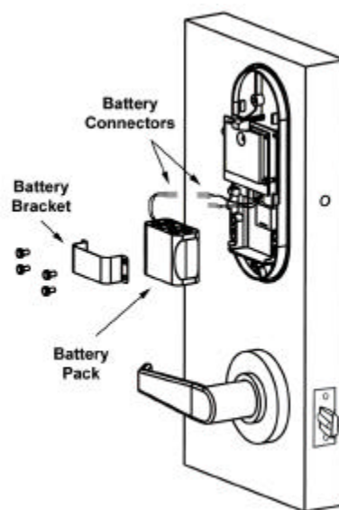
Figure 2-35 – MIRL Battery Pack Installation
