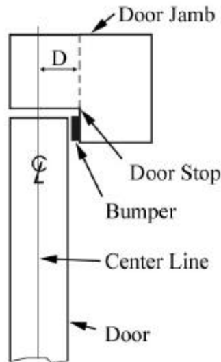
Figure 2-4 – Locating Center Line on Doorjamb (top view)
