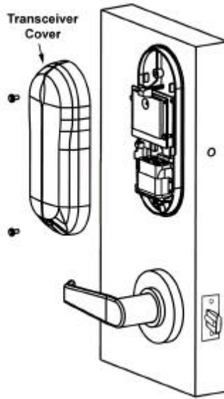
Figure 2-37 – MIRL Transceiver Cover
