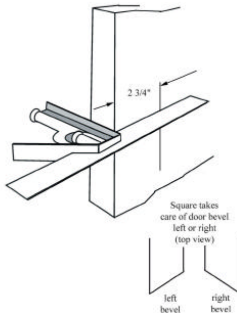
Figure 2-1 – Marking 2 ¾" Setback with Square
