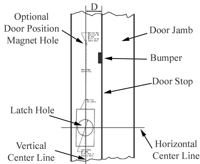
Figure 2-5 – Template, RSTP21, on Doorjamb (side view)
