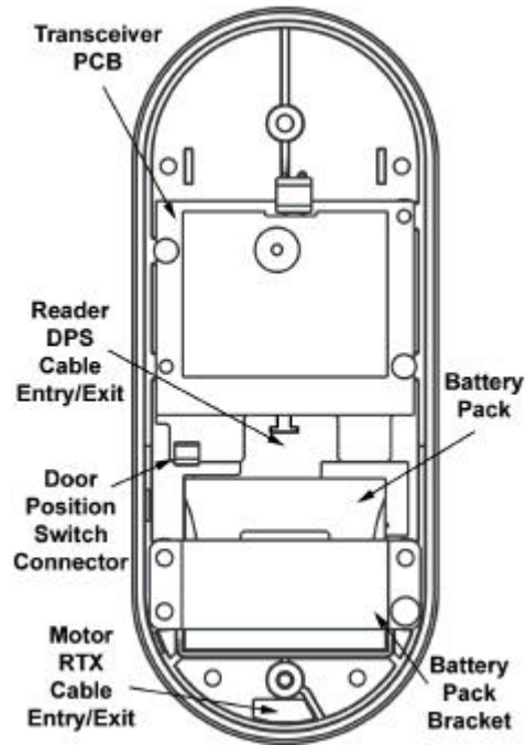
Figure 2-14 –Transceiver Base Plate Components
