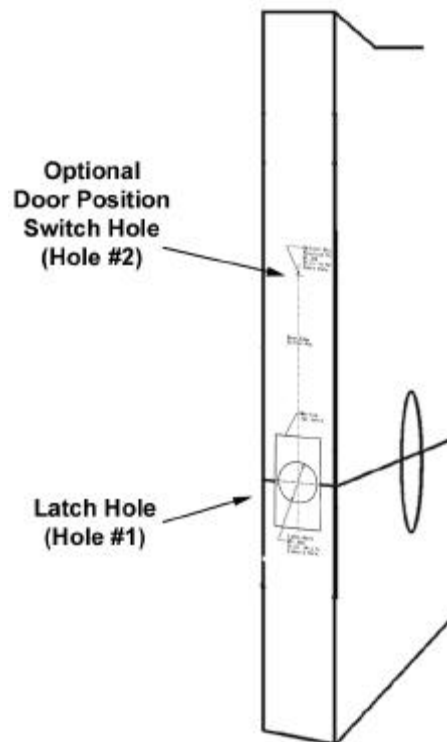
Figure 2-3 – Template RSTP21 on Metal Door Edge
