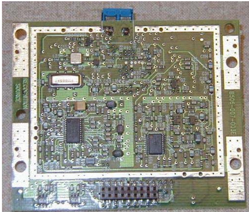
Transceiver without Cover
