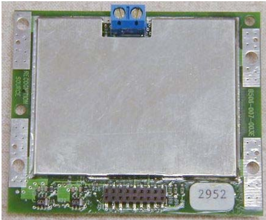
Transceiver with Cover
