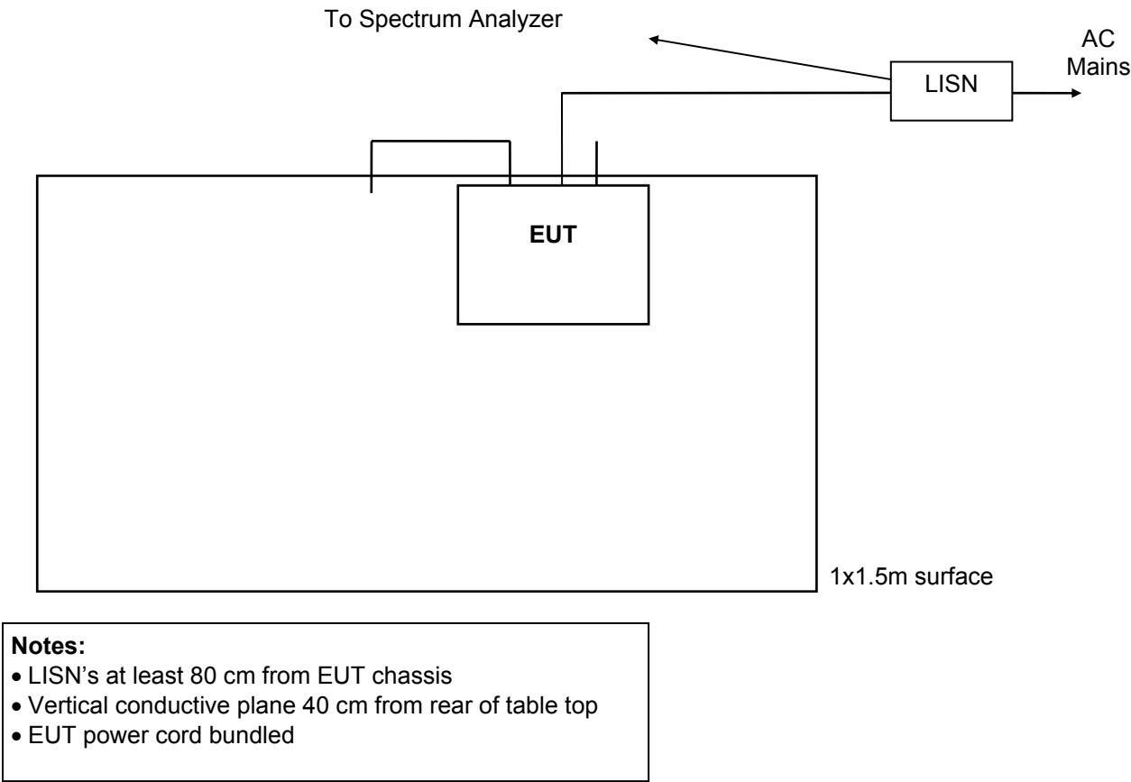
Figure 2. Conducted Emissions Test Setup
