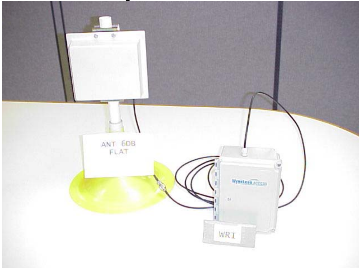
WRI Configuration with 6dB External Antenna
