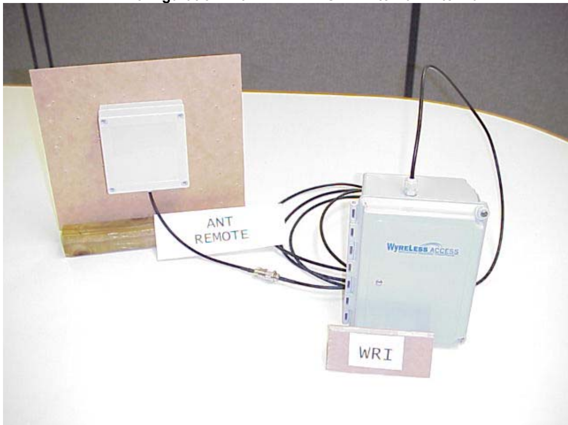
WRI Configuration with ANT-REMOTE External Antenna
