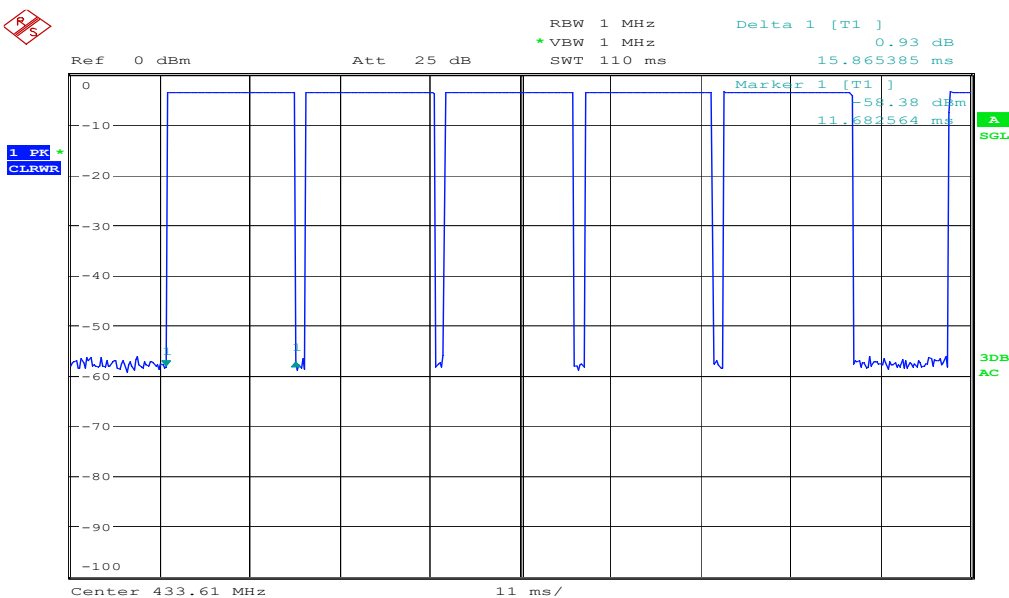
Detail of a single pulse train
