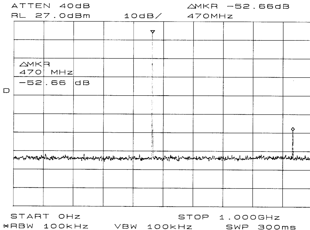
Figure six Emissions at Antenna Terminal low power.
