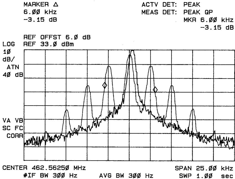
Figure four Occupied Band Width with no CTCSS tone.
