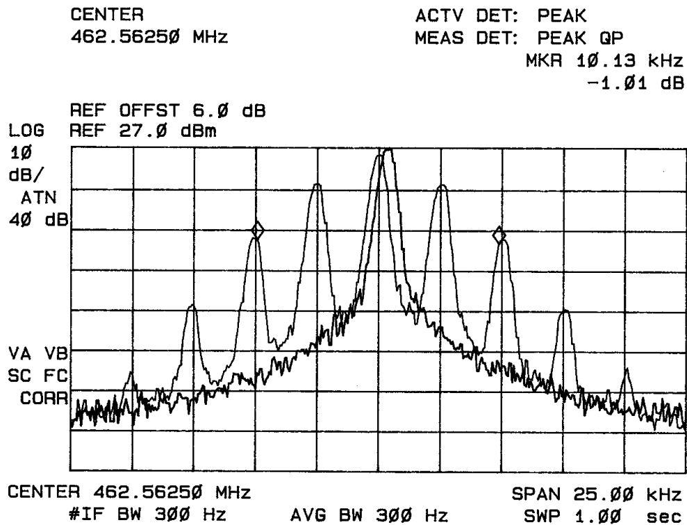
Figure five Occupied Band Width with CTCSS tone.
