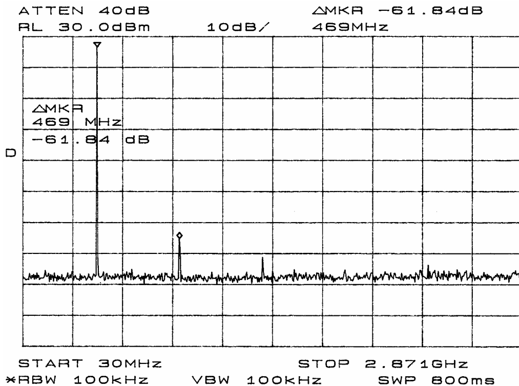
Figure 7: Emissions at Antenna Terminal (467.55 MHz)
