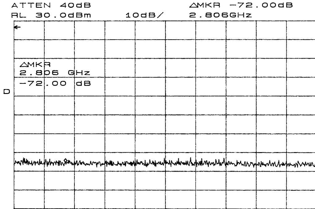
Figure 7A: Emissions at Antenna Terminal (467.55 MHz)
