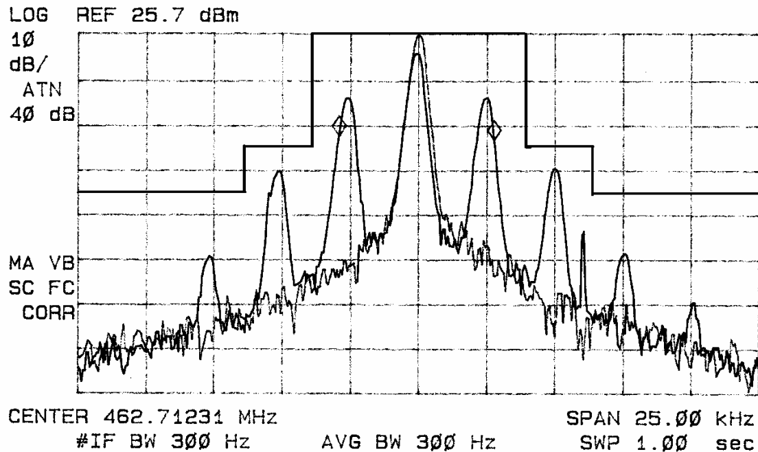
Figure four Occupied Band Width. Data taken with 6dB attenuation at output of 1.5 Watt (31.7 dBm) transmitter.
