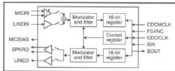
GCT-D430 CODEC Block Diagram
