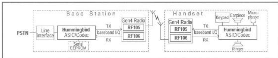
GCT-D430 Spread Spectrum Telephone System Architecture
