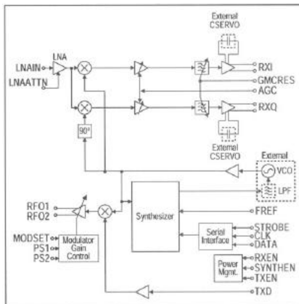
GCT-D430 RF Block Diagram
