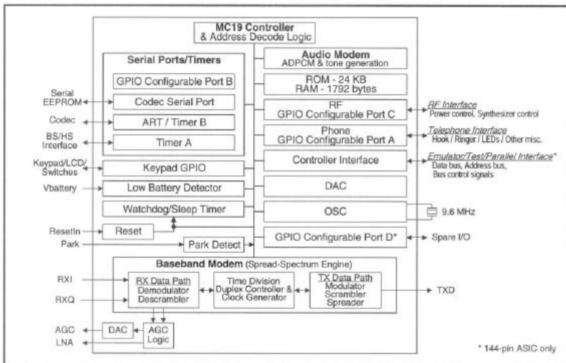
GCT-D430 ASIC Block Diagram
