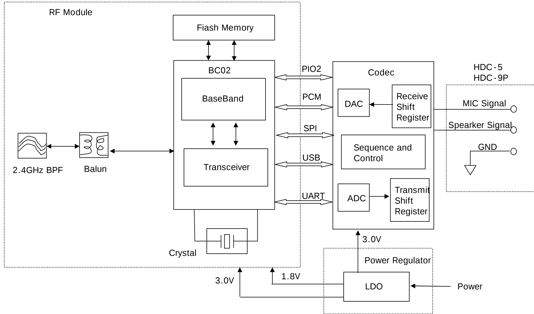
GBH-200A (Audiogate) Block Diagram
