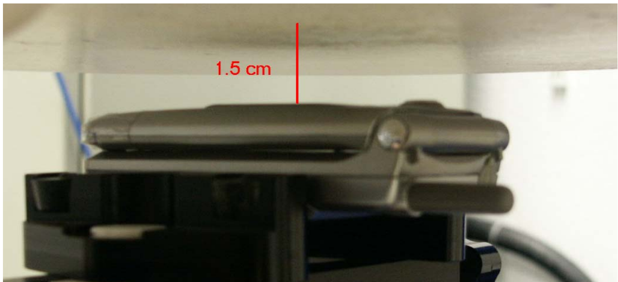
Fig. 20: Body worn configuration with 1.5 cm distance (Antenna towards the ground; GPRS Class 10).
