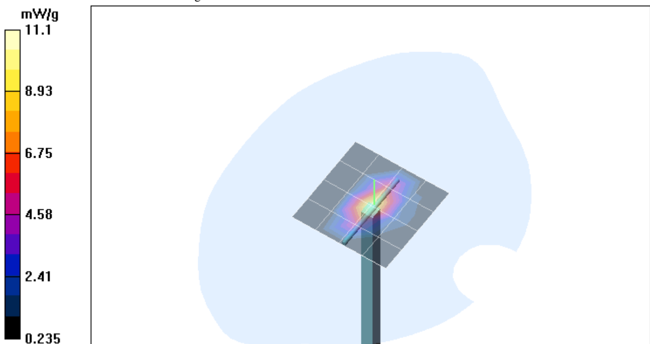
Fig. 11: Validation measurement 1900 MHz body (December 10, 2003), coarse grid. Ambient Temperature: 20.2° C, Liquid Temperature: 19.5° C.
