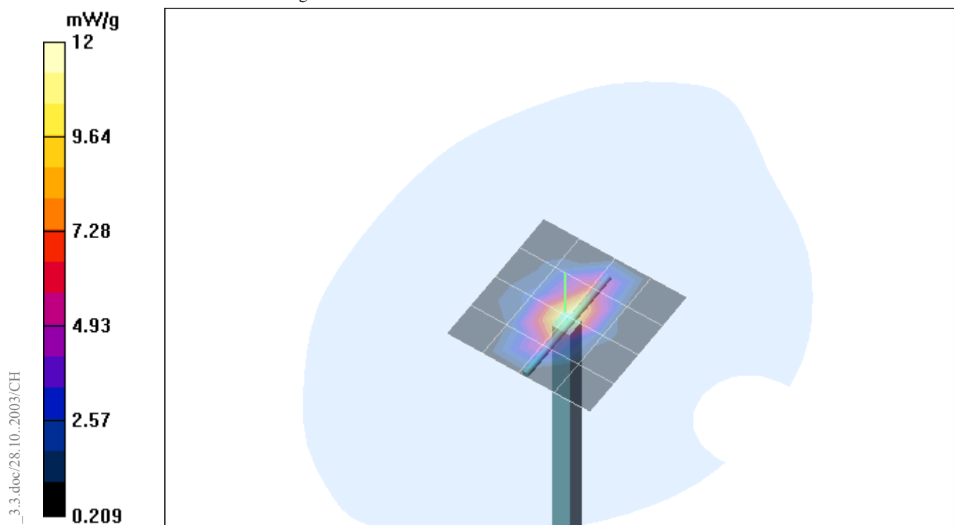
Fig. 10: Validation measurement 1900 MHz Head (December 01, 2003), coarse grid. Ambient Temperature: 20.5° C, Liquid Temperature: 19.4° C.
