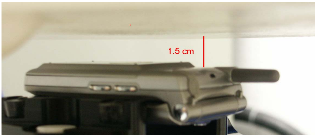
Fig. 19: Body worn configuration with 1.5 cm distance (Antenna towards the phantom; GPRS Class 10 and GSM mode).
