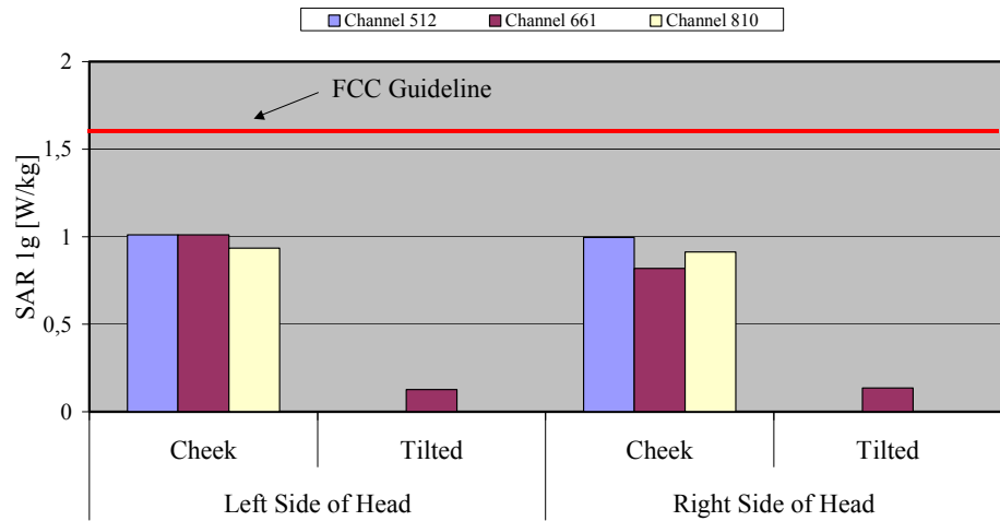
Fig. 8: The measured head phantom SAR values for the Mirae MGH 900 for PCS 1900 in comparison to the FCC exposure limit.
