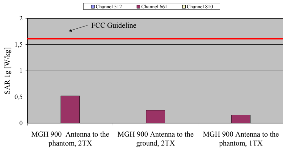
Fig. 9: The measured SAR values in body-worn configuration for the Mirae MGH 900 for PCS 1900 in comparison to the FCC exposure limit.
