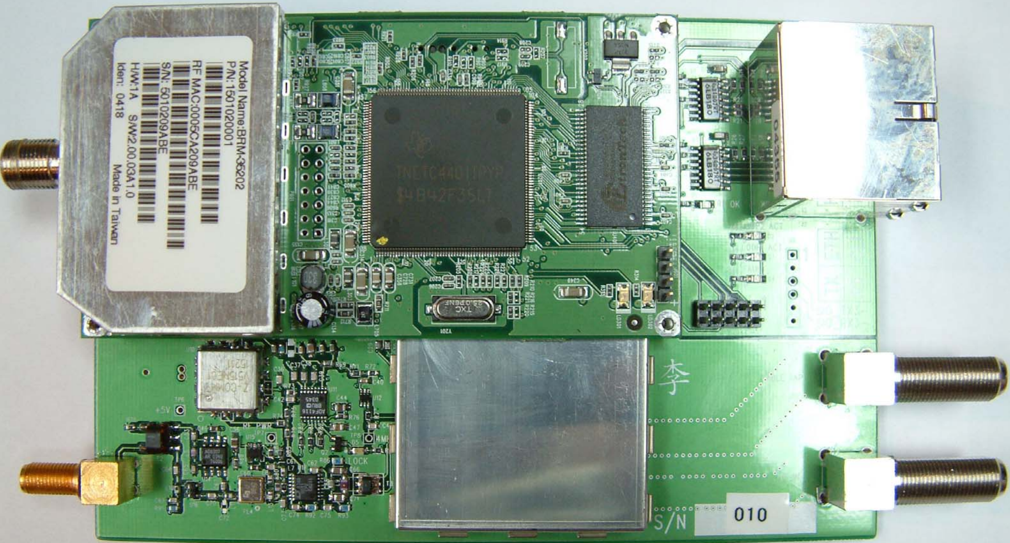
AX300 WITH TRANSPONDER MODULE
