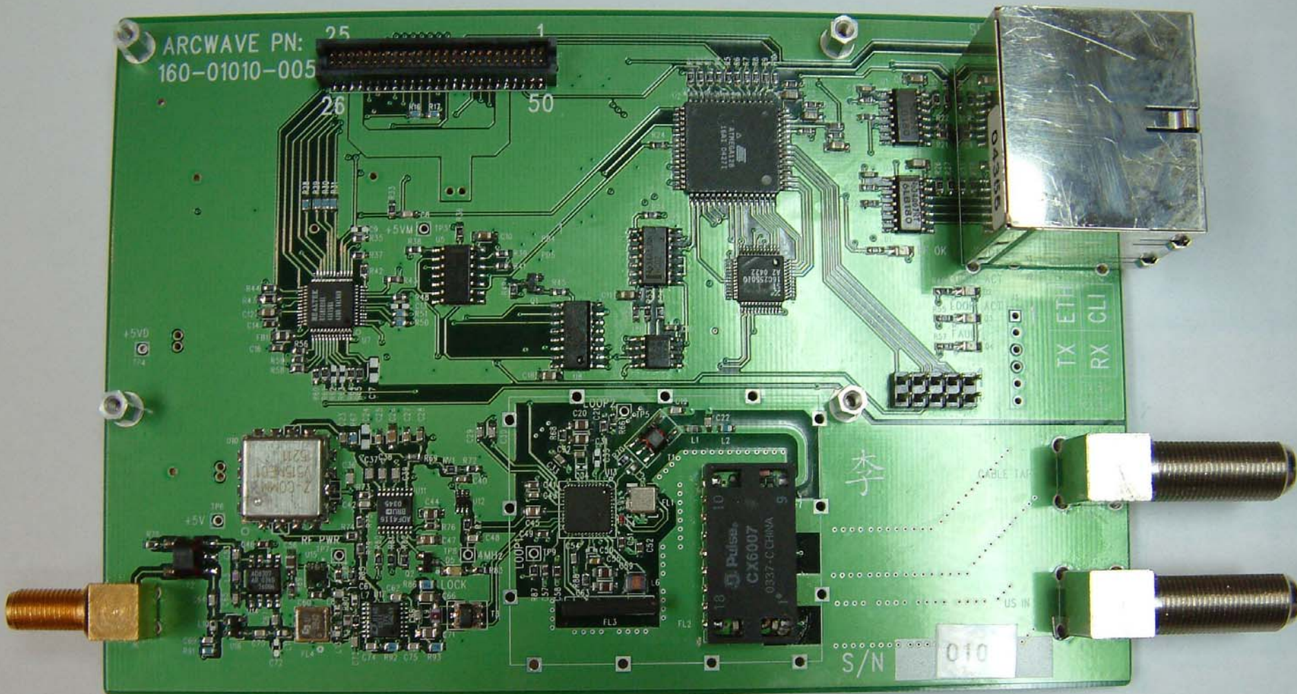
AX300 DOWNSTREAM MODULE
