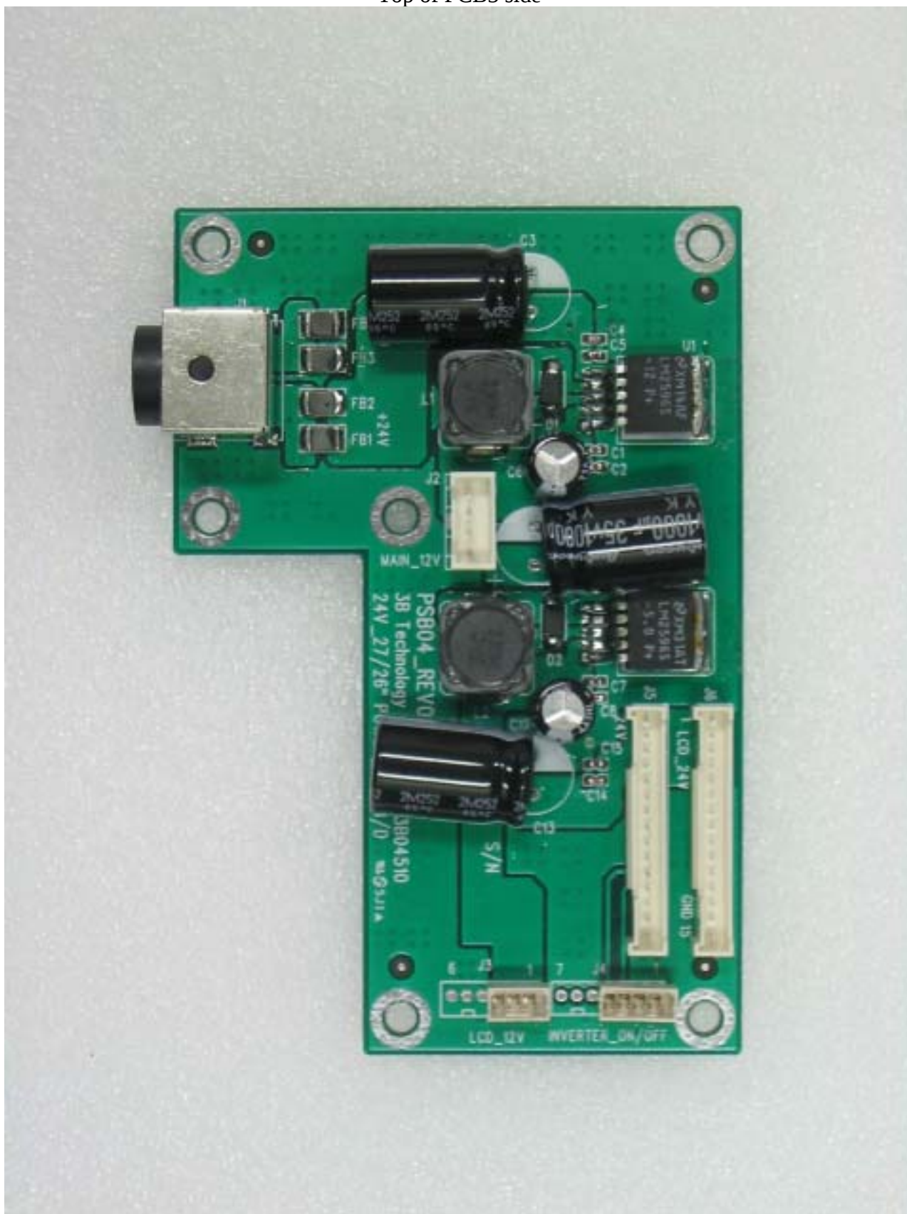
Top of PCB3 side
