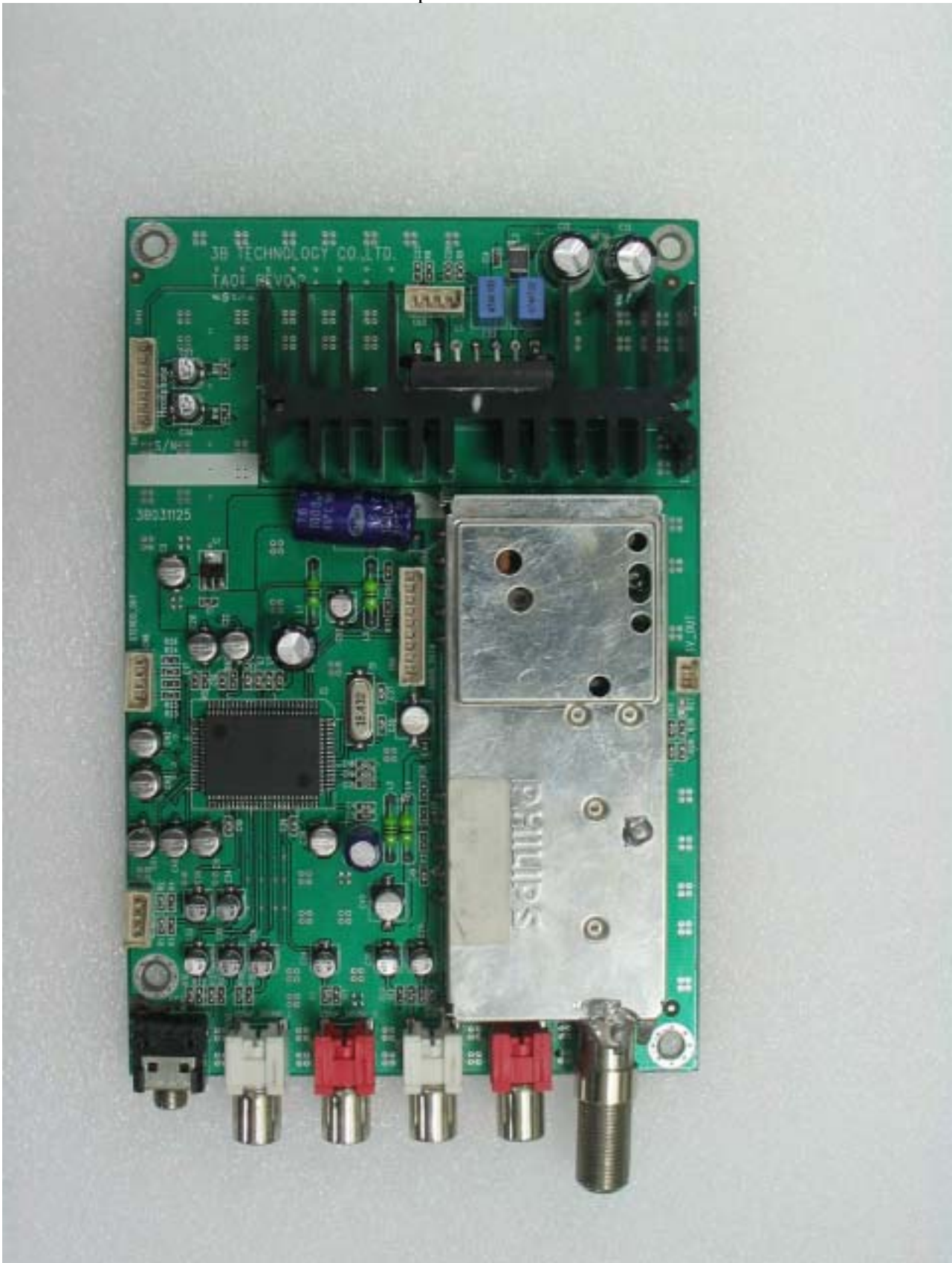
Top of PCB6 side
