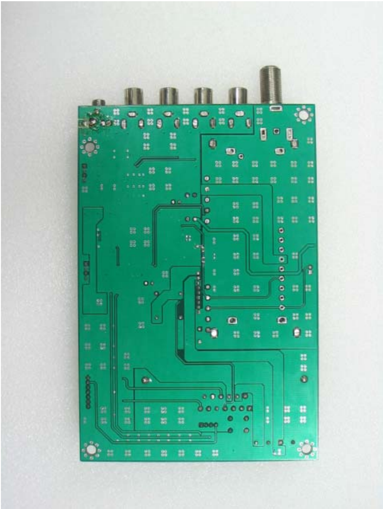
Bottom of PCB6 side
