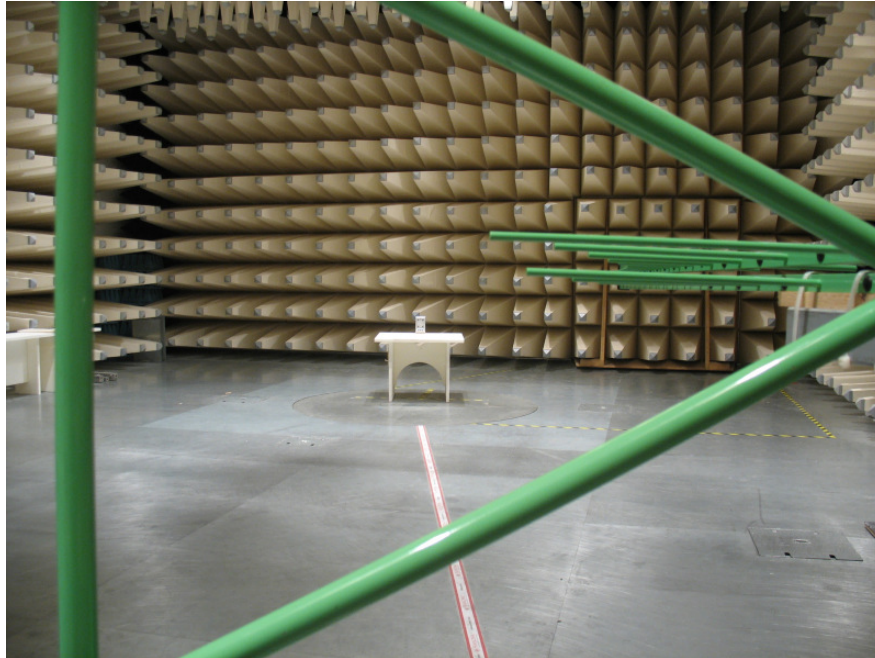
Photo 3 (Radiated Emissions):
