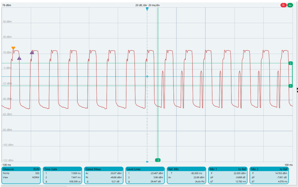
Figure 3-2 Measured 900 MHz Radio Duty Cycle
