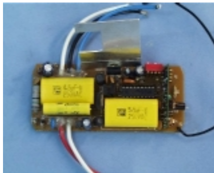
Internal Photo – 2
