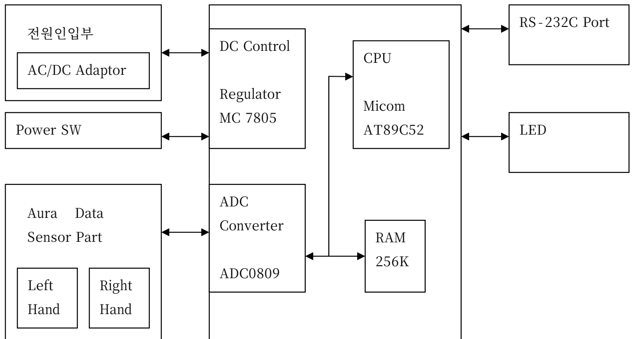
AuraCom Block Diagram
