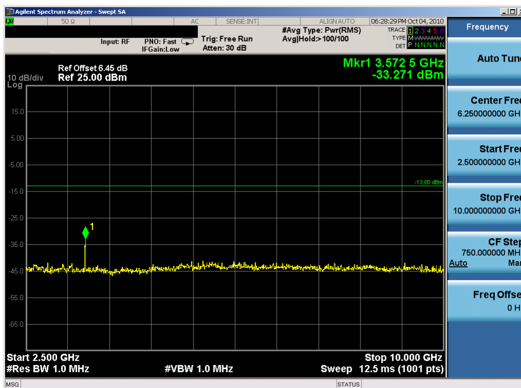
Plot 7-21. Conducted Spurious Plot (64QAM, Tx=713MHz)
