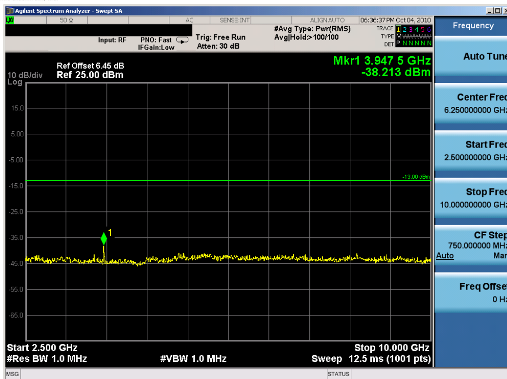
Plot 7-59. Conducted Spurious Plot (64QAM, Tx=790.5MHz)
