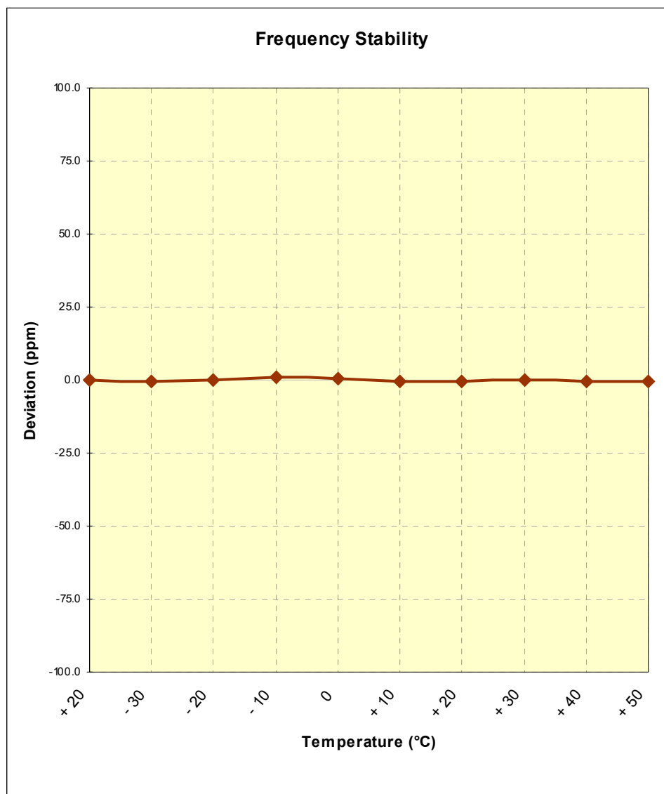
Figure 6-7. Frequency Stability Graph (TD-CDMA Mode Tx=785.5MHz)
