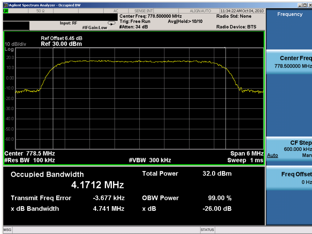
Plot 7-30. Occupied Bandwidth Plot (64QAM, Tx=778.5MHz)
