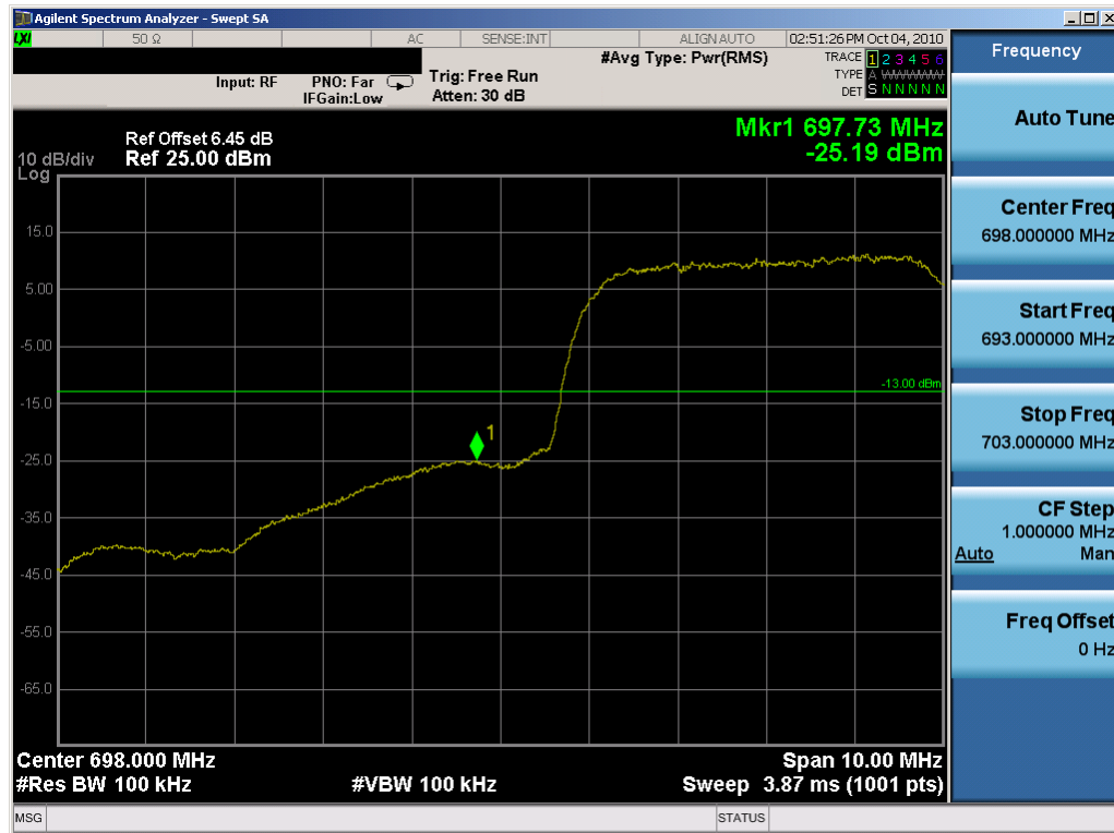
Plot 7-1. Lower Band Edge Plot (QPSK, Tx=701MHz)
