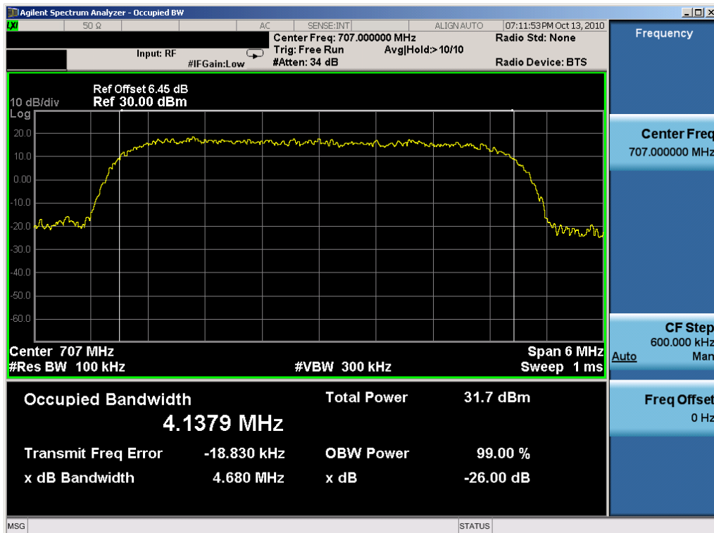
Plot 7-11. Occupied Bandwidth Plot (16QAM, Tx=707MHz)
