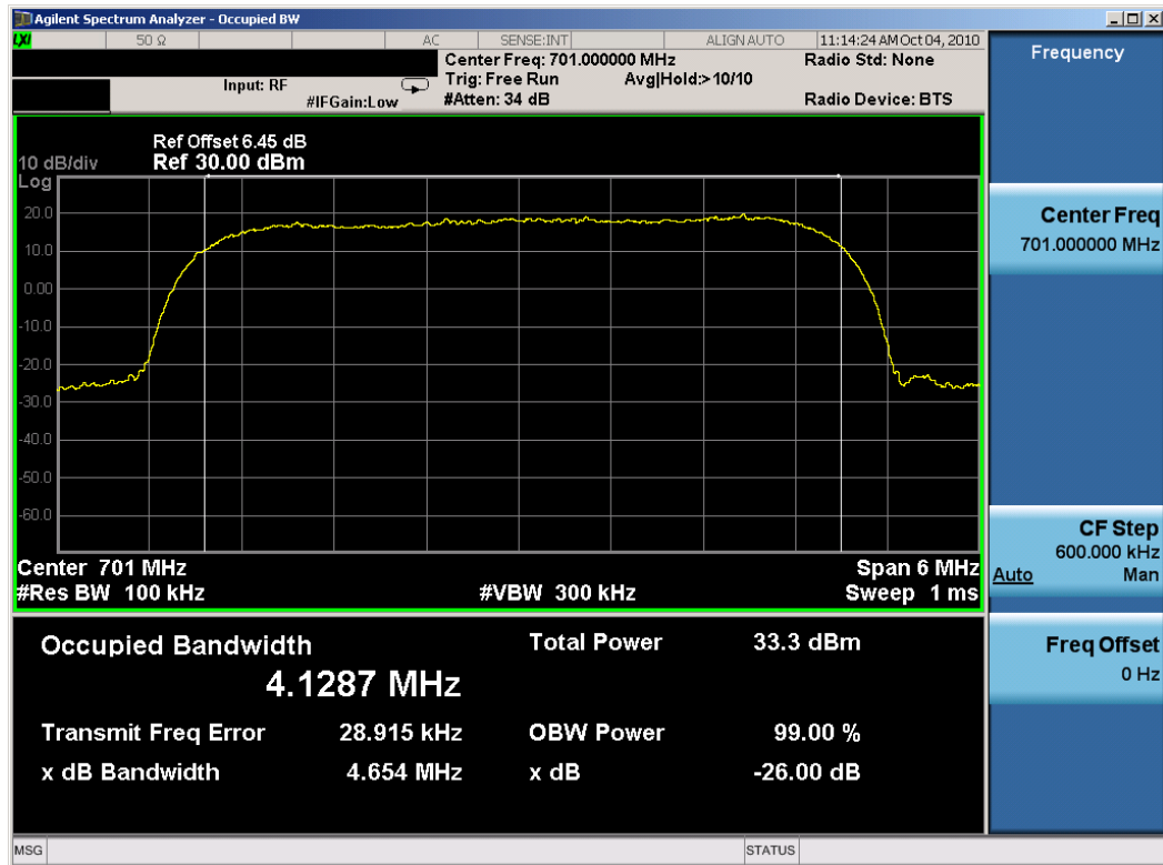
Plot 7-7. Occupied Bandwidth Plot (QPSK, Tx=701MHz)
