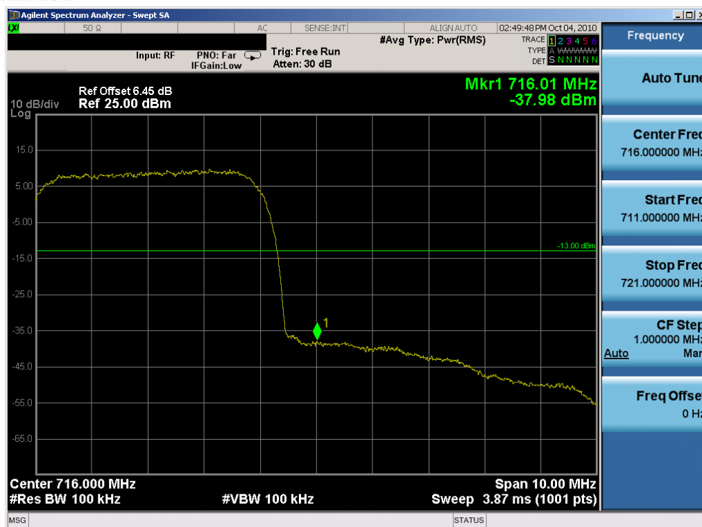
Plot 7-4. Upper Band Edge Plot (QPSK, Tx=713MHz)
