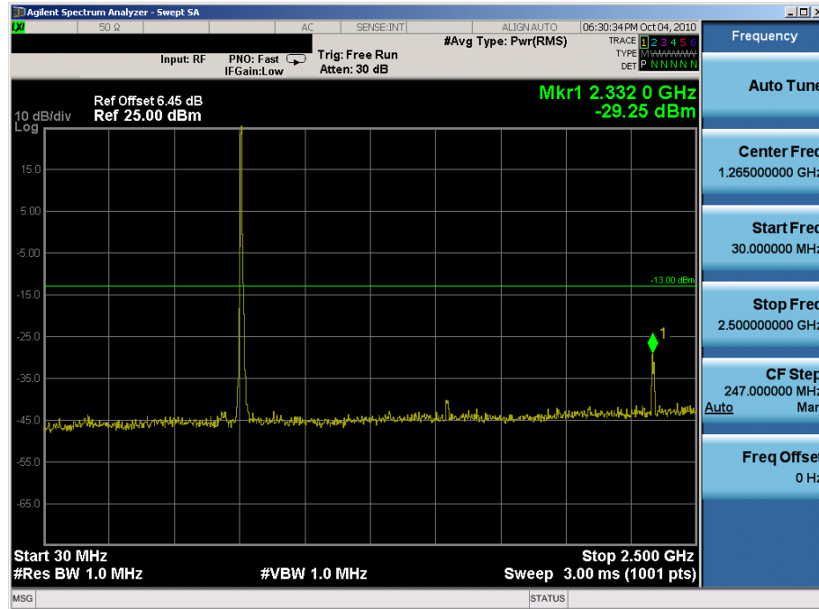
Plot 7-37. Conducted Spurious Plot (64QAM, Tx=778.5MHz)
