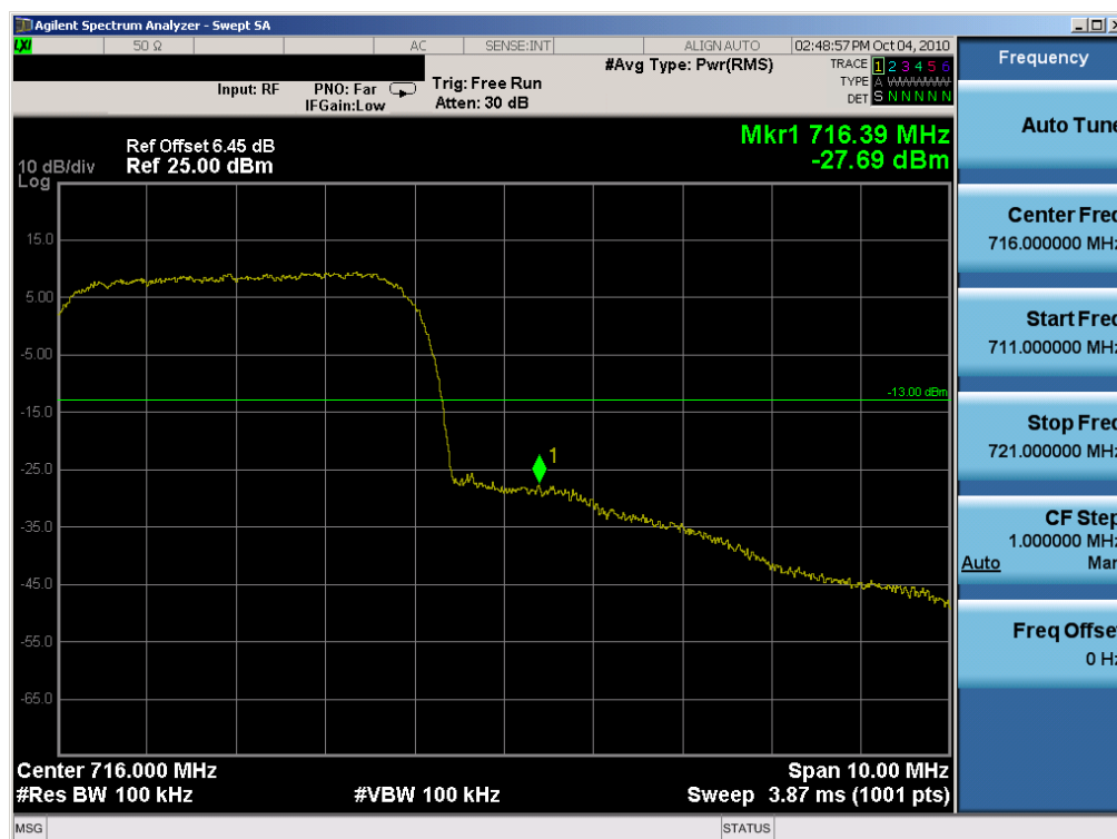
Plot 7-5. Upper Band Edge Plot (16QAM, Tx=713MHz)
