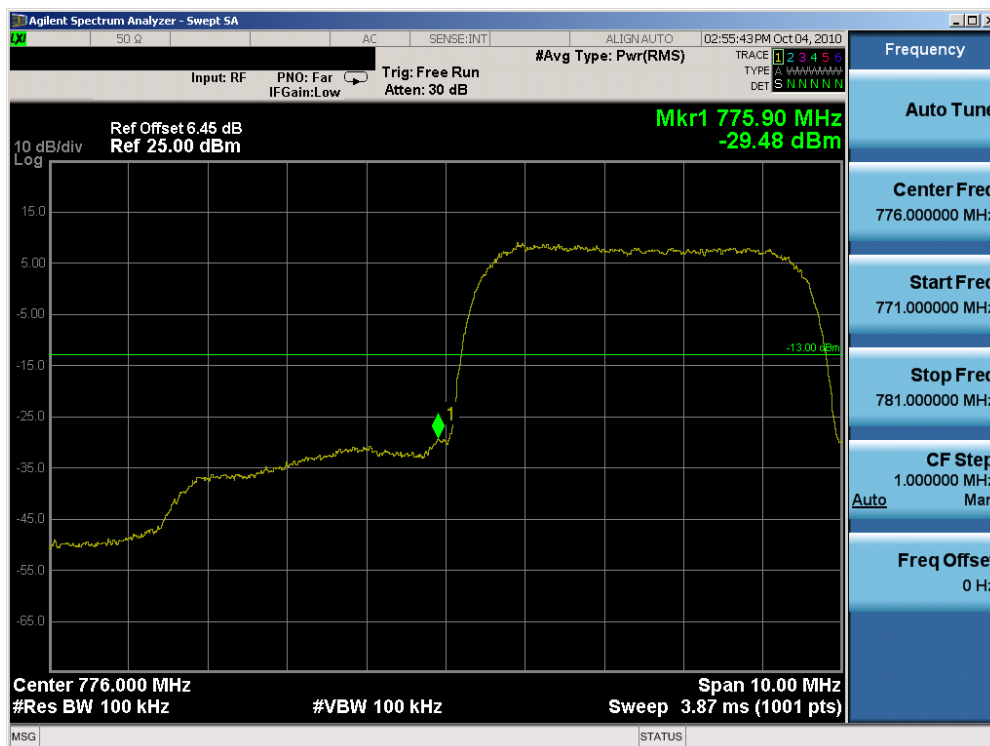
Plot 7-22. Lower Band Edge Plot (QPSK, Tx=778.5MHz)
