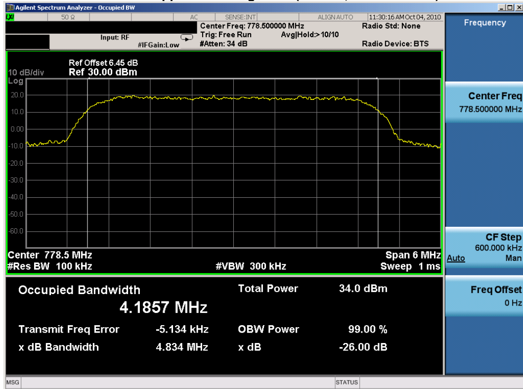
Plot 7-28. Occupied Bandwidth Plot (QPSK, Tx=778.5MHz)
