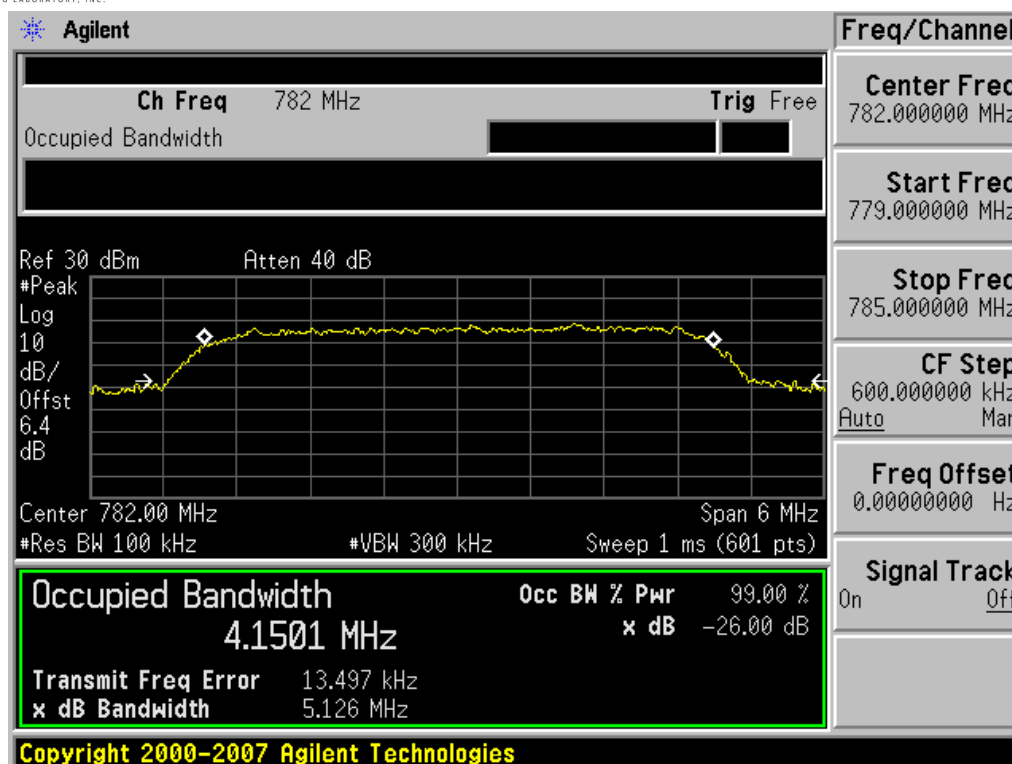
Plot 7-33. Occupied Bandwidth Plot (64QAM, Tx=782 MHz)
