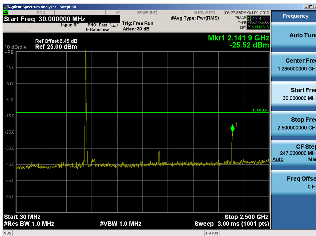
Plot 7-20. Conducted Spurious Plot (64QAM, Tx=713MHz)
