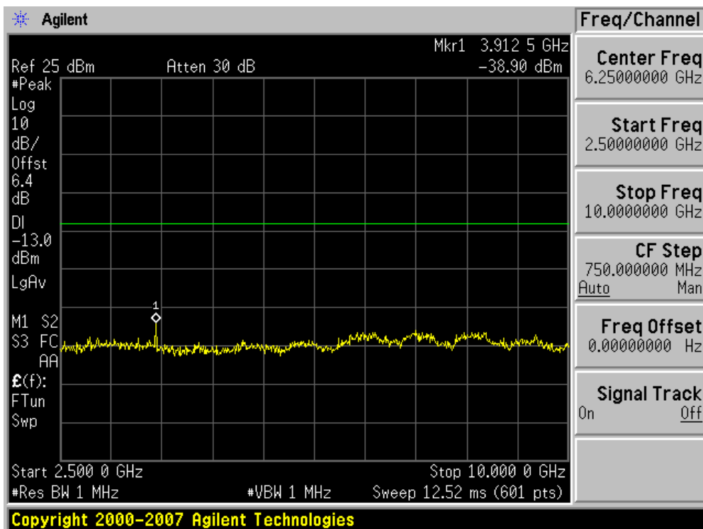
Plot 7-40. Conducted Spurious Plot (64QAM, Tx=782MHz)
