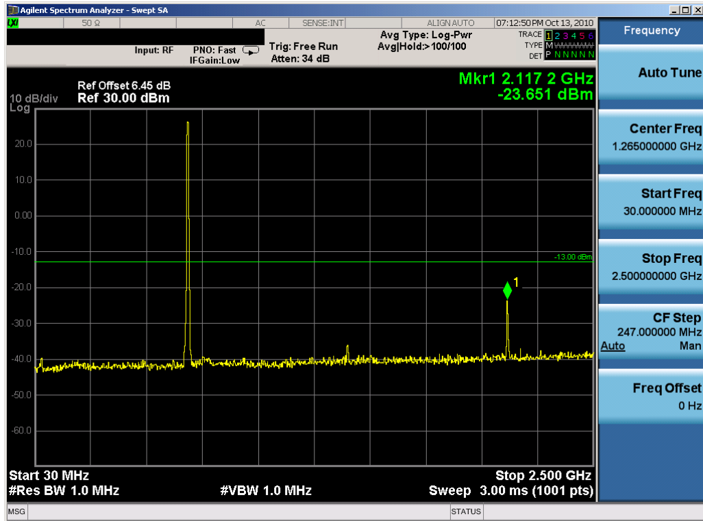
Plot 7-18. Conducted Spurious Plot (64QAM, Tx=707MHz)
