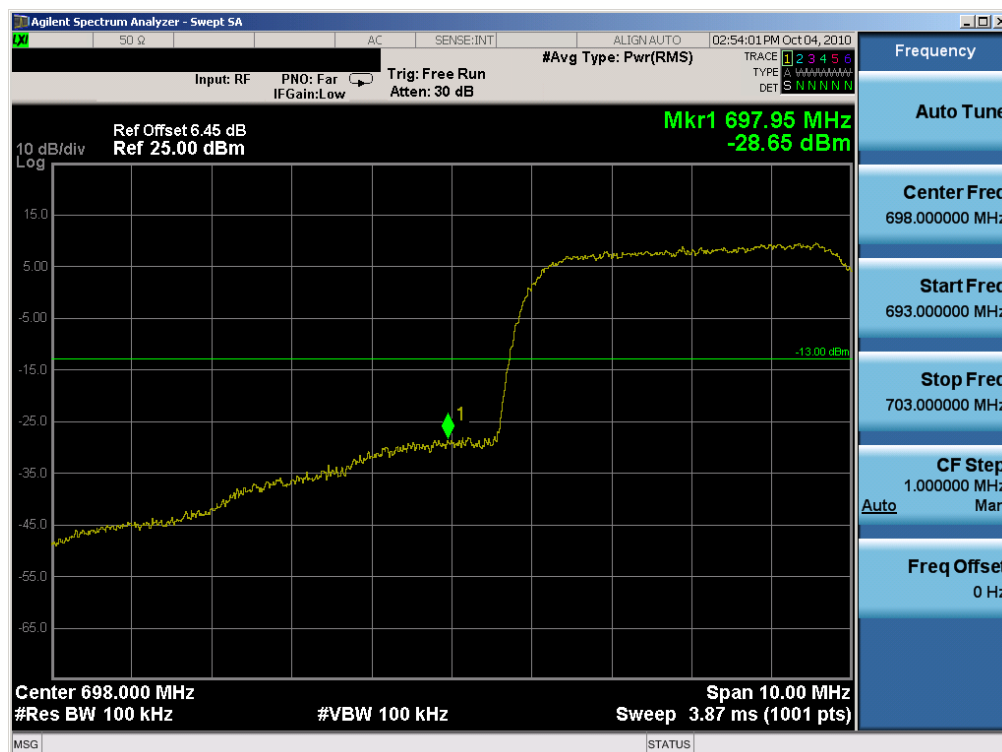
Plot 7-3. Lower Band Edge Plot (64QAM, Tx=701MHz)
