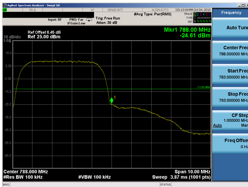
Plot 7-25. Upper Band Edge Plot (QPSK, Tx=785.5MHz)
