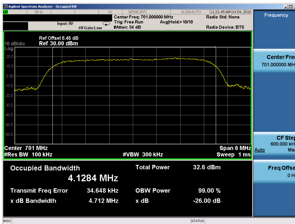
Plot 7-9. Occupied Bandwidth Plot (64QAM, Tx=701MHz)
