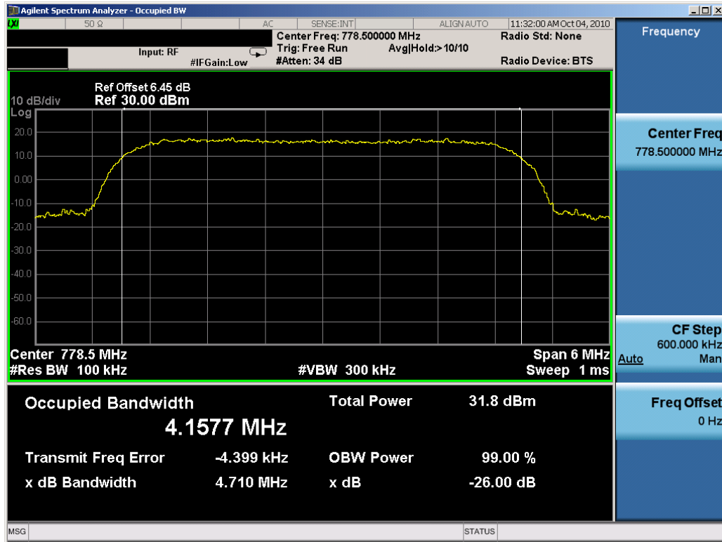
Plot 7-29. Occupied Bandwidth Plot (16QAM, Tx=778.5MHz)
