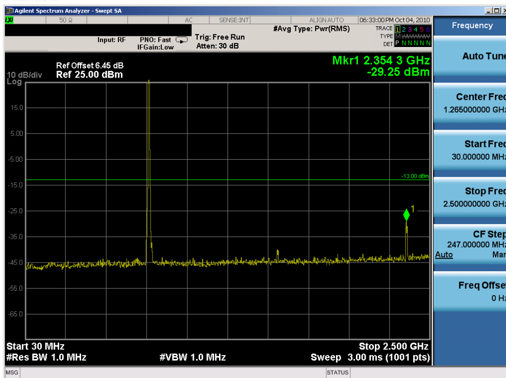
Plot 7-41. Conducted Spurious Plot (64QAM, Tx=785.5MHz)
