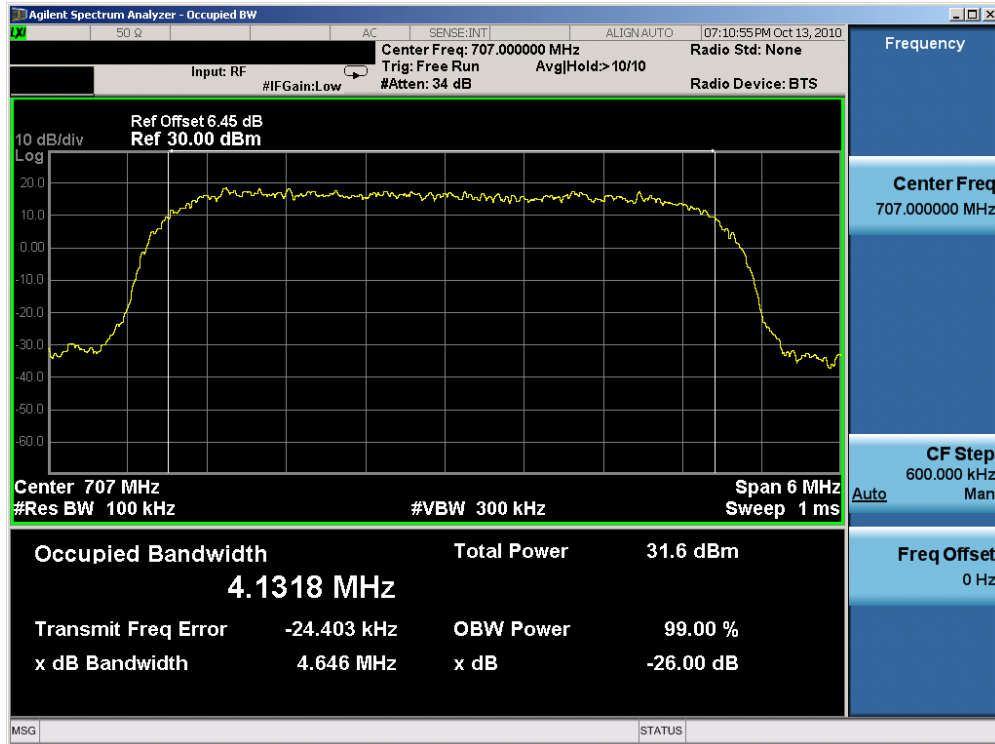
Plot 7-10. Occupied Bandwidth Plot (QPSK Tx=707MHz)
