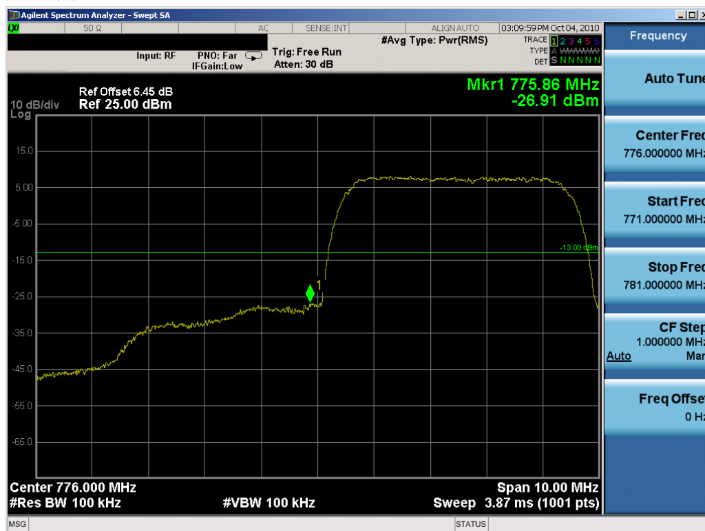
Plot 7-23. Lower Band Edge Plot (16QAM, Tx=778.5MHz)
