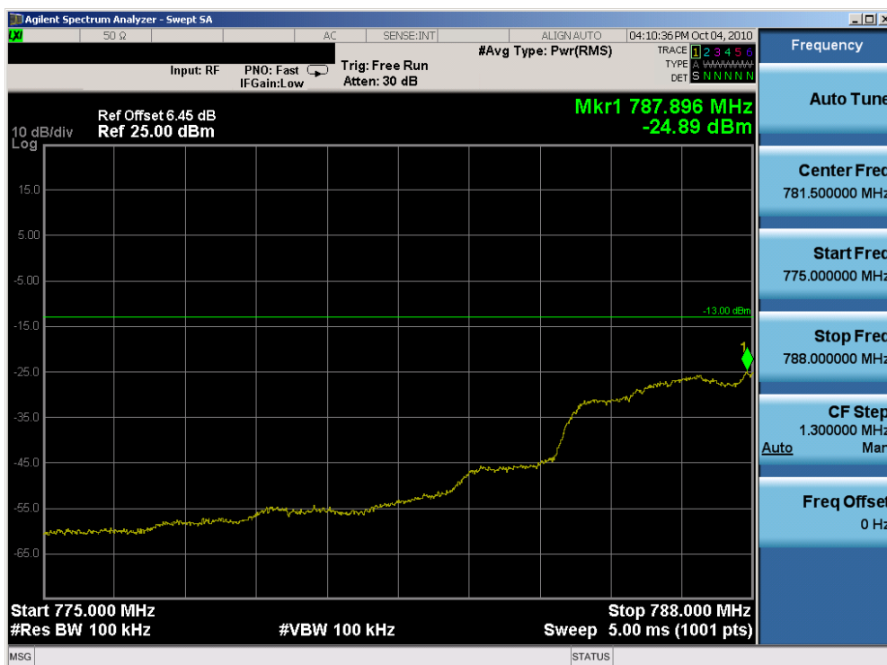
Plot 7-46. Lower Emission Mask 775-788MHz Plot (QPSK, Tx=790.5MHz)
