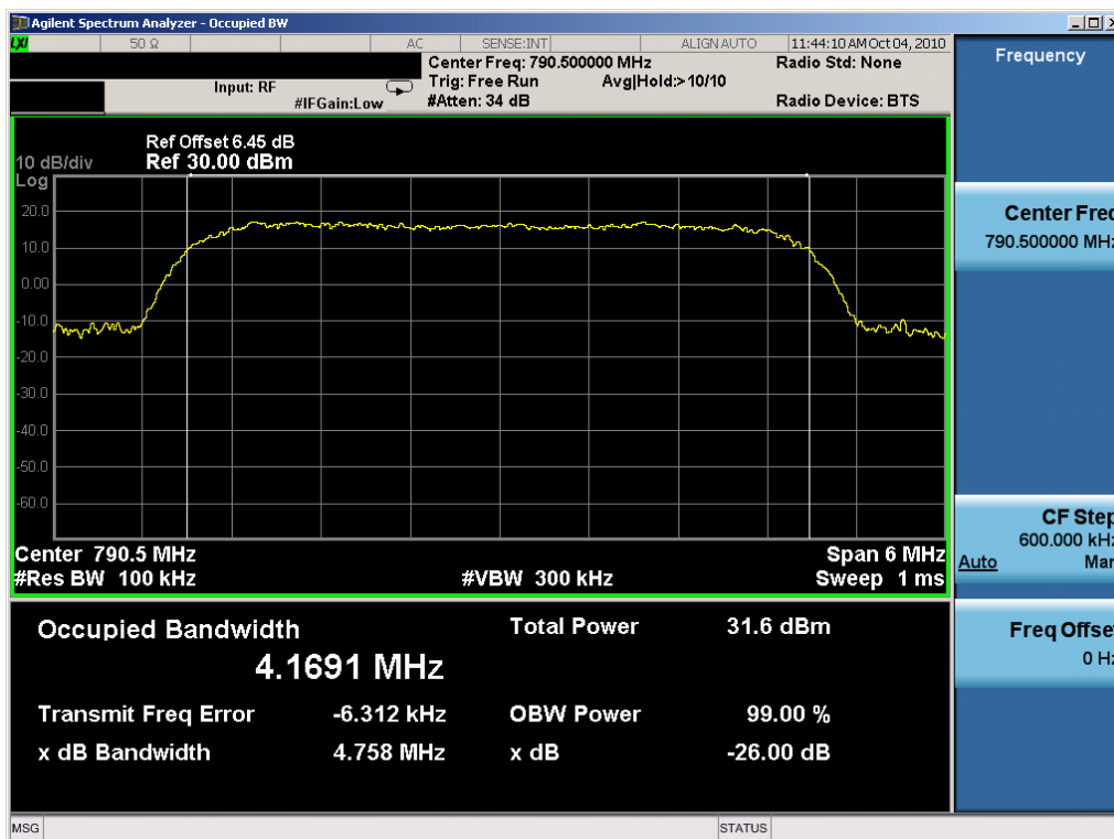
Plot 7-56. Occupied Bandwidth Plot (16QAM, Tx=790.5MHz)
