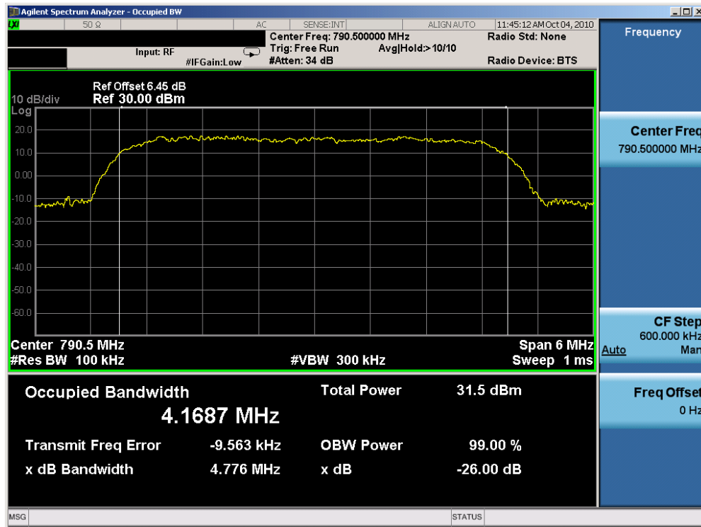
Plot 7-57. Occupied Bandwidth Plot (64QAM, Tx=790.5MHz)
