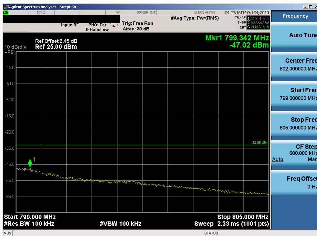
Plot 7-51. Upper Emission Mask 799-805MHz Plot (64QAM, Tx=790.5MHz)
