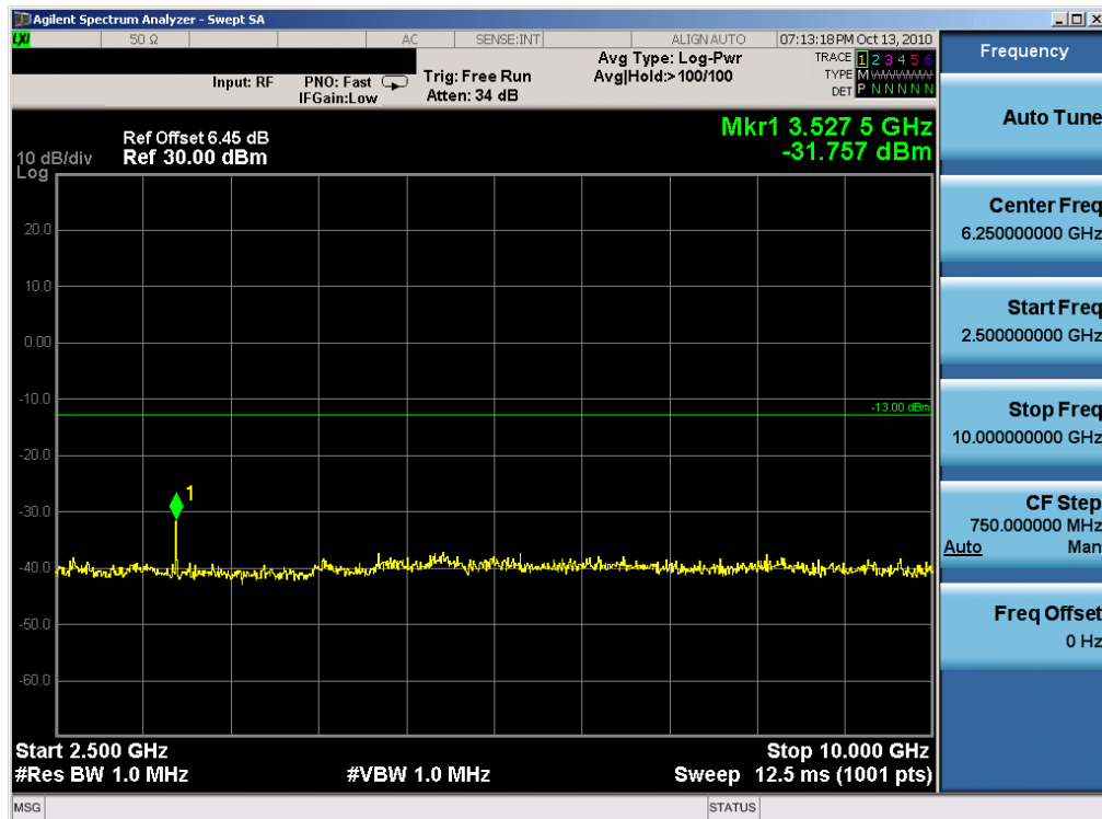
Plot 7-19. Conducted Spurious Plot (64QAM, Tx=707MHz)
