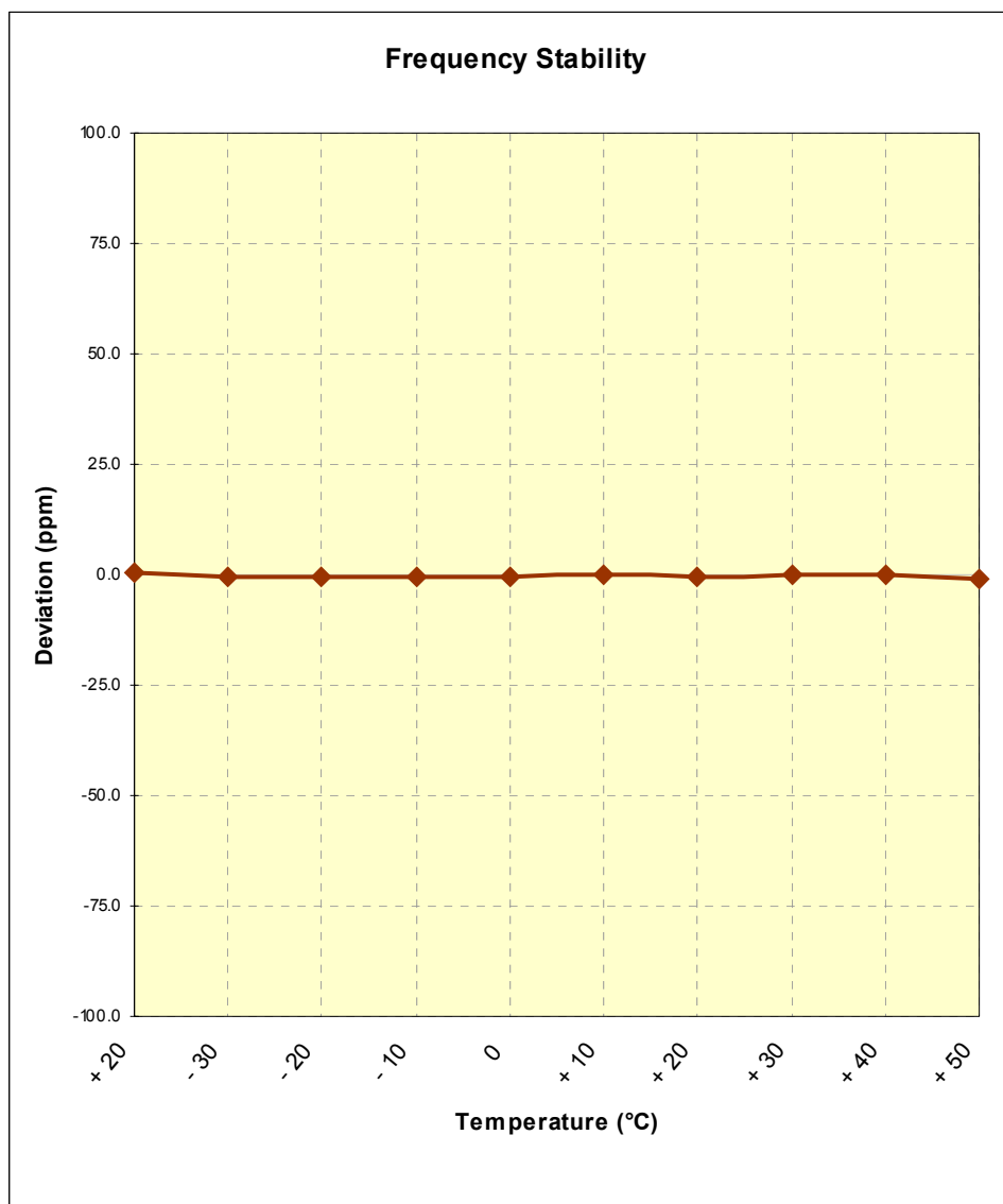
Figure 6-8. Frequency Stability Graph (TD-CDMA Mode Tx=790.5MHz)
