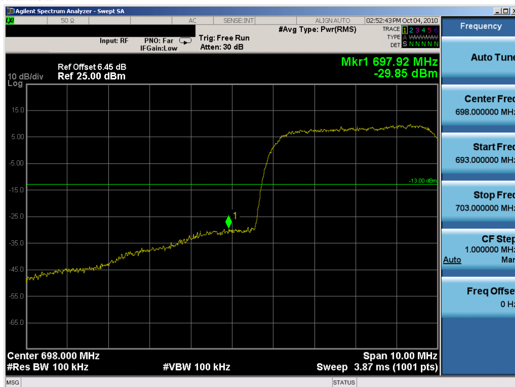
Plot 7-2. Lower Band Edge Plot (16QAM, Tx=701MHz)
