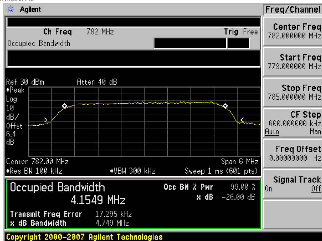
Plot 7-31. Occupied Bandwidth Plot (QPSK, Tx=782 MHz)
