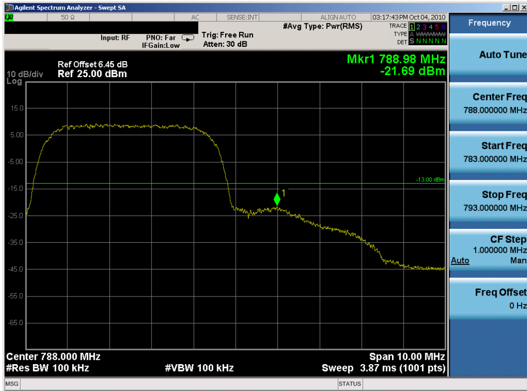
Plot 7-27. Upper Band Edge Plot (64QAM, Tx=785.5MHz)
