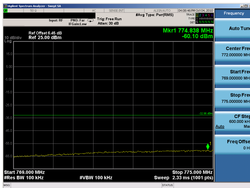
Plot 7-43. Lower Emission Mask 769-775MHz Plot (QPSK, Tx=790.5MHz)
