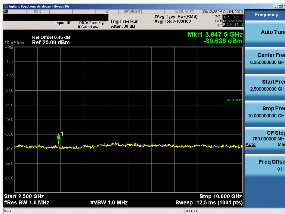
Plot 7-17. Conducted Spurious Plot (64QAM, Tx=701MHz)
