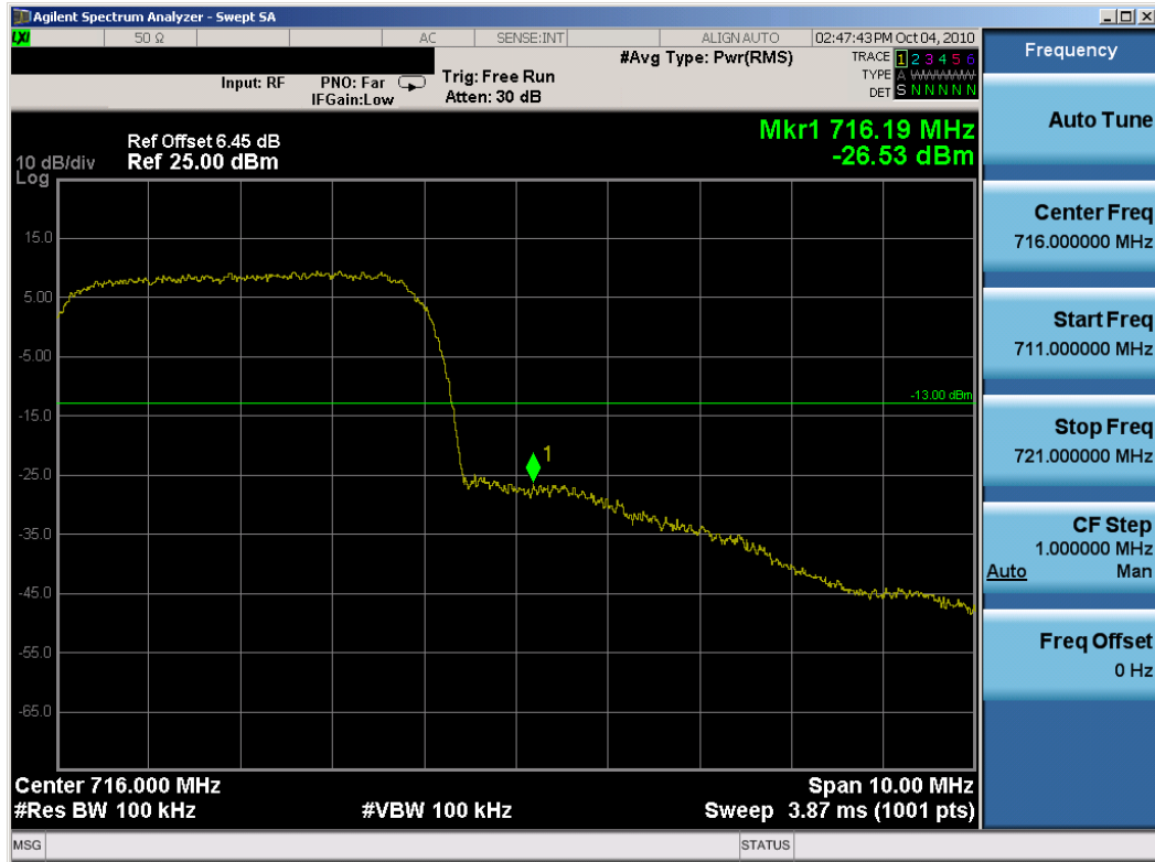
Plot 7-6. Upper Band Edge Plot (64QAM, Tx=713MHz)
