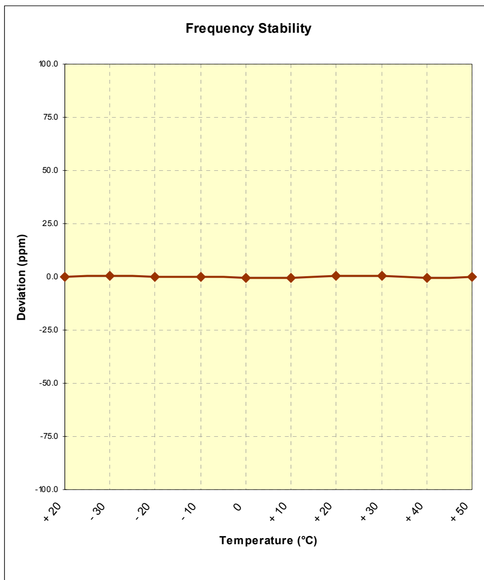
Figure 6-2. Frequency Stability Graph (TD-CDMA Mode Tx=701MHz)
