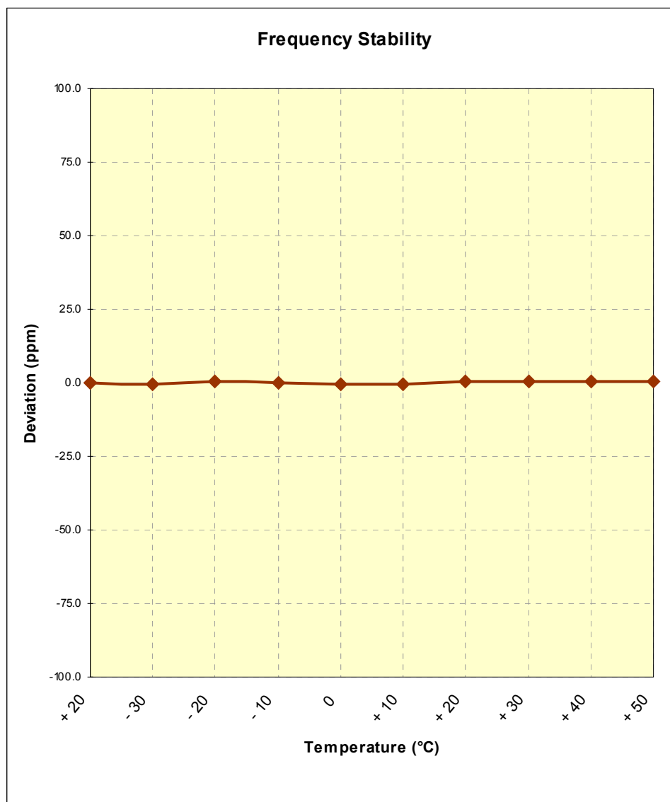
Figure 6-4. Frequency Stability Graph (TD-CDMA Mode - Tx=713MHz)
