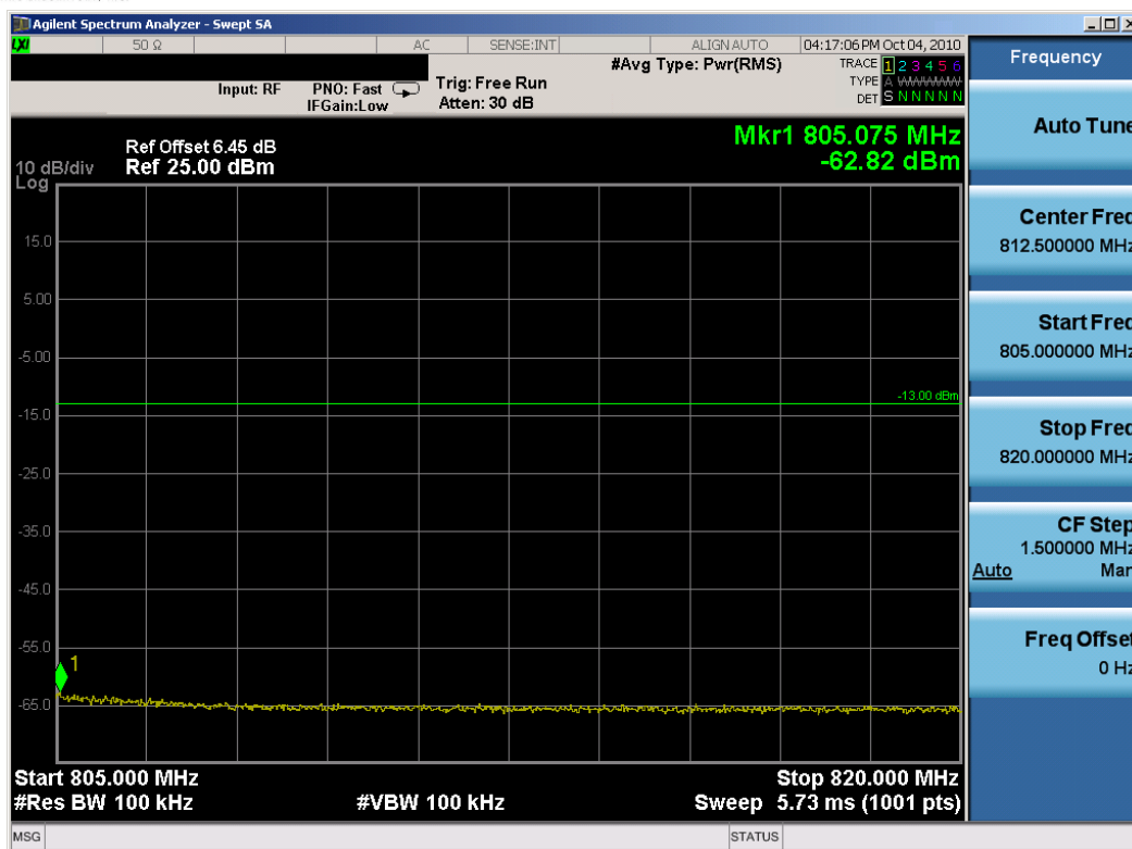
Plot 7-53. Upper Emission Mask Above 805MHz Plot (16QAM, Tx=790.5MHz)
