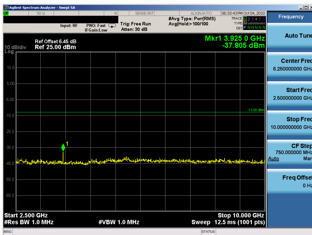
Plot 7-42. Conducted Spurious Plot (64QAM, Tx=785.5MHz)
