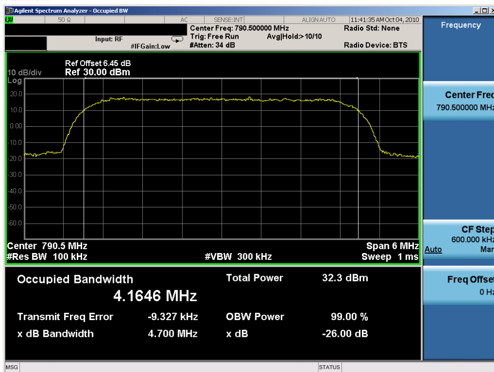
Plot 7-55. Occupied Bandwidth Plot (QPSK, Tx=790.5MHz)
