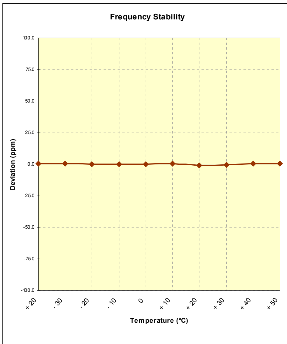
Figure 6-5. Frequency Stability Graph (TD-CDMA Mode Tx=778.5MHz)
