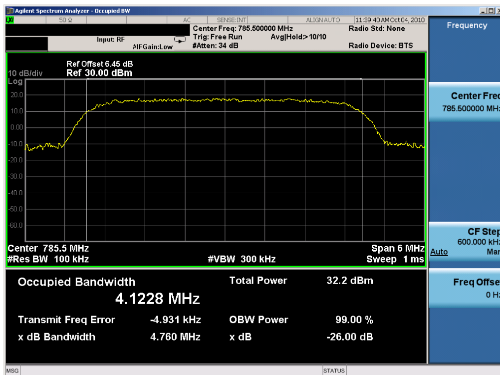
Plot 7-36. Occupied Bandwidth Plot (64QAM, Tx=785.5MHz)
