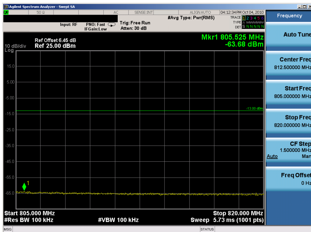
Plot 7-52. Upper Emission Mask Above 805MHz Plot (QPSK, Tx=790.5MHz)
