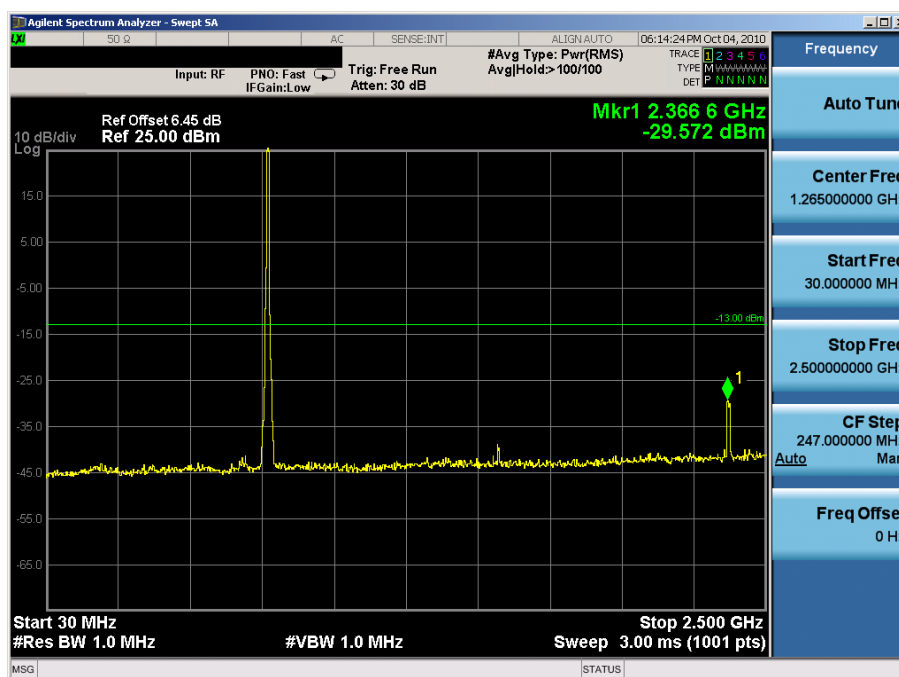
Plot 7-16. Conducted Spurious Plot (64QAM, Tx=701MHz)
