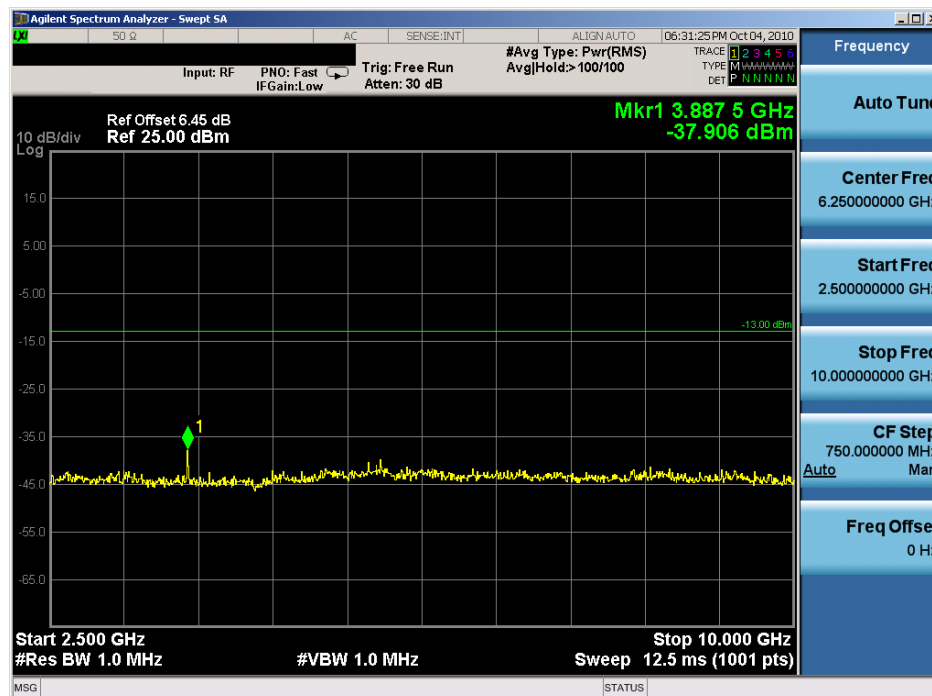
Plot 7-38. Conducted Spurious Plot (64QAM, Tx=778.5MHz)
