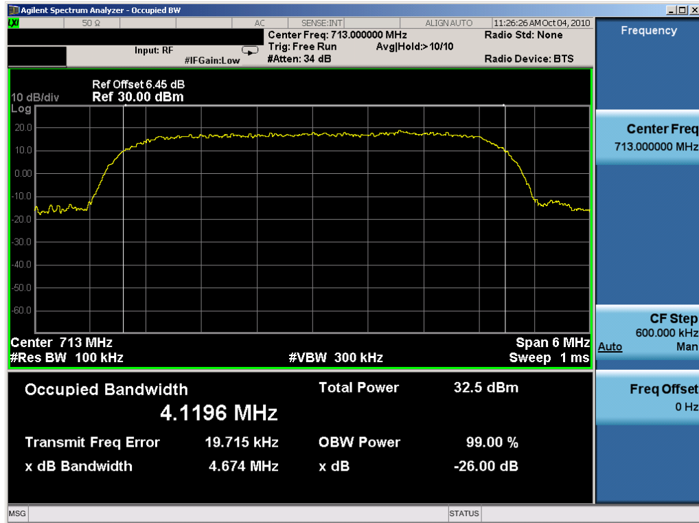
Plot 7-14. Occupied Bandwidth Plot (16QAM, Tx=713MHz)
