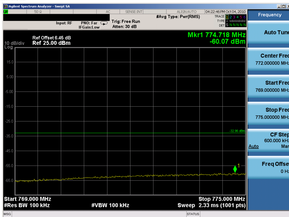
Plot 7-45. Lower Emission Mask 769-775MHz Plot (64QAM, Tx=790.5MHz)
