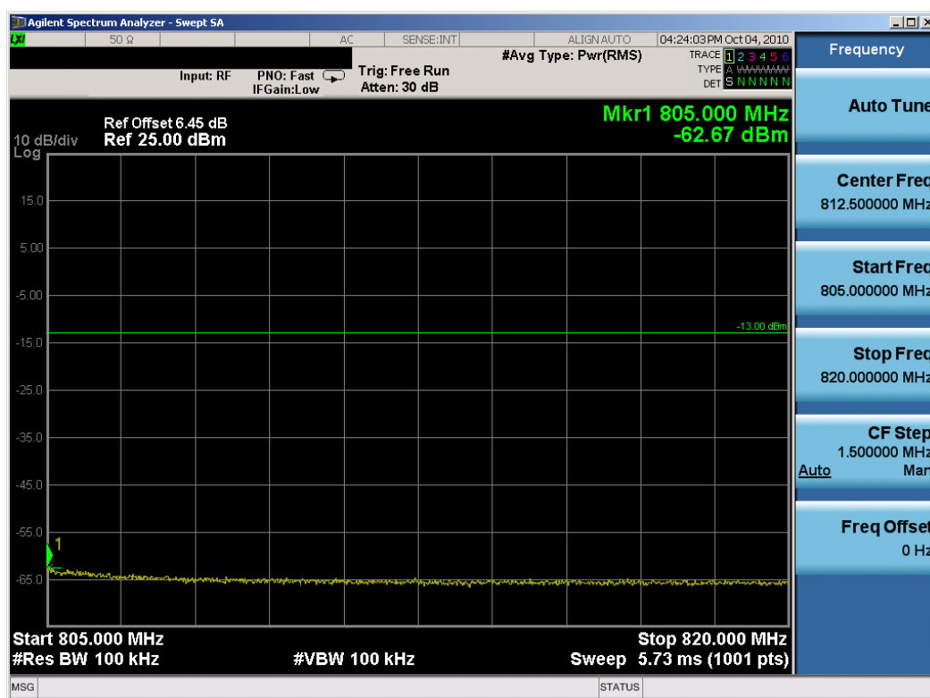
Plot 7-54. Upper Emission Mask Above 805MHz Plot (64QAM, Tx=790.5MHz)
