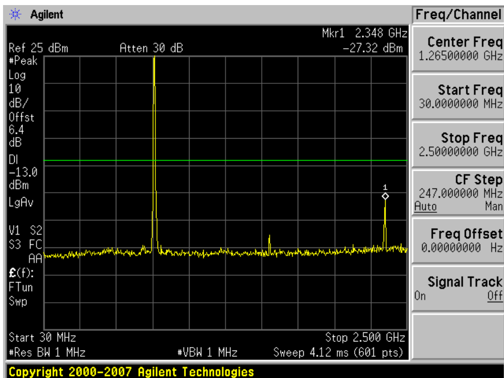
Plot 7-39. Conducted Spurious Plot (64QAM, Tx=782MHz)
