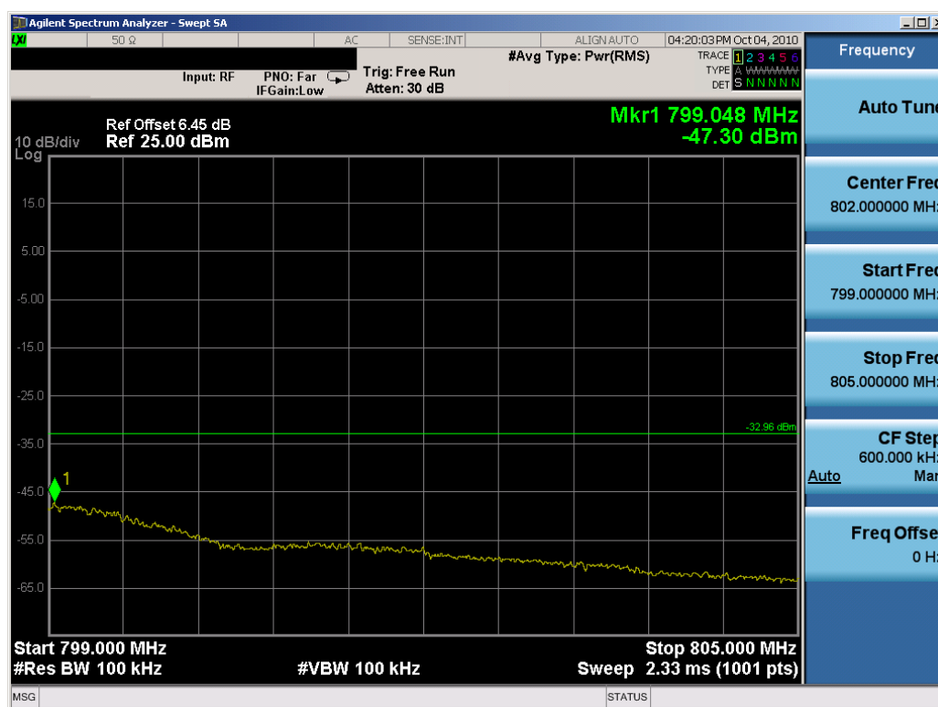
Plot 7-50. Upper Emission Mask 799-805MHz Plot (16QAM, Tx=790.5MHz)
