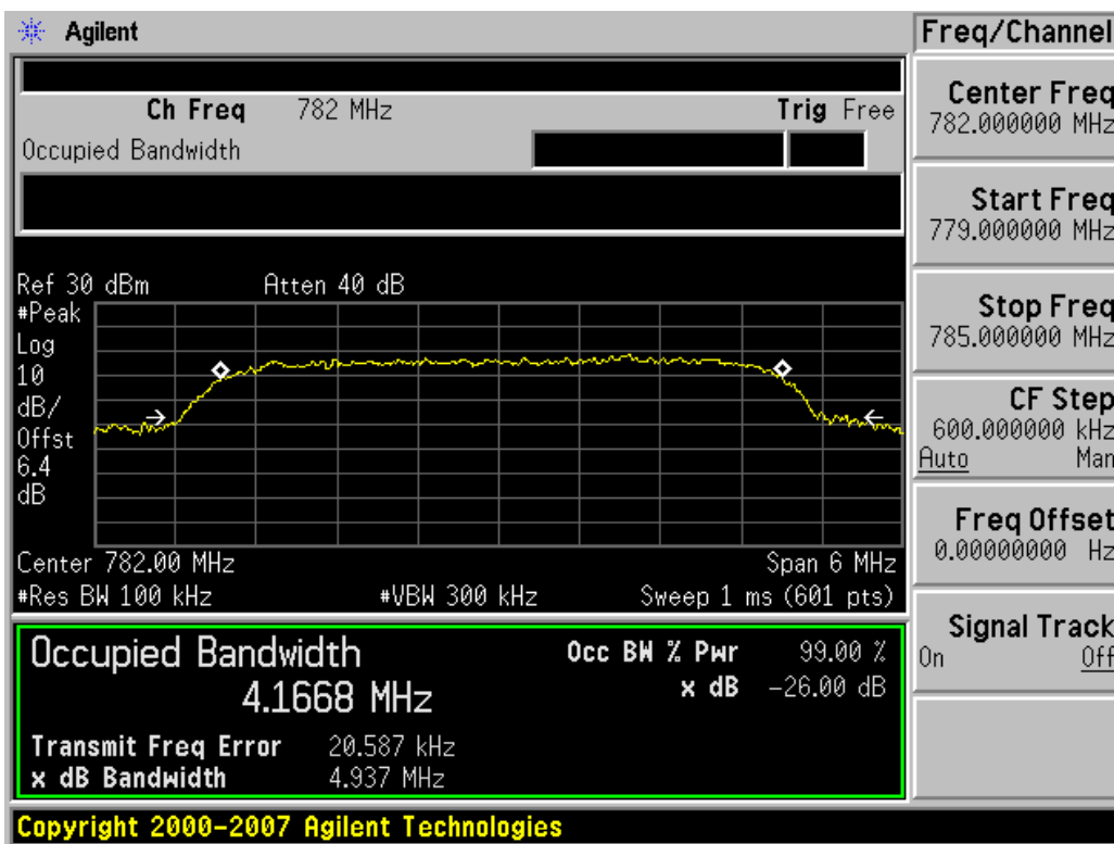
Plot 7-32. Occupied Bandwidth Plot (16QAM, Tx=782 MHz)
