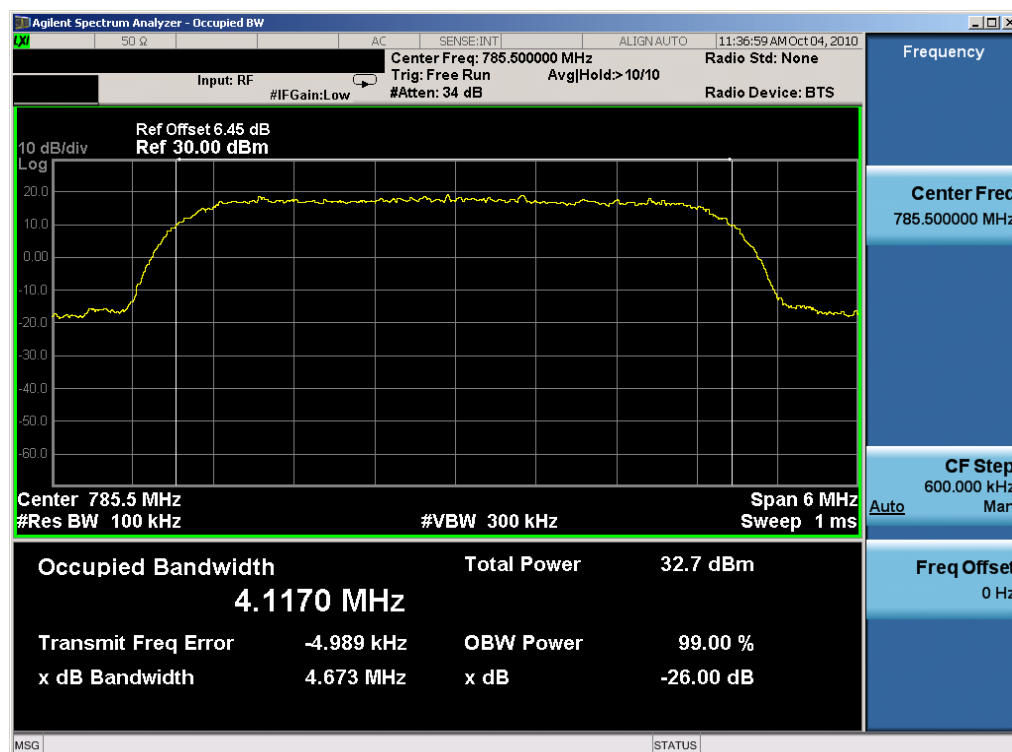
Plot 7-34. Occupied Bandwidth Plot (QPSK, Tx=785.5MHz)
