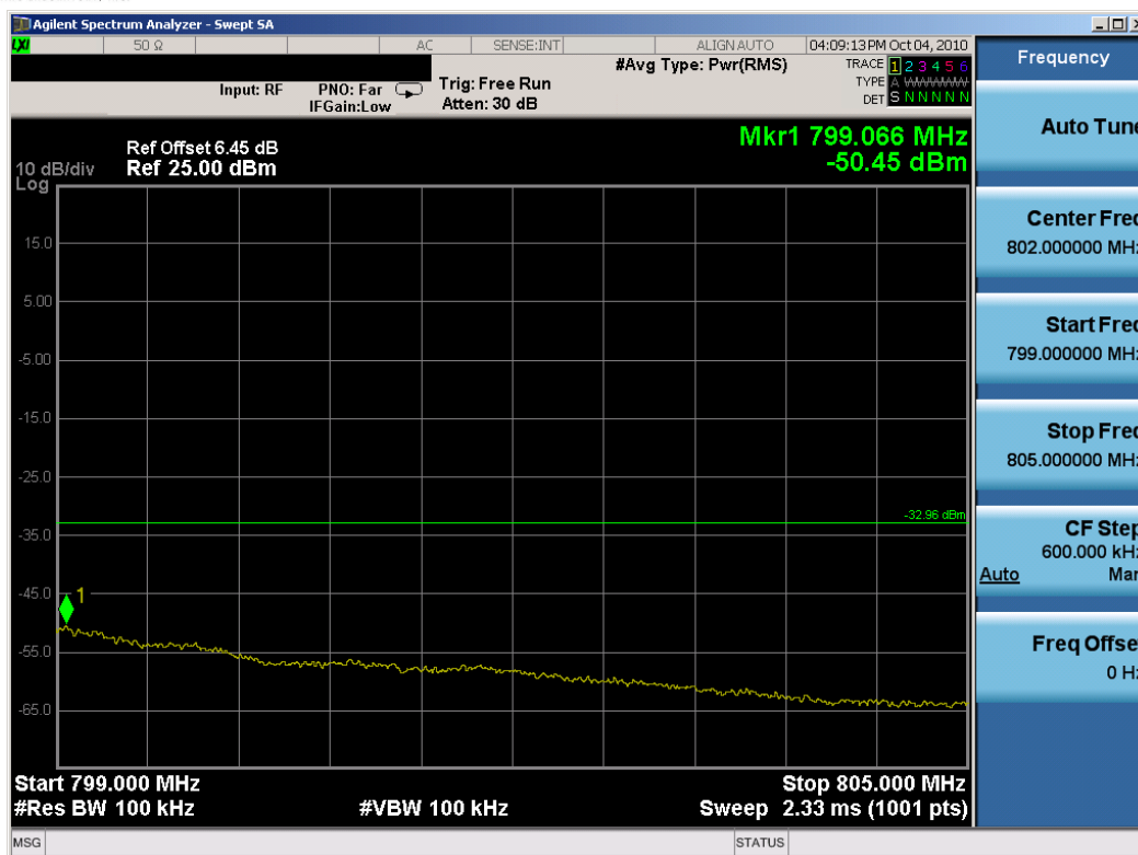
Plot 7-49. Upper Emission Mask 799-805MHz Plot (QPSK, Tx=790.5MHz)
