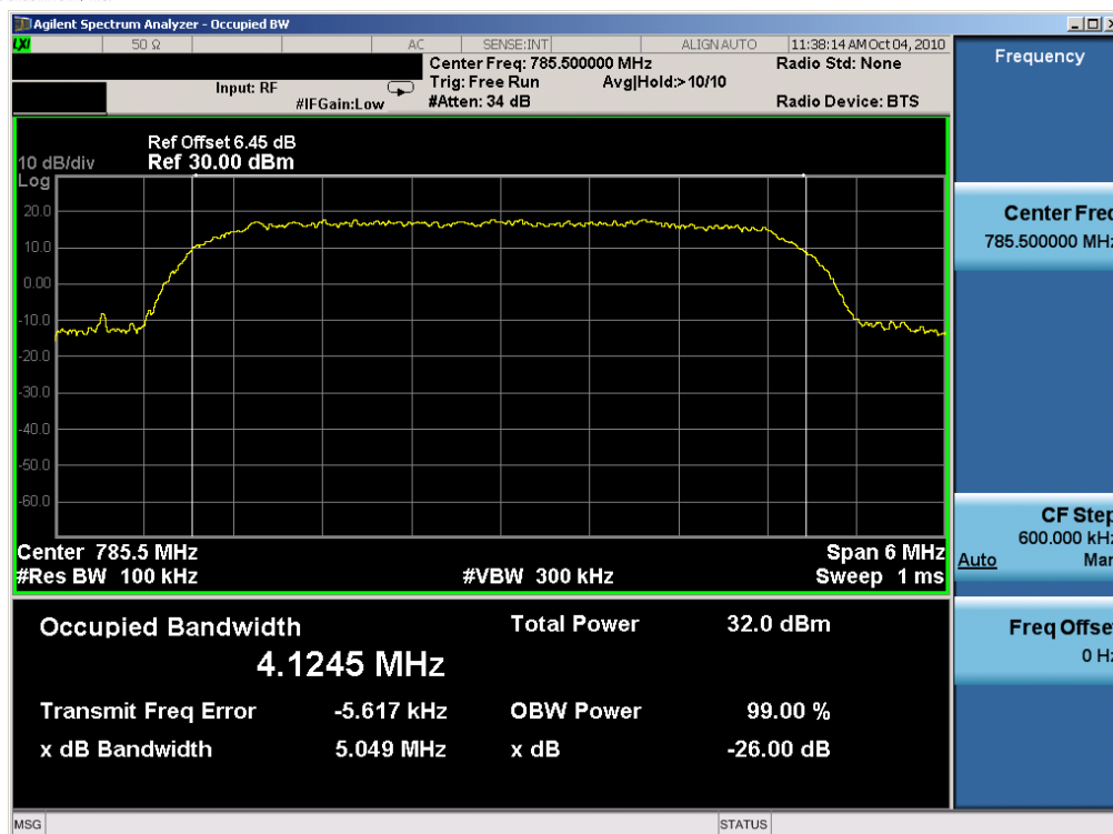
Plot 7-35. Occupied Bandwidth Plot (16QAM, Tx=785.5MHz)
