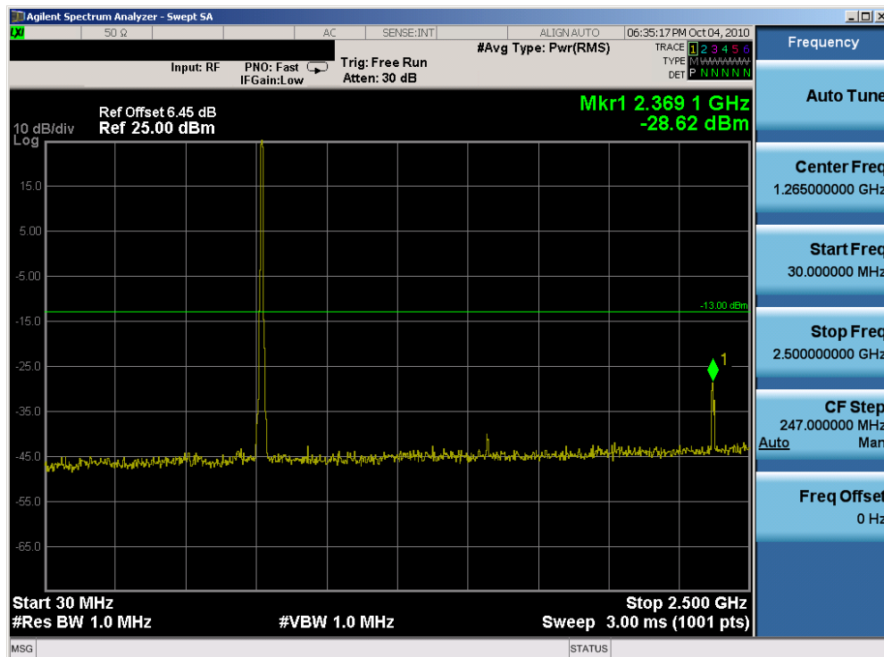
Plot 7-58. Conducted Spurious Plot (64QAM, Tx=790.5MHz)
