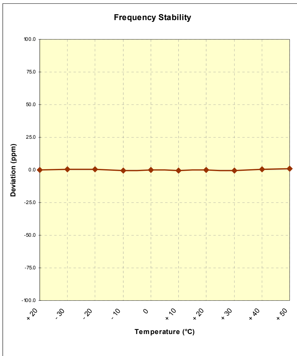
Figure 6-3. Frequency Stability Graph (TD-CDMA Mode Tx=707MHz)
