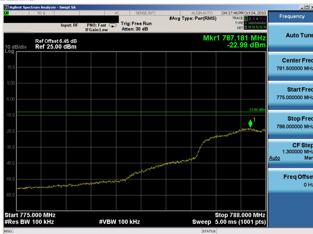
Plot 7-47. Lower Emission Mask 775-788MHz Plot (16QAM, Tx=790.5MHz)
