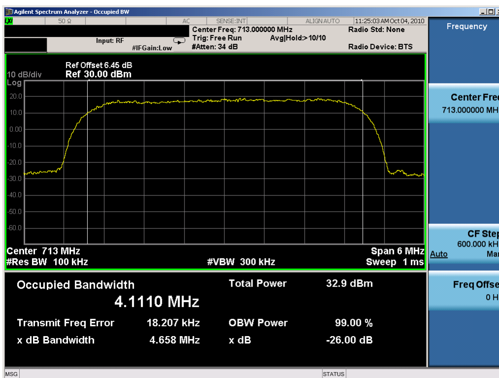
Plot 7-13. Occupied Bandwidth Plot (QPSK, Tx=713MHz)
