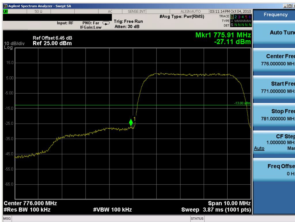
Plot 7-24. Lower Band Edge Plot (64QAM, Tx=778.5MHz)
