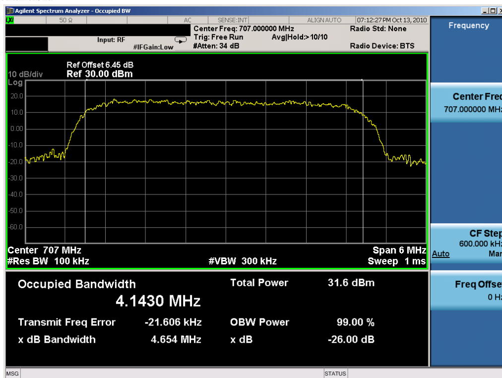
Plot 7-12. Occupied Bandwidth Plot (64QAM, Tx=707MHz)
