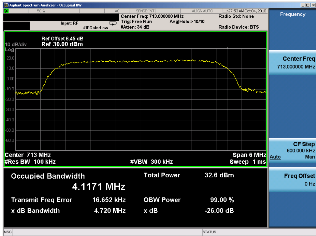
Plot 7-15. Occupied Bandwidth Plot (64QAM, Tx=713MHz)
