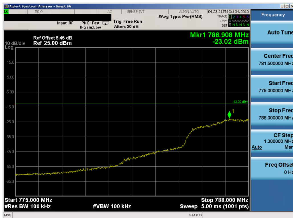
Plot 7-48. Lower Emission Mask 775-788MHz Plot (64QAM, Tx=790.5MHz)
