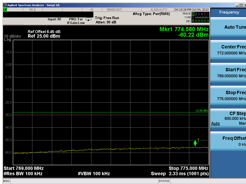
Plot 7-44. Lower Emission Mask 769-775MHz Plot (16QAM, Tx=790.5MHz)
