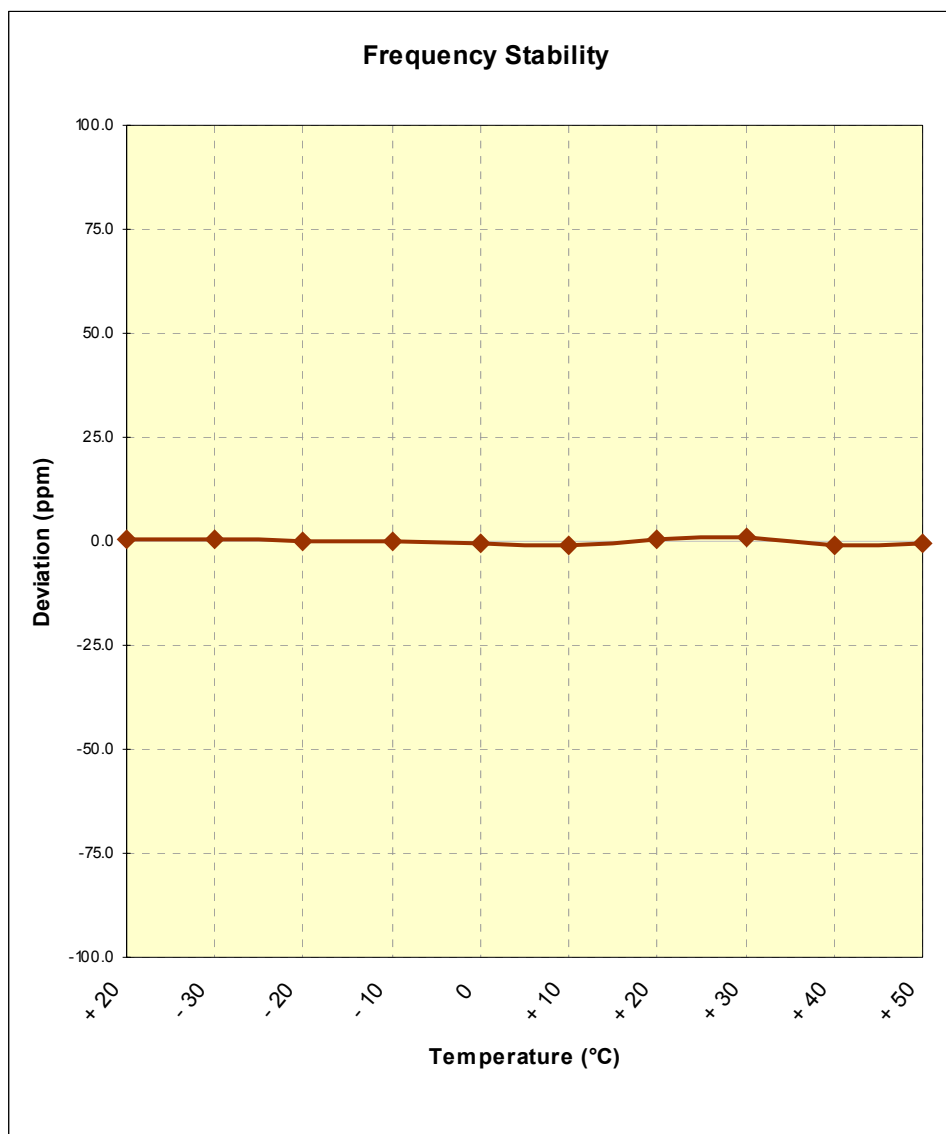
Figure 6-6. Frequency Stability Graph (TD-CDMA Mode Tx=782MHz)
