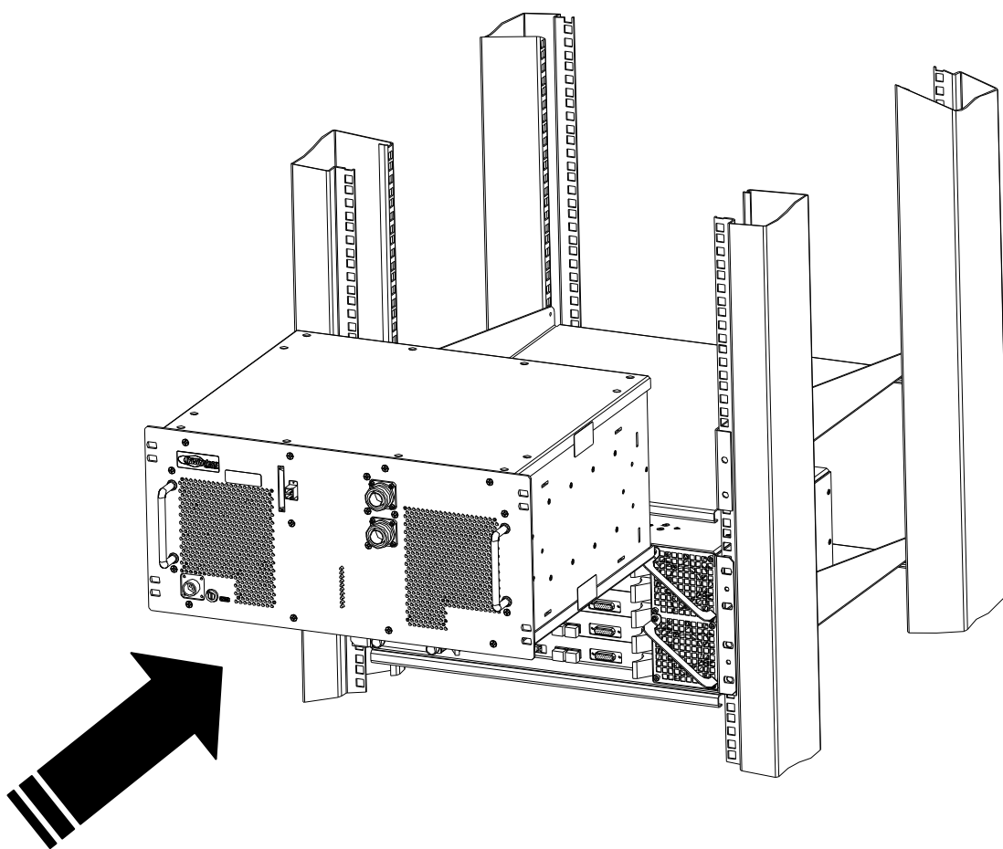
Figure 5-7 : Installing Radio Equipment Shelf
