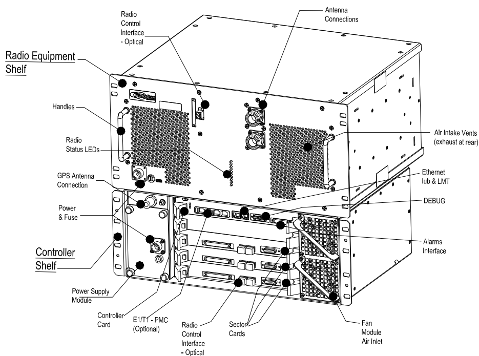
Figure 4-3 : General Description – Front View
