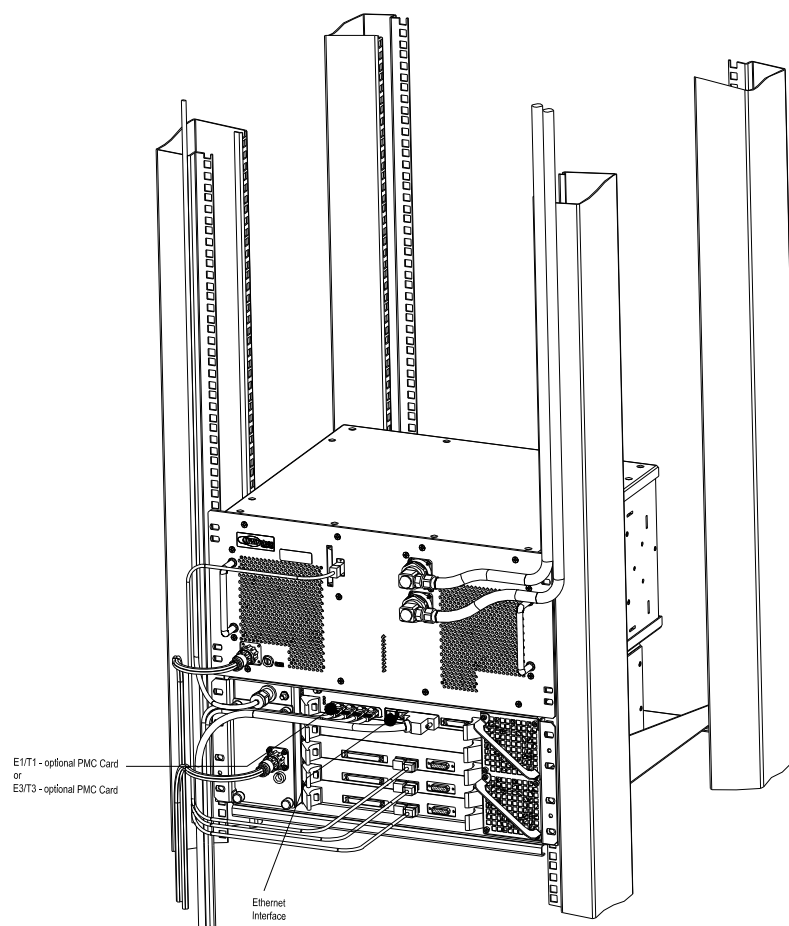
Figure 5-13 : Backhaul Connections
