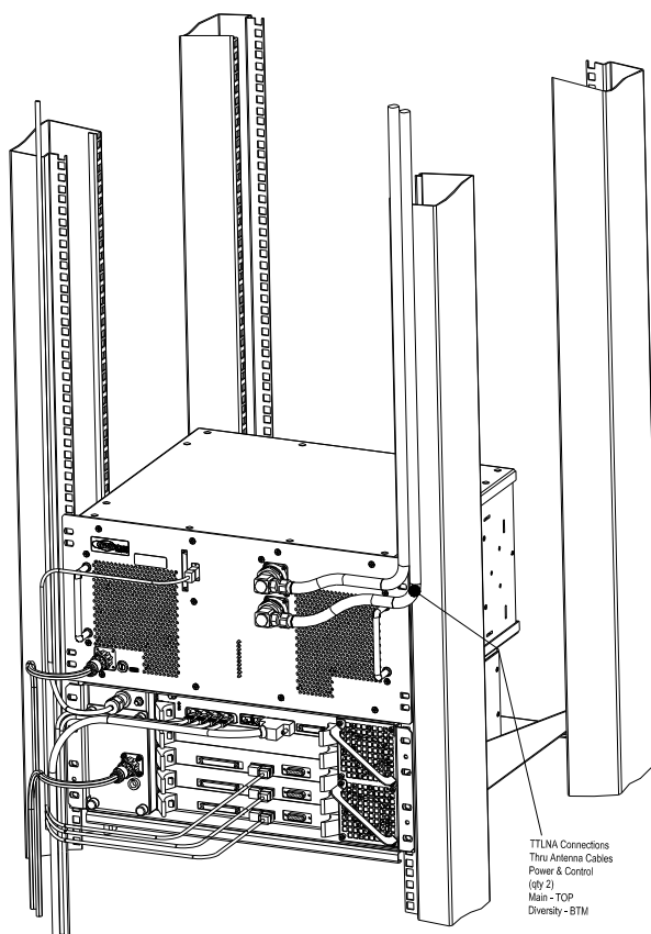
Figure 5-19 : TTLNA Connections
