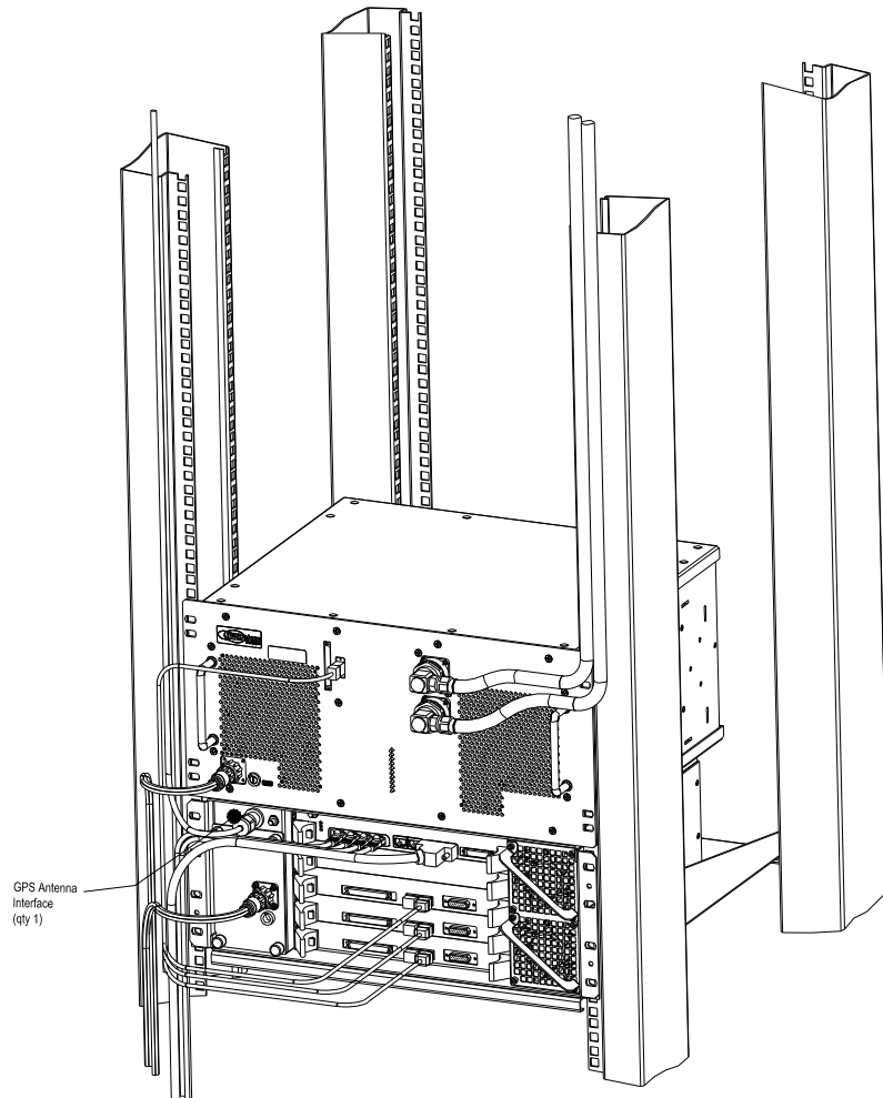
Figure 5-18 : GPS Antenna Connection
