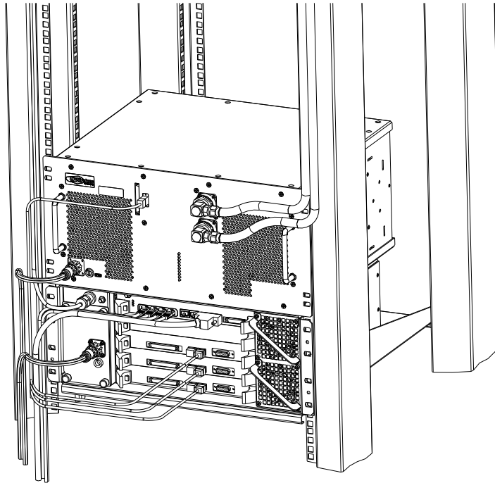
Figure 5-3 : Node B Rack Mount – Single Support Shelf (all cables shown)
