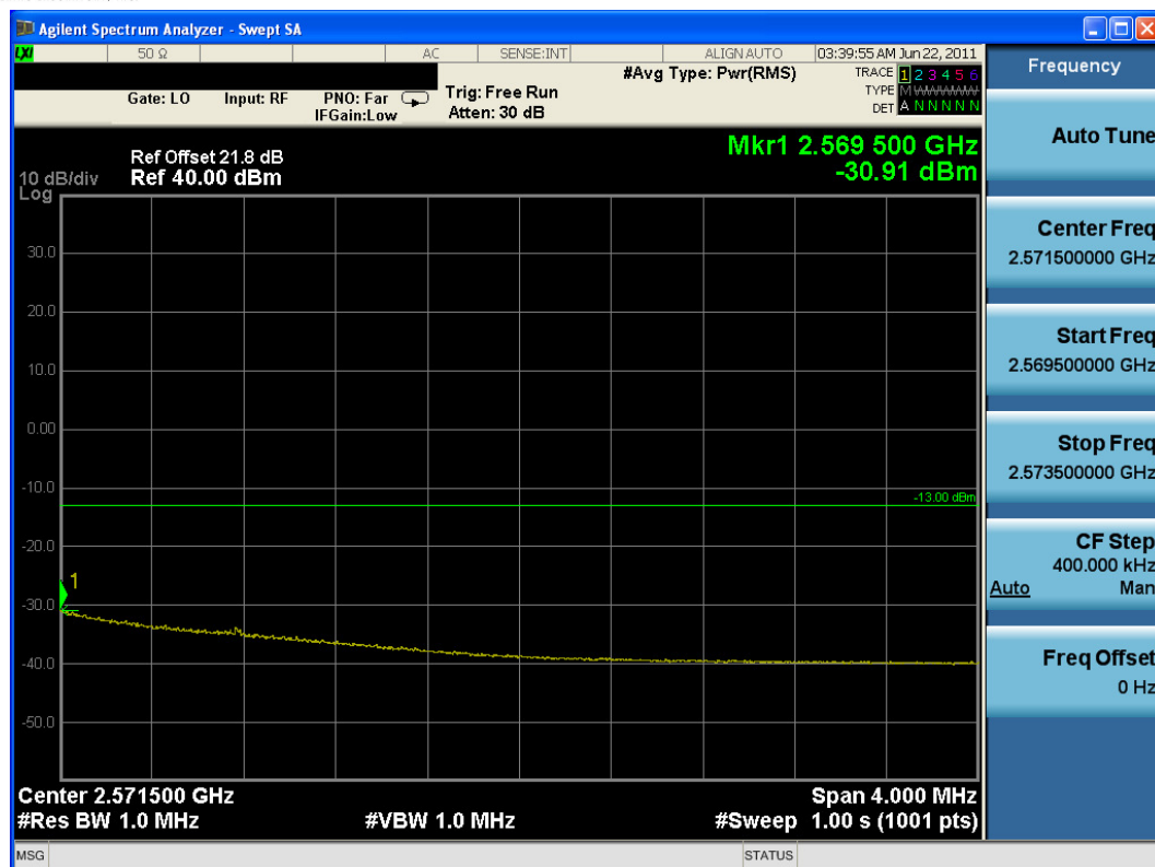
Plot 7-27. Hi 4MHz Plot (TD-CDMA – QPSK) Antenna Port 2
