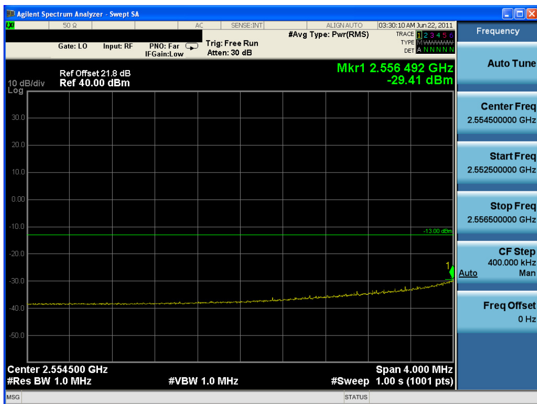
Plot 7-26. Lo 4MHz Plot (TD-CDMA QPSK) Antenna Port 2
