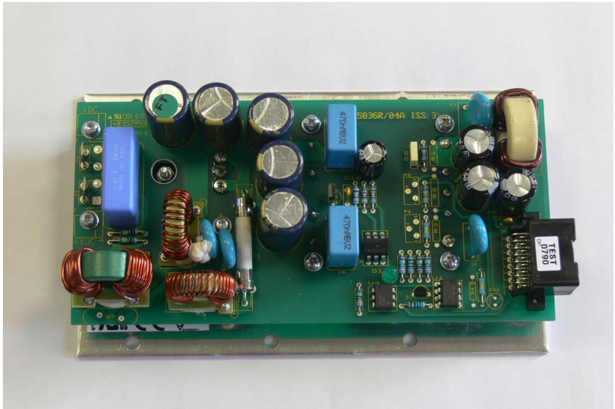
Figure 4: 12VDC Power Supply
