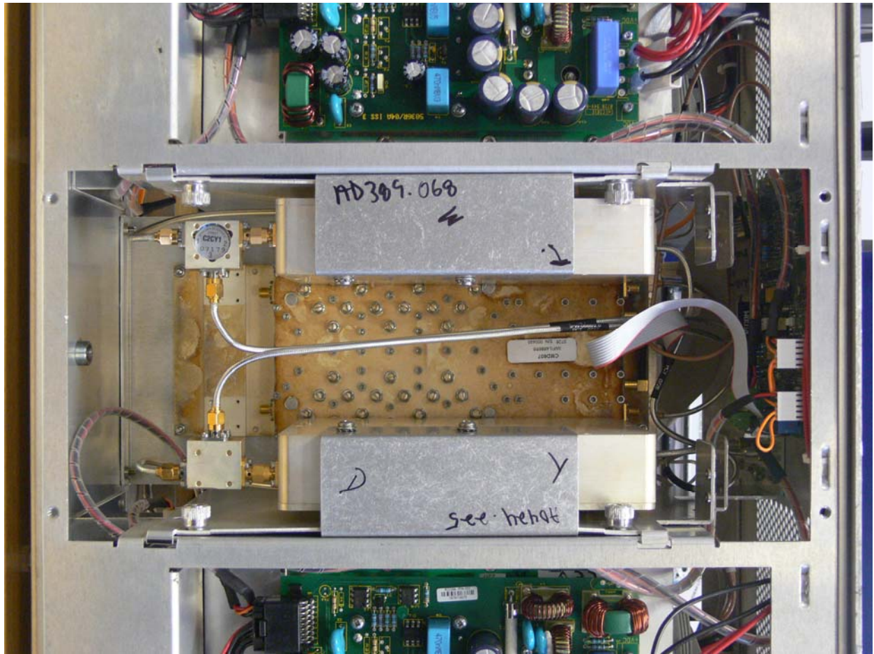
Figure 2: Radio Shelf – Bottom Cover Removed
