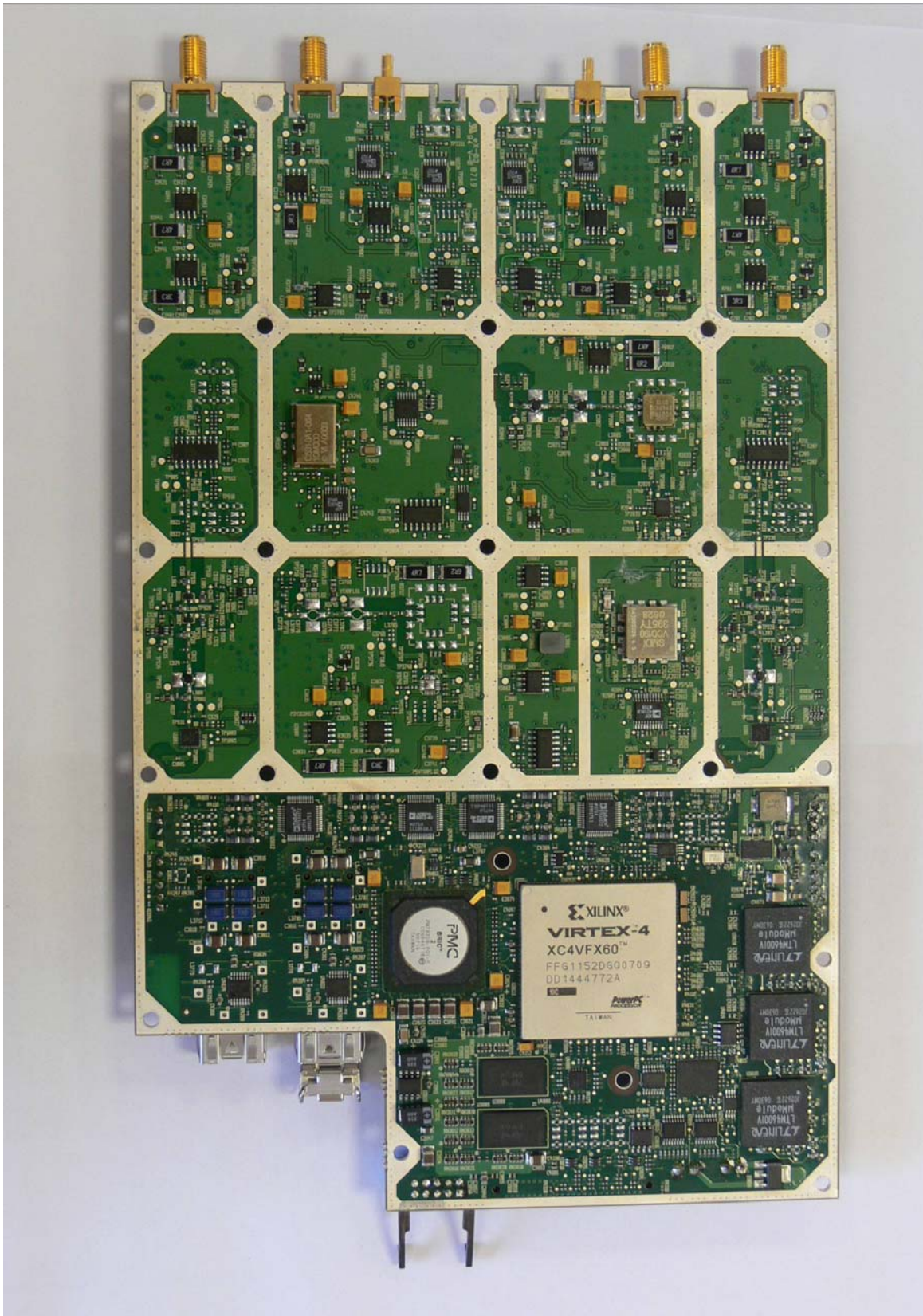
Figure 10: Radio Card- Bottom
