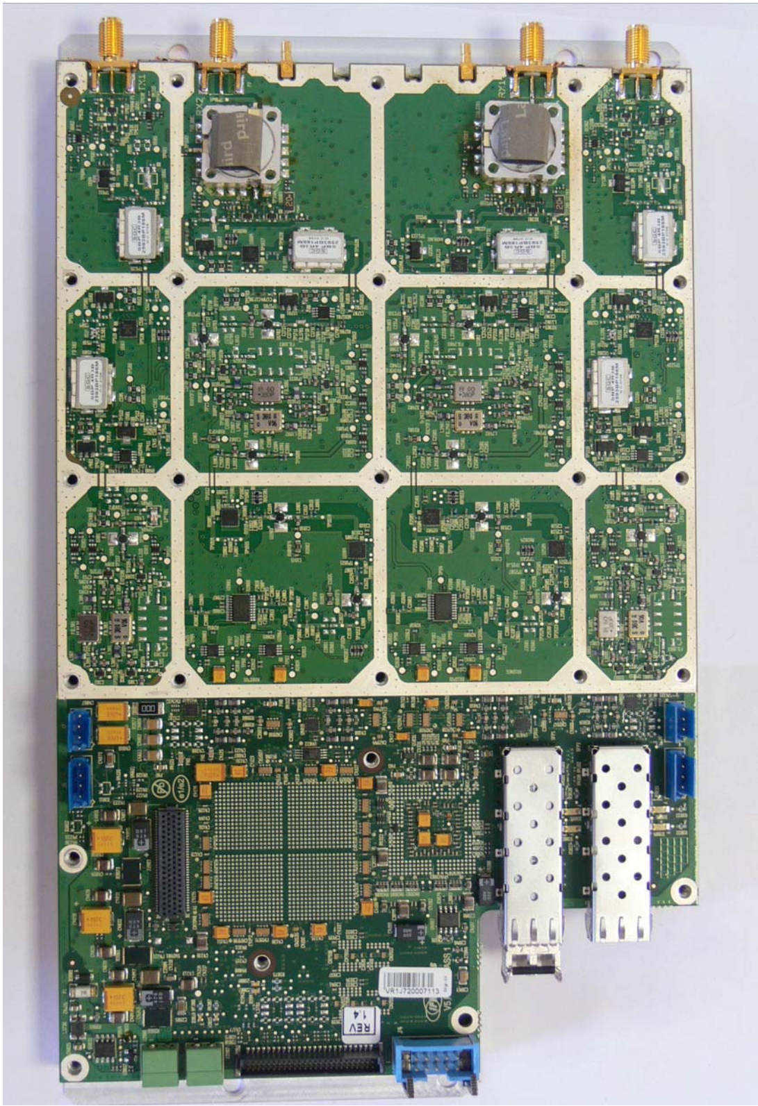
Figure 9: Radio Card - Top
