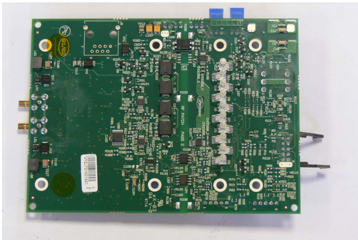
Figure 8: RF Patch Card – Bottom
