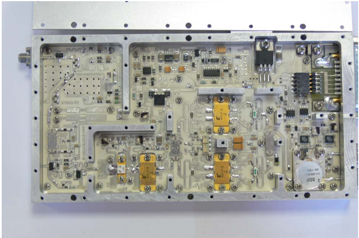
Figure 6: PA Internal – Lid Removed
