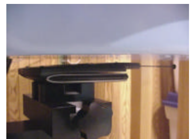
Body SAR Test Setup - Rear of EUT
