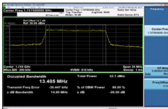
Band4_15MHz_16QAM_75_0_HighCH20325-1747.5
