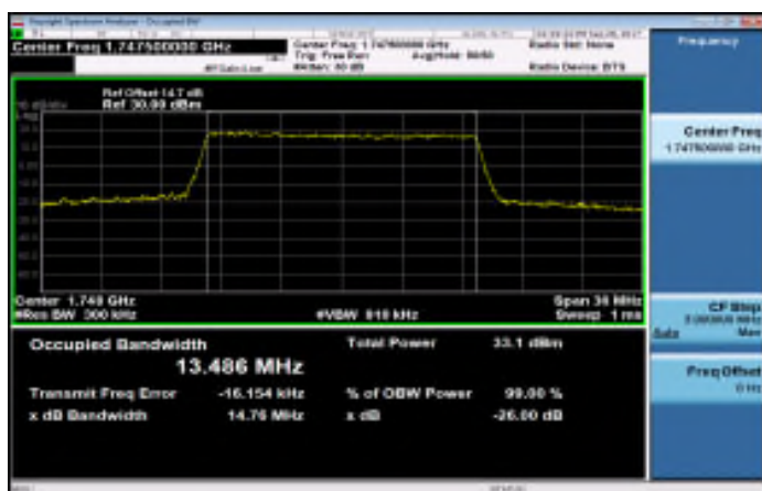
Band4_15MHz_QPSK_75_0_HighCH20325-1747.5
