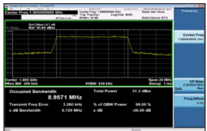
Band2_10MHz_16QAM_50_0_HighCH19150-1905
