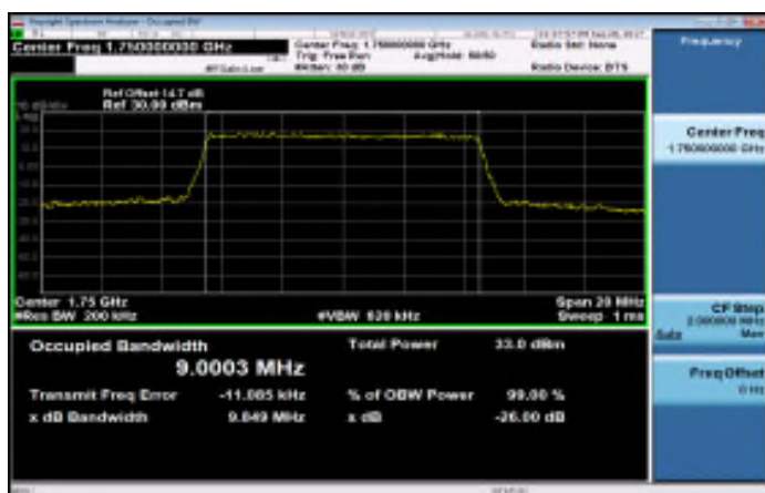
Band4_10MHz_QPSK_50_0_HighCH20350-1750
