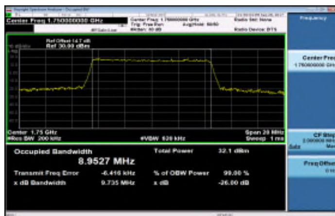
Band4_10MHz_16QAM_50_0_HighCH20350-1750
