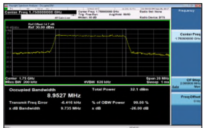
Band4_10MHz_16QAM_50_0_HighCH20350-1750
