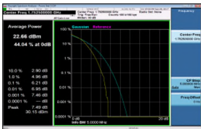
LTE_Band4_5MHz_16QAM_25_0_HighCH20375-1752.5
