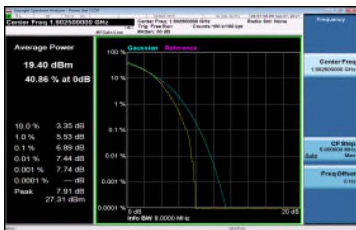
LTE_Band2_15MHz_16QAM_75_0_HighCH19125-1902.5
