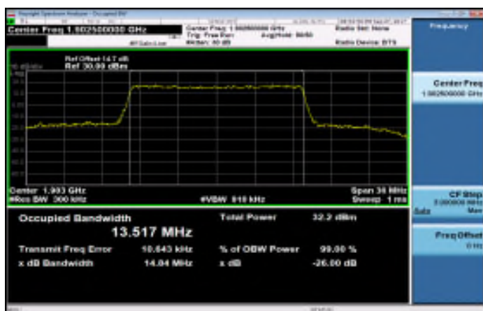
Band2_15MHz_QPSK_75_0_HighCH19125-1902.5
