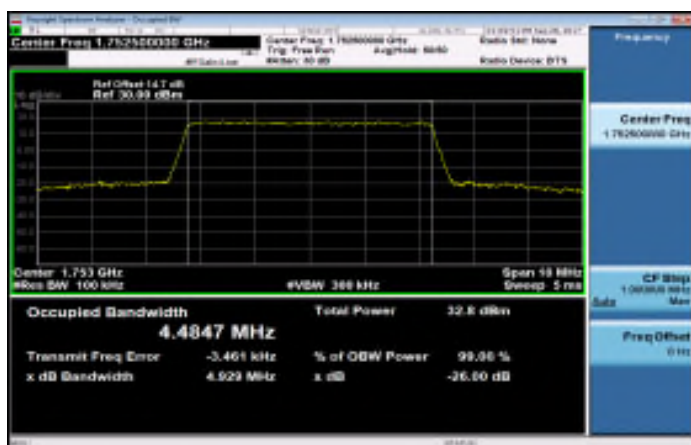
Band4_5MHz_QPSK_25_0_HighCH20375-1752.5
