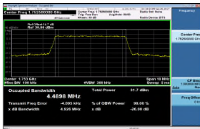
Band4_5MHz_16QAM_25_0_HighCH20375-1752.5
