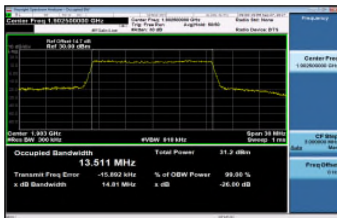
Band2_15MHz_16QAM_75_0_HighCH19125-1902.5
