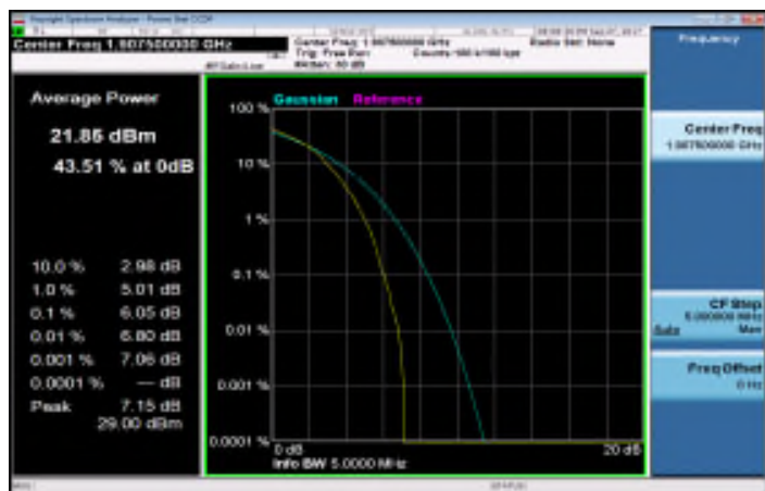
LTE_Band2_5MHz_16QAM_25_0_HighCH19175-1907.5
