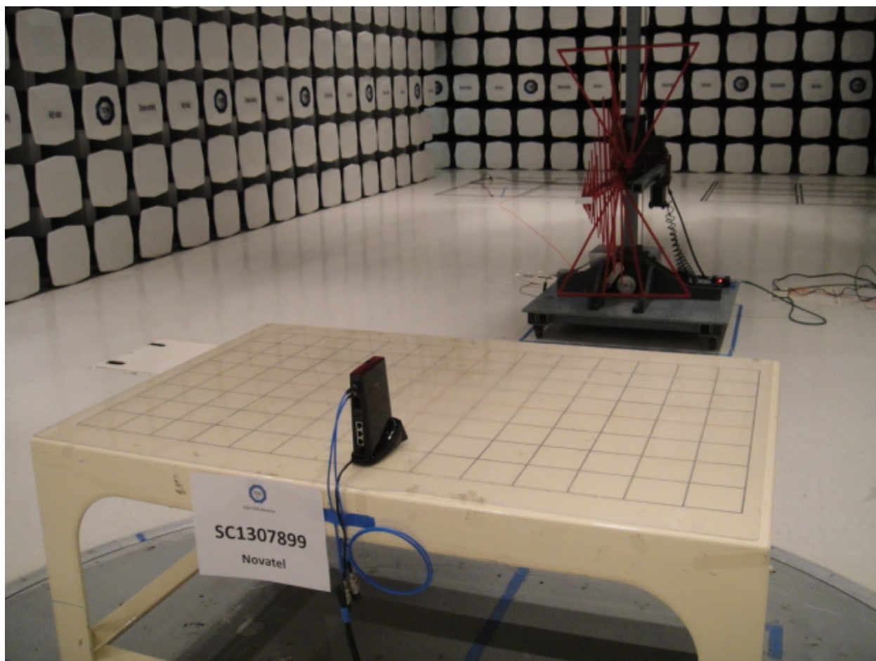
Radiated Emissions Test Setup 1 (WiFi Below 1 GHz)
