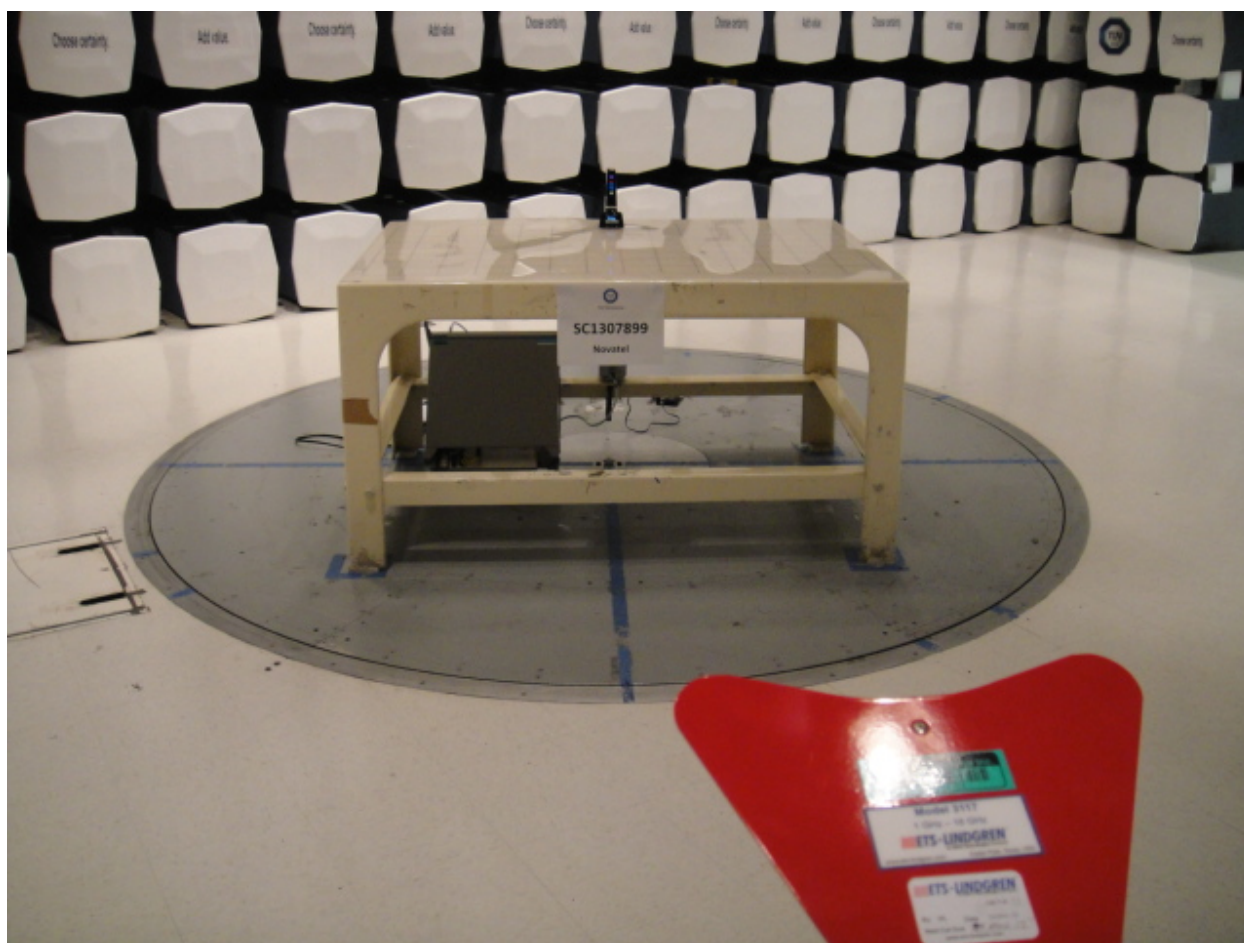
Radiated Emissions Test Setup 4 (LTE/CDMA Above 1 GHz)
