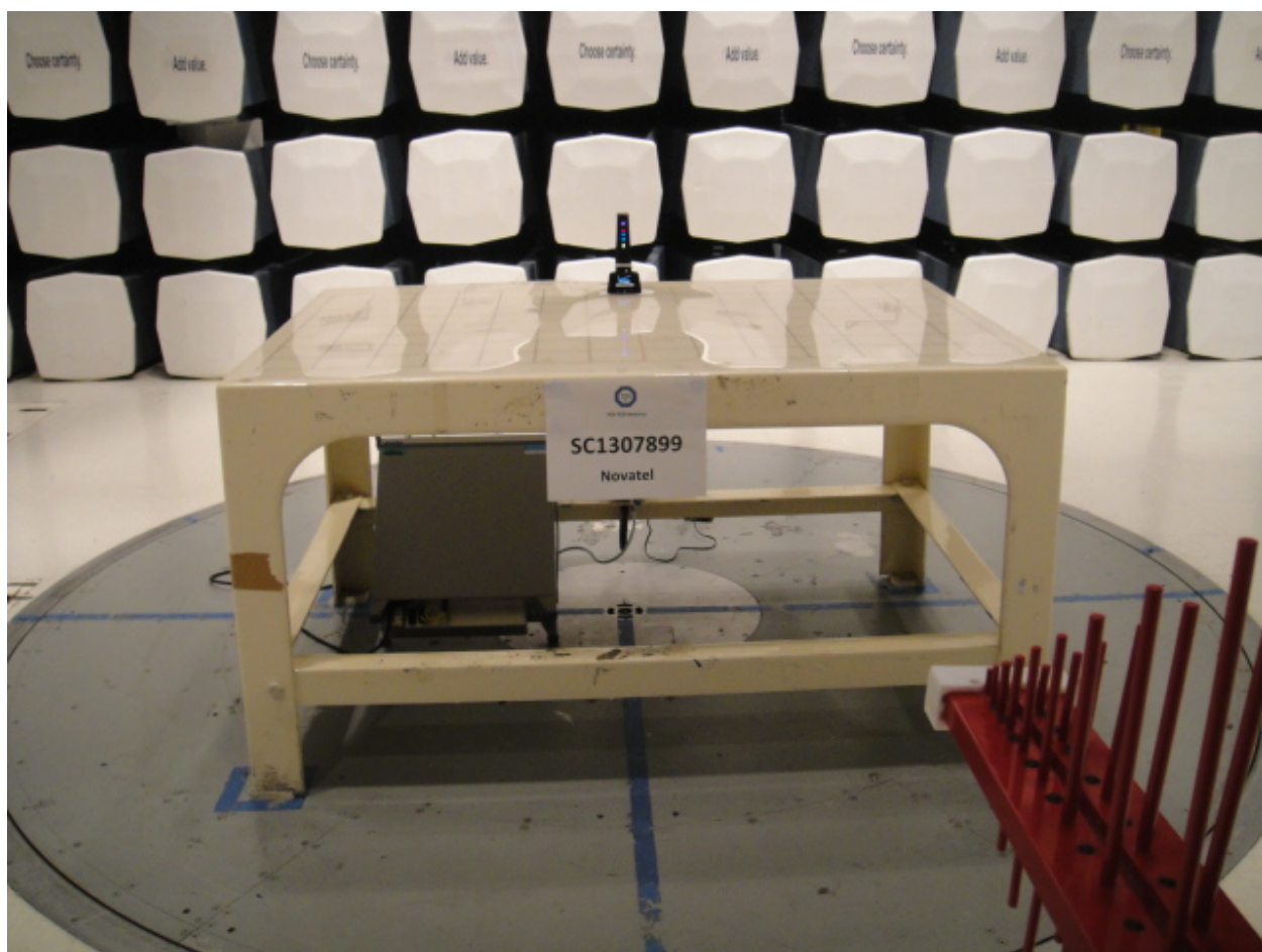
Radiated Emissions Test Setup 3 (LTE/CDMA Below 1 GHz)
