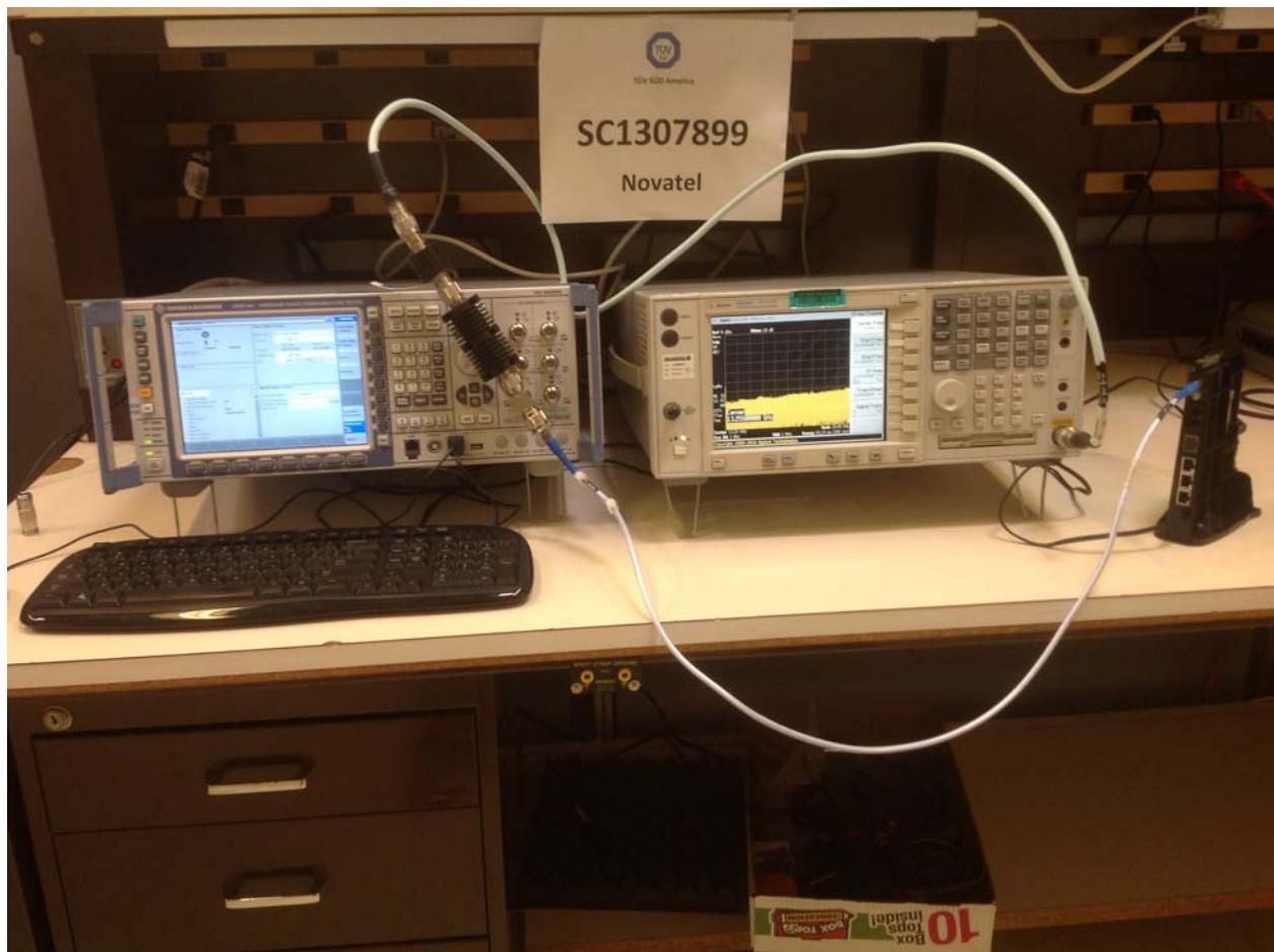
Conducted Port Test Setup 6 (CDMA Measurements with Spectrum Analyzer)
