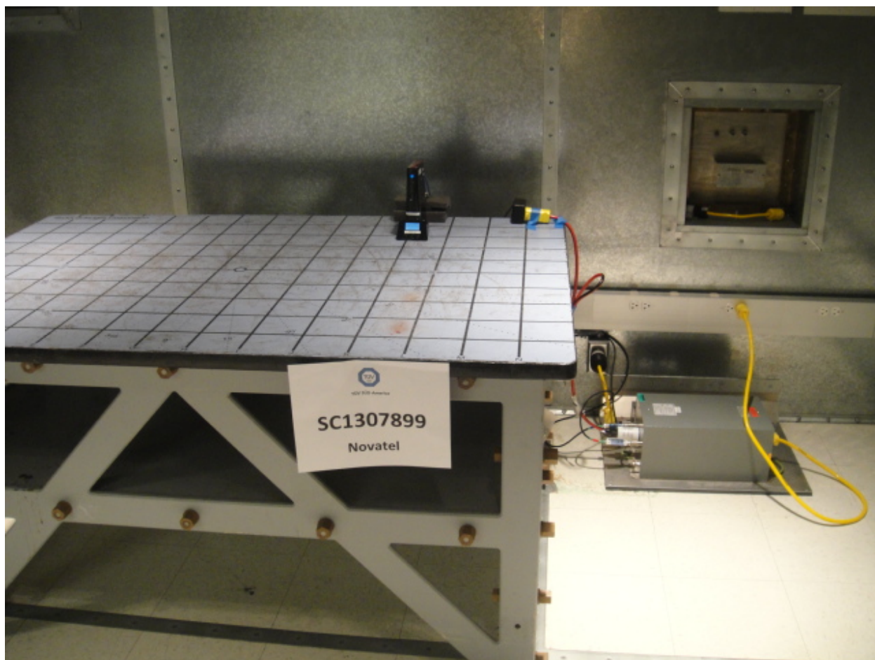
Conducted Emissions Test Setup 1 (Wi Fi)
