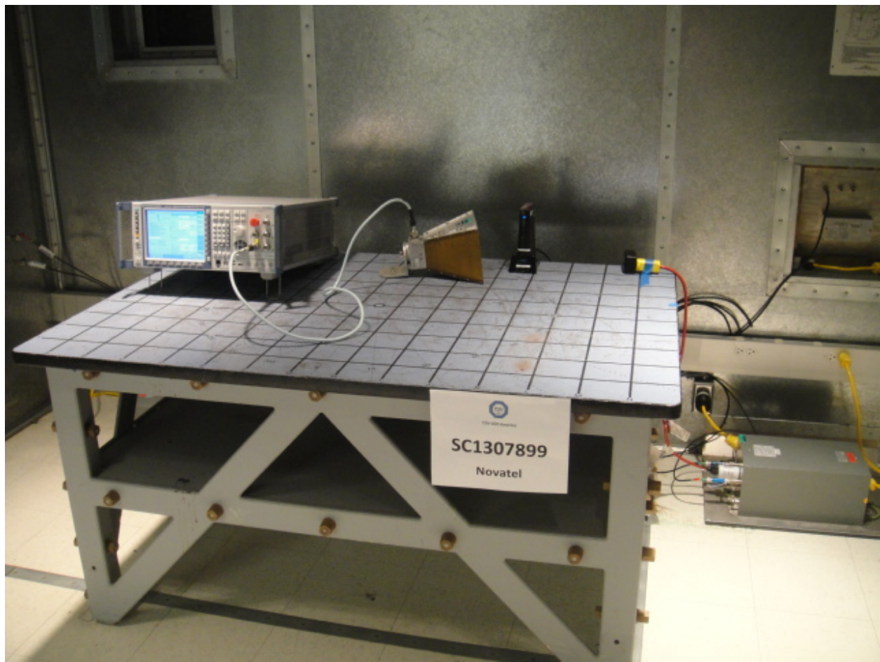
Conducted Emissions Test Setup 2 (LTE/CDMA)
