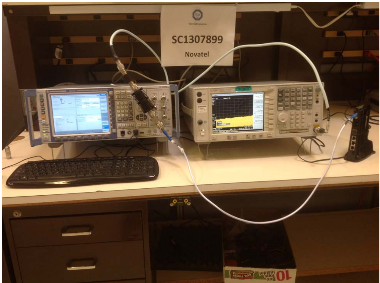
Conducted Port Test Setup 5 (LTE Measurements with Spectrum Analyzer)
