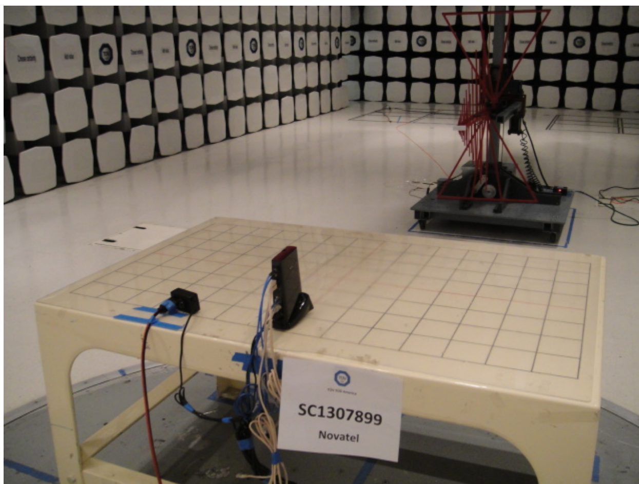
Radiated Emissions Test Setup 5 (RX Mode Below/Above 1 GHz)
