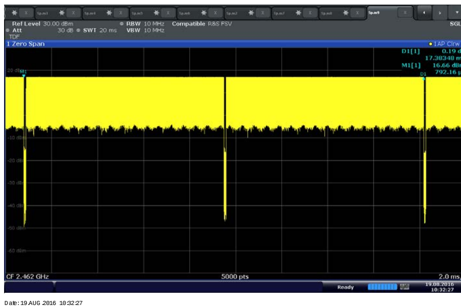
Sample Duty Cycle Calculation (802.11b) 2 Tx /17.383 ms
