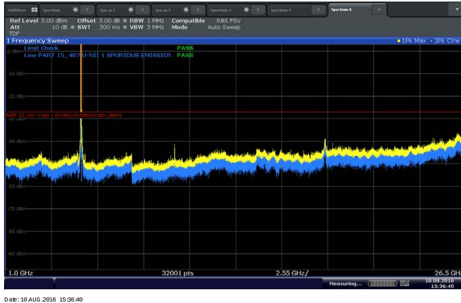
802.11a U-NII 1 Low Channel above 1GHz
