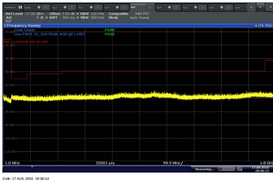
802.11 a U-NII 1 Low Channel below 1GHz
