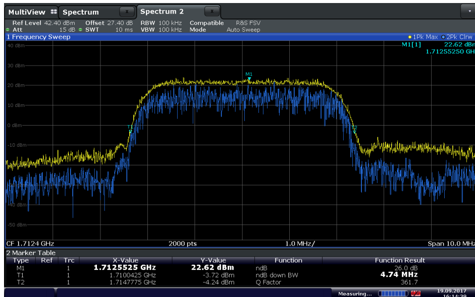
Low Channel 1712.4 MHz 26dB BW
