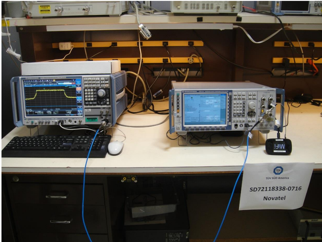
Antenna Conducted Port Bench Measurement
