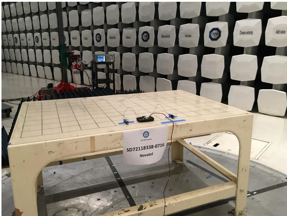
Radiated Emission Measurement Above 1GHz (Front and Back)
