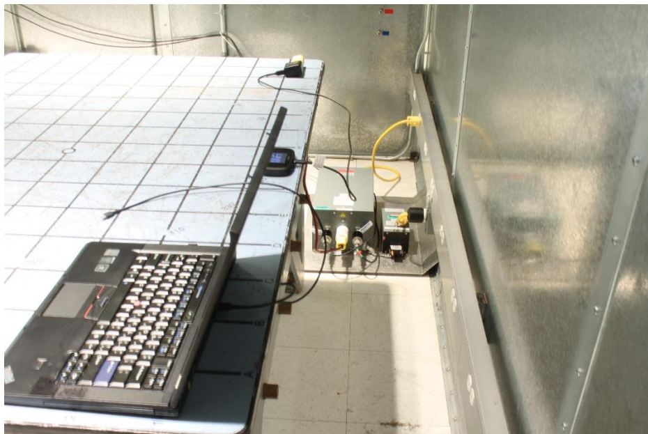
Conducted Emission Measurement (Front and Back)
