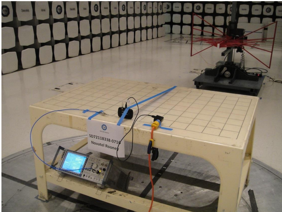
Radiated Emission Measurement Below 1GHz (Front and Back)
