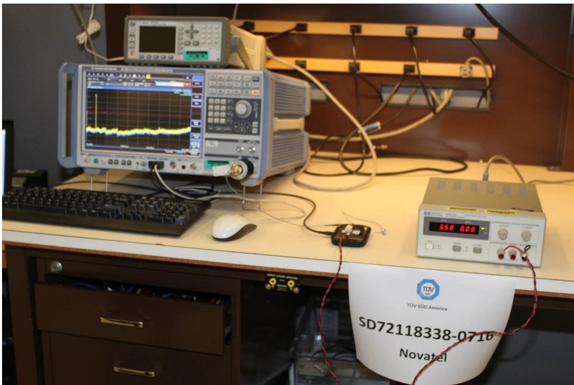
Antenna Conducted Port Bench Measurement
