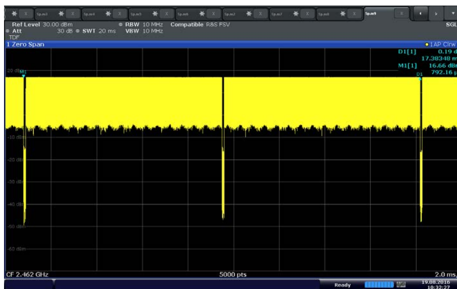
Sample Duty Cycle Calculation (802.11b) 2 Tx /17.383 ms
