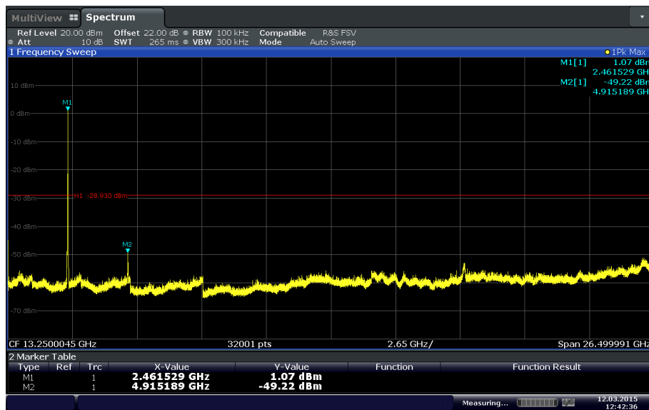
802.11n ht20 MIMO mode Channel 10 (2457MHz)
