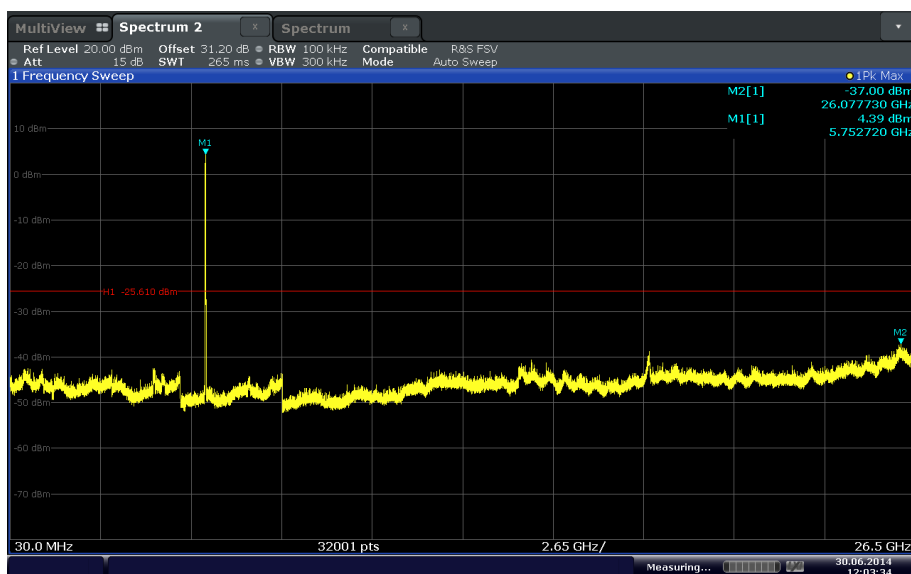
802.11n ht20 mode MIMO Channel 149 (5745MHz)
