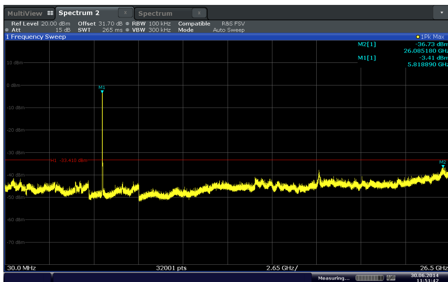
802.11a mode SISO Channel 165 (5825MHz)
