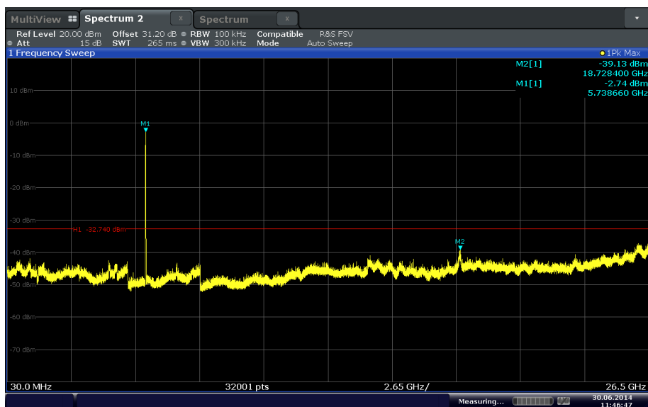
802.11a mode SISO Channel 149 (5745MHz)
