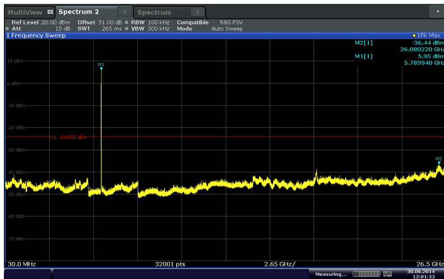
802.11n ht20 mode MIMO Channel 157 (5785MHz)
