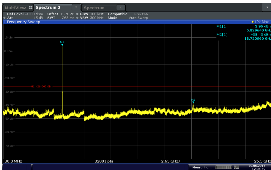
802.11n ht20 mode MIMO Channel 165 (5825MHz)
