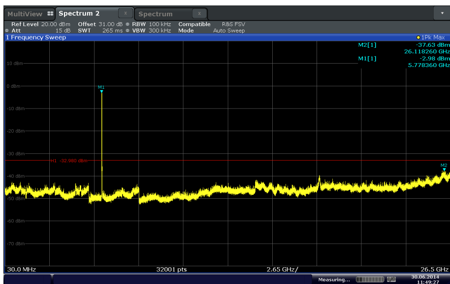
802.11a mode SISO Channel 157 (5785MHz)
