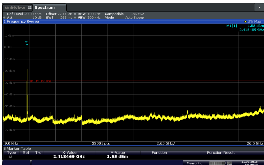
802.11g SISO mode Channel 2 (2417MHz)
