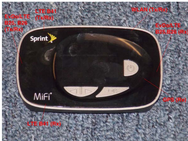
Antenna Location
