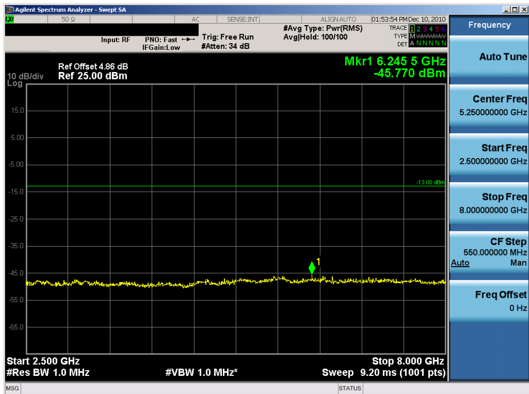
Plot 8-6. Conducted Spurious Plot (QPSK – RB Size 50)
