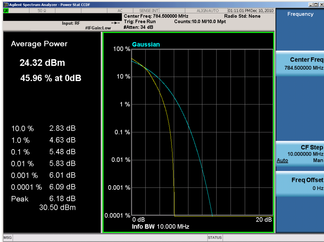
Plot 7-22. Peak-Average Ratio Plot (16-QAM – High Channel, RB Size 25)
