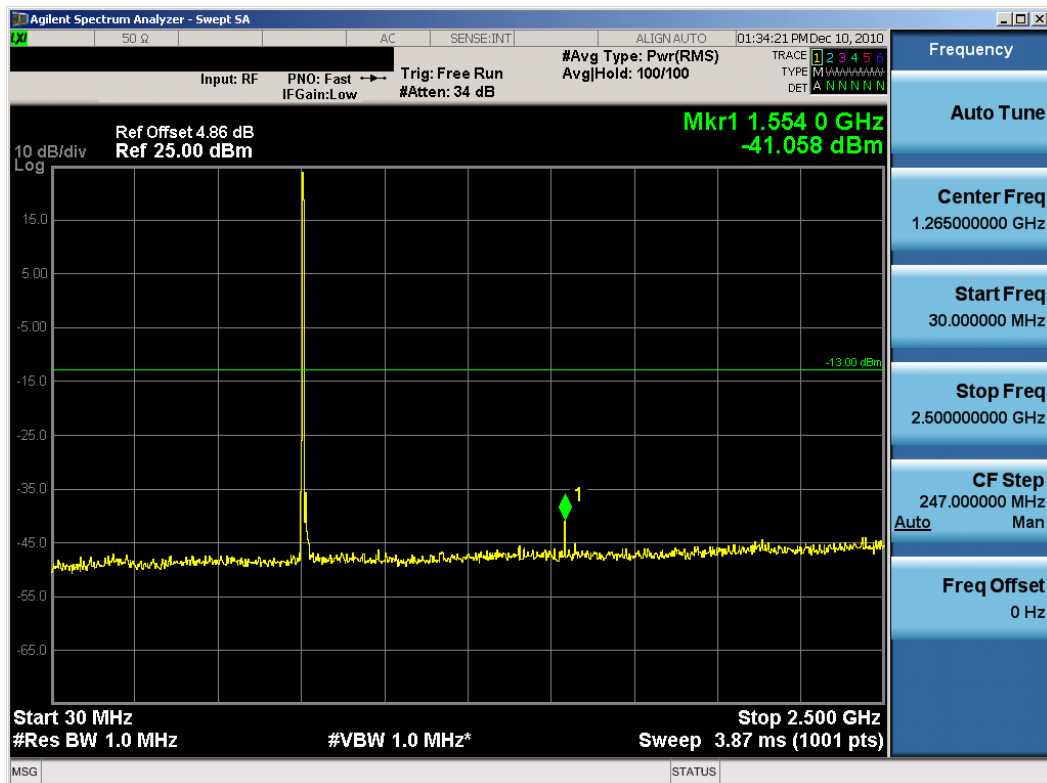
Plot 7-11. Conducted Spurious Plot (16-QAM – Low Channel, RB Size 25)
