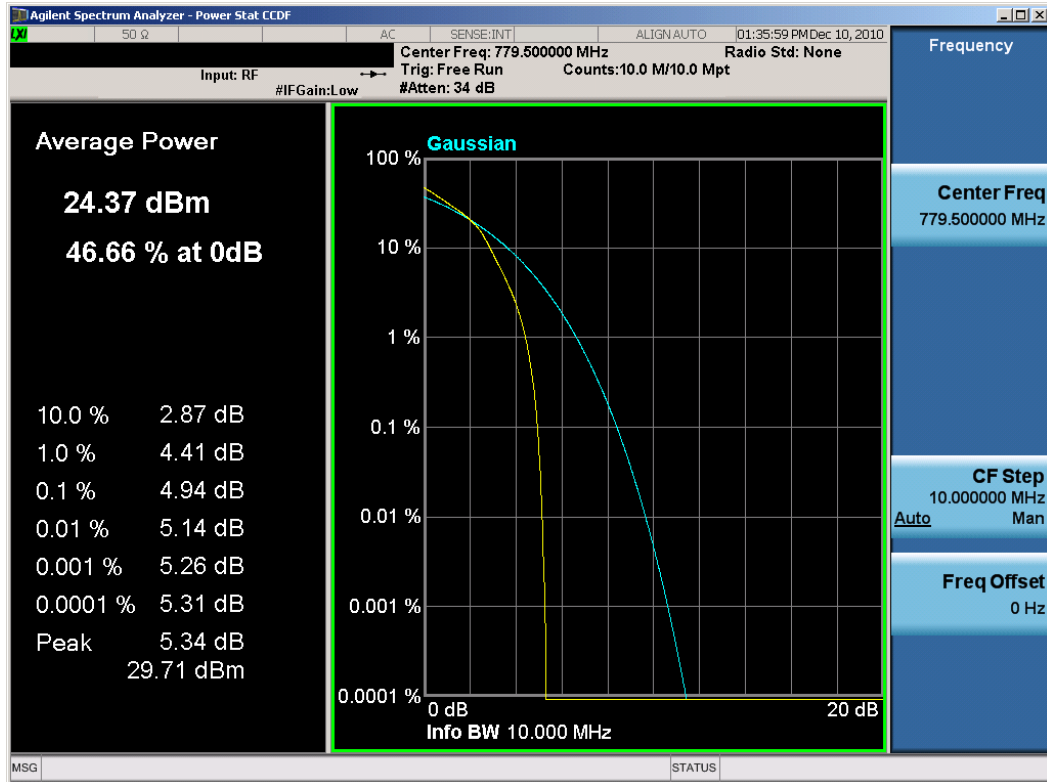
Plot 7-10. Peak-Average Ratio Plot (16-QAM – Low Channel, RB Size 25)
