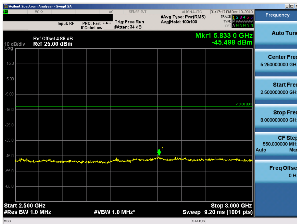
Plot 7-24. Conducted Spurious Plot (16-QAM – High Channel, RB Size 25)
