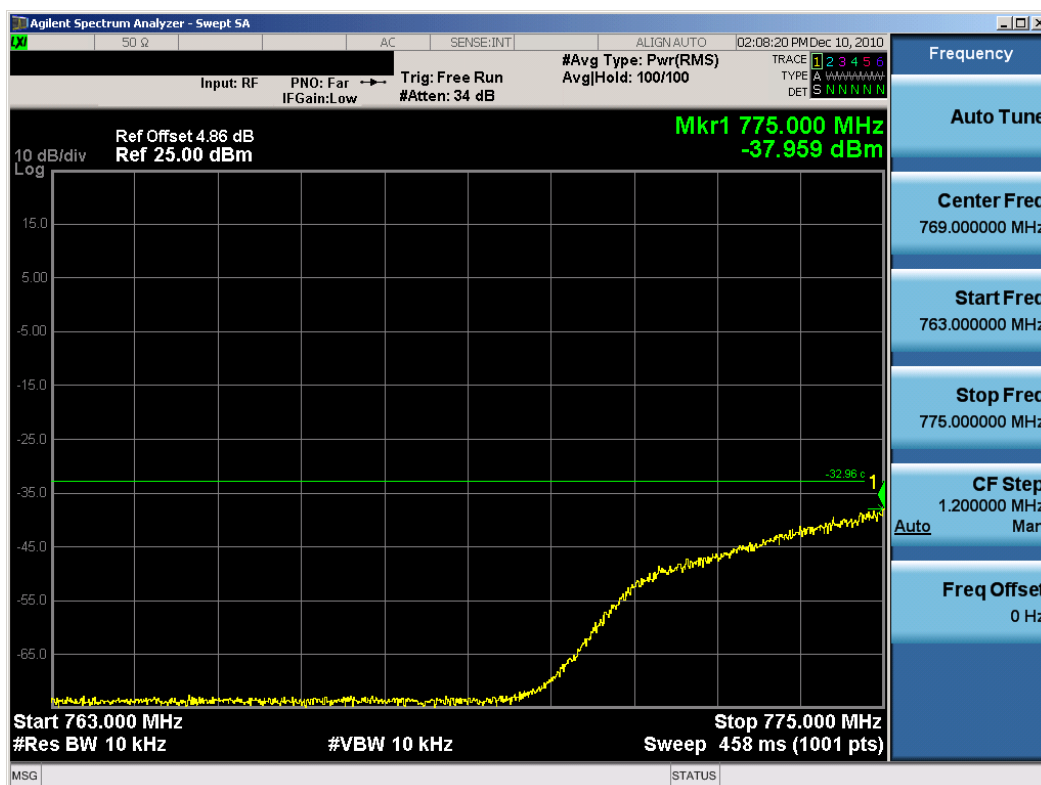
Plot 8-10. Lower Emission Mask (763 – 775MHz) Plot (16-QAM – RB Size 50)
