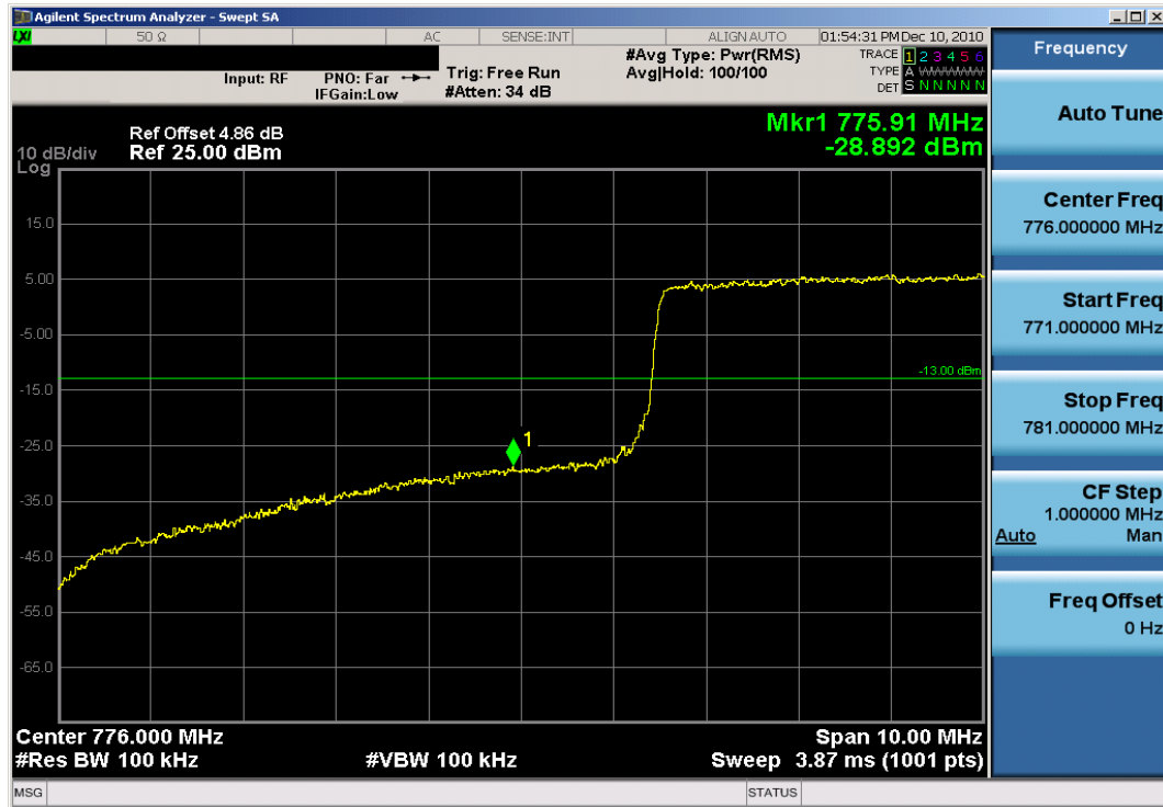
Plot 8-1. Lower Band Edge Plot (QPSK – RB Size 50)
