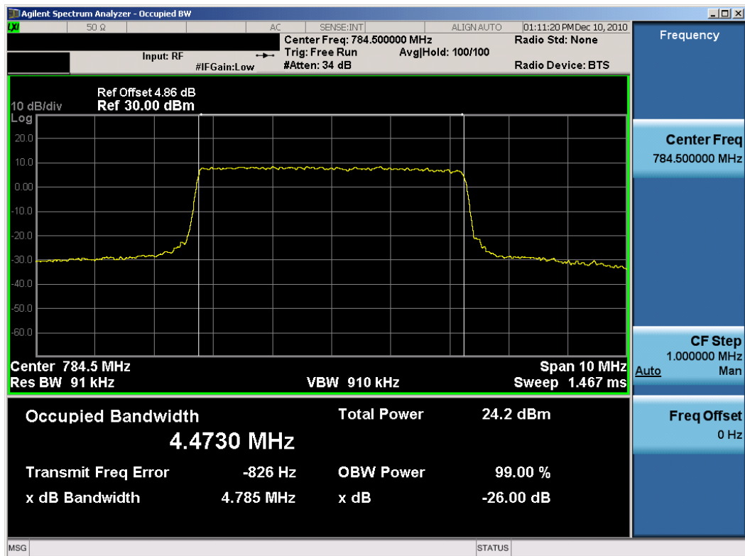
Plot 7-21. Occupied Bandwidth Plot (16-QAM – High Channel, RB Size 25)
