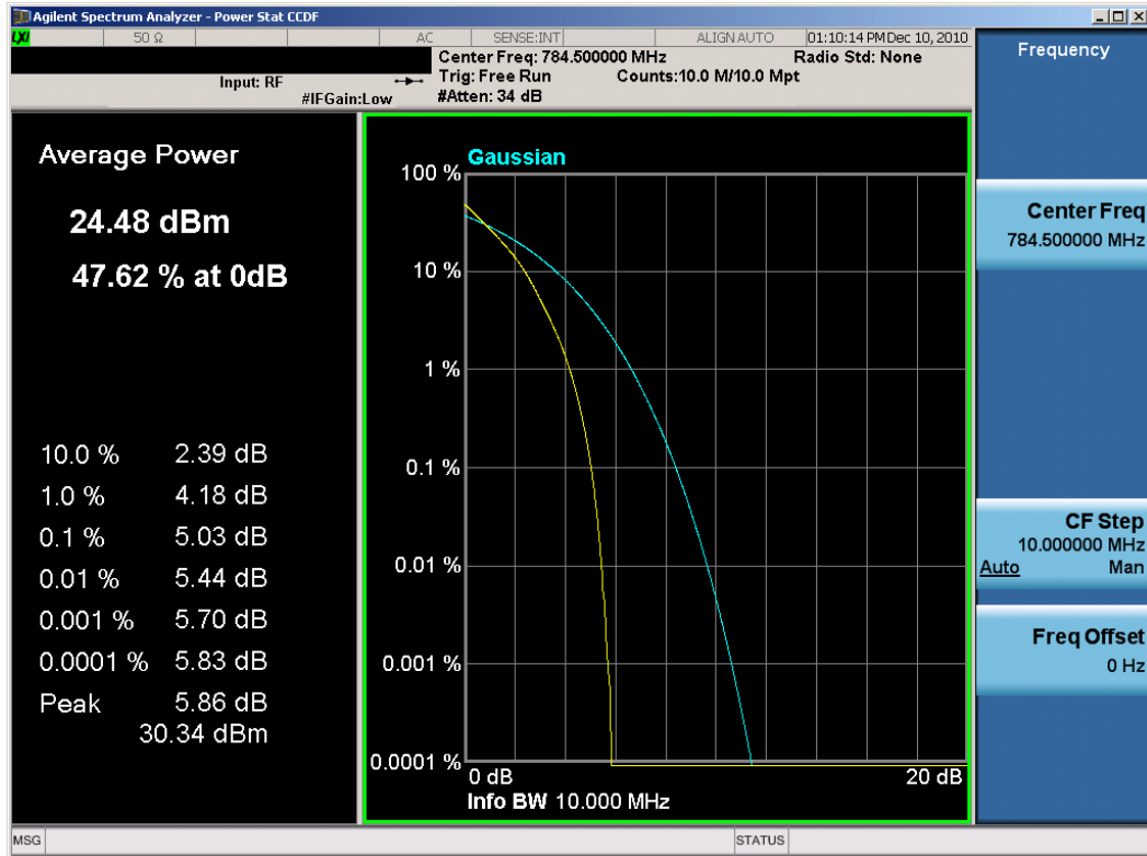
Plot 7-16. Peak-Average Ratio Plot (QPSK – High Channel, RB Size 25)
