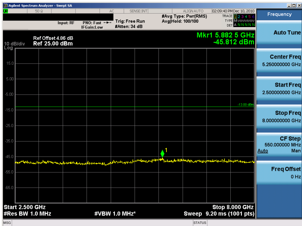
Plot 8-14. Conducted Spurious Plot (16-QAM – RB Size 50)
