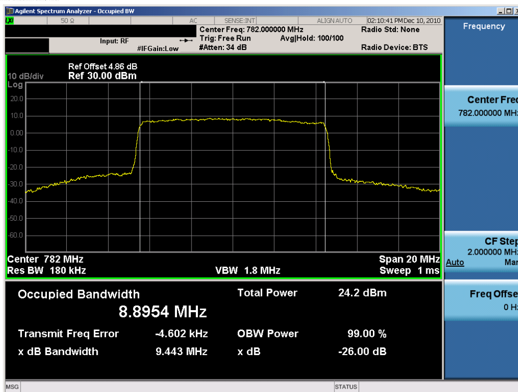
Plot 8-11. Occupied Bandwidth Plot (16-QAM – RB Size 50)
