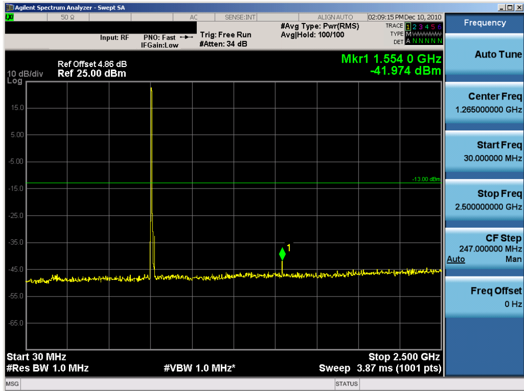
Plot 8-13. Conducted Spurious Plot (16-QAM – RB Size 50)
