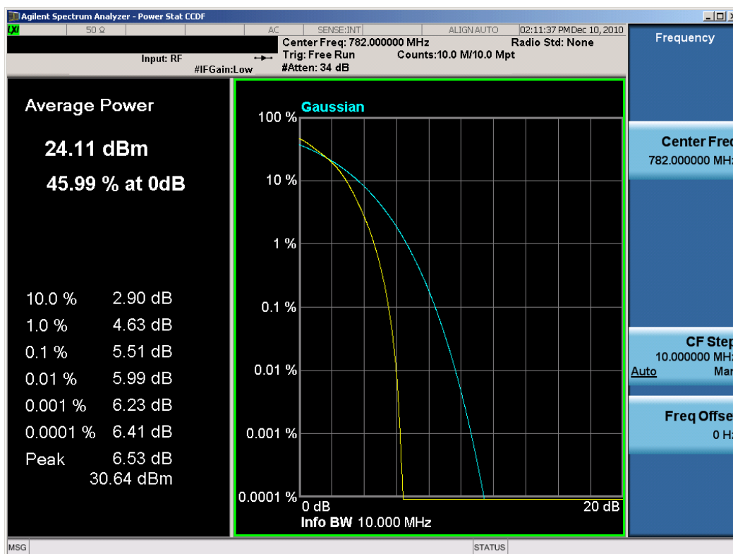
Plot 8-12. Peak-Average Ratio Plot (16-QAM – RB Size 50)
