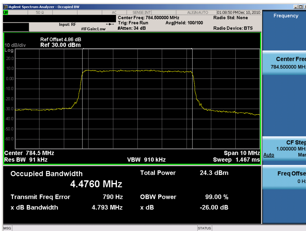
Plot 7-15. Occupied Bandwidth Plot (QPSK – High Channel, RB Size 25)
