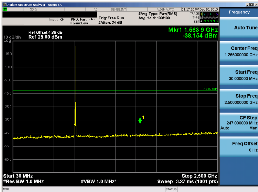
Plot 7-23. Conducted Spurious Plot (16-QAM – High Channel, RB Size 25)
