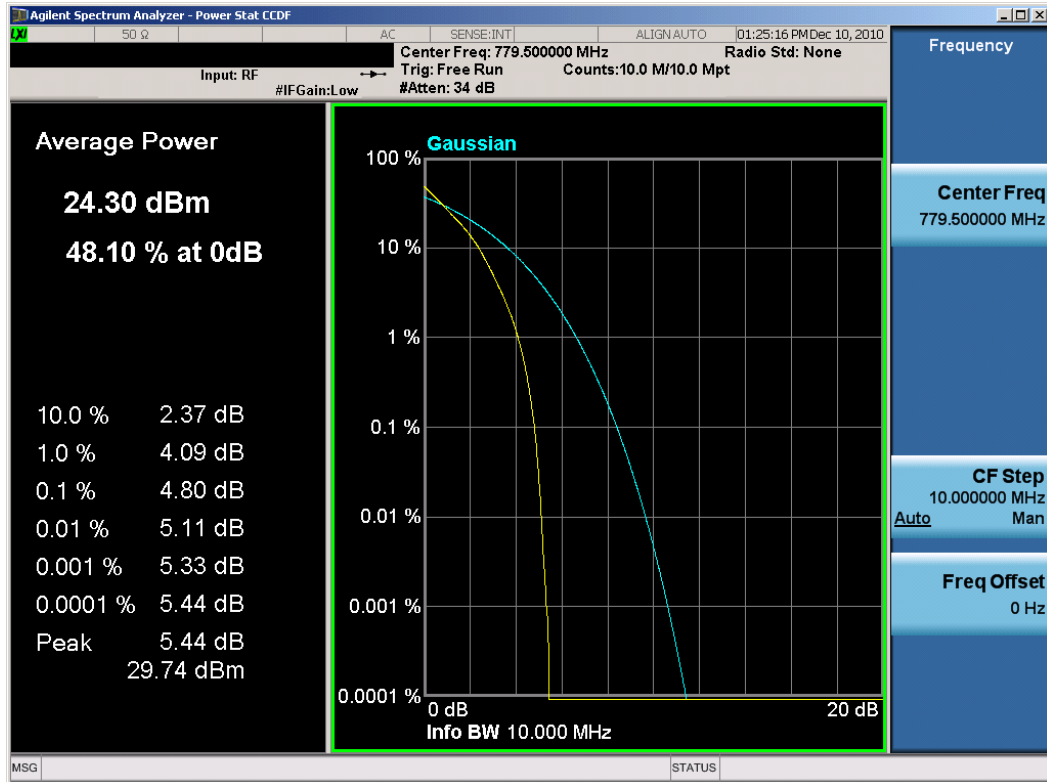
Plot 7-4. Peak-Average Ratio Plot (QPSK – Low Channel, RB Size 25)
