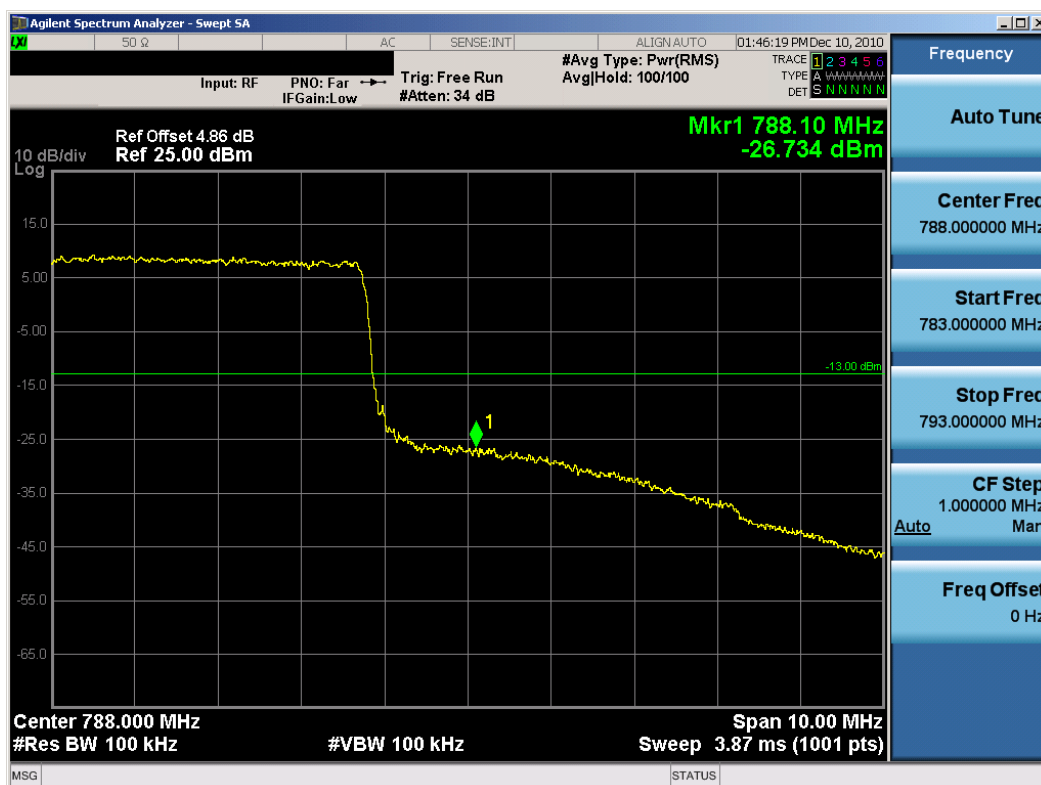
Plot 7-19. Upper Band Edge Plot (16-QAM – High Channel, RB Size 25)
