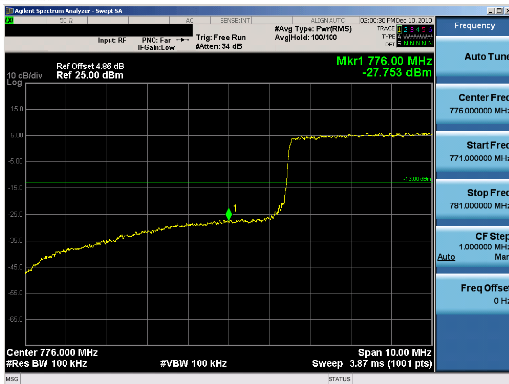
Plot 8-9. Lower Band Edge Plot (16-QAM – RB Size 50)
