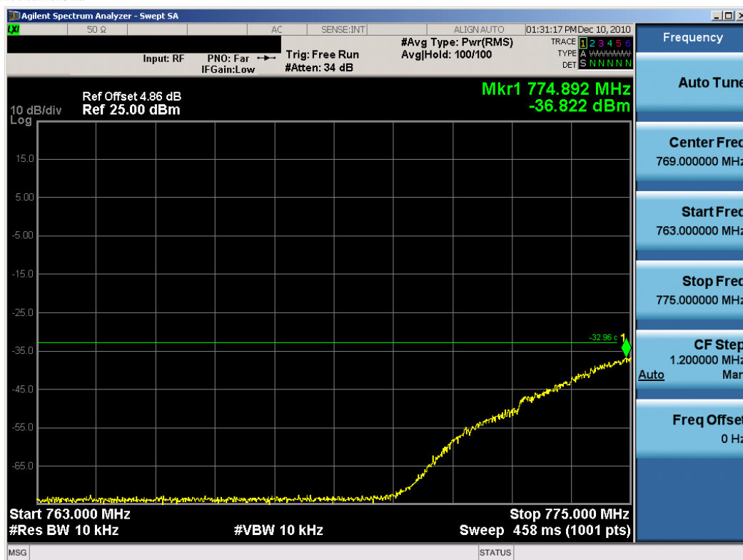
Plot 7-8. Lower Emission Mask (763 – 775MHz) Plot (16-QAM – Low Channel, RB Size 25)
