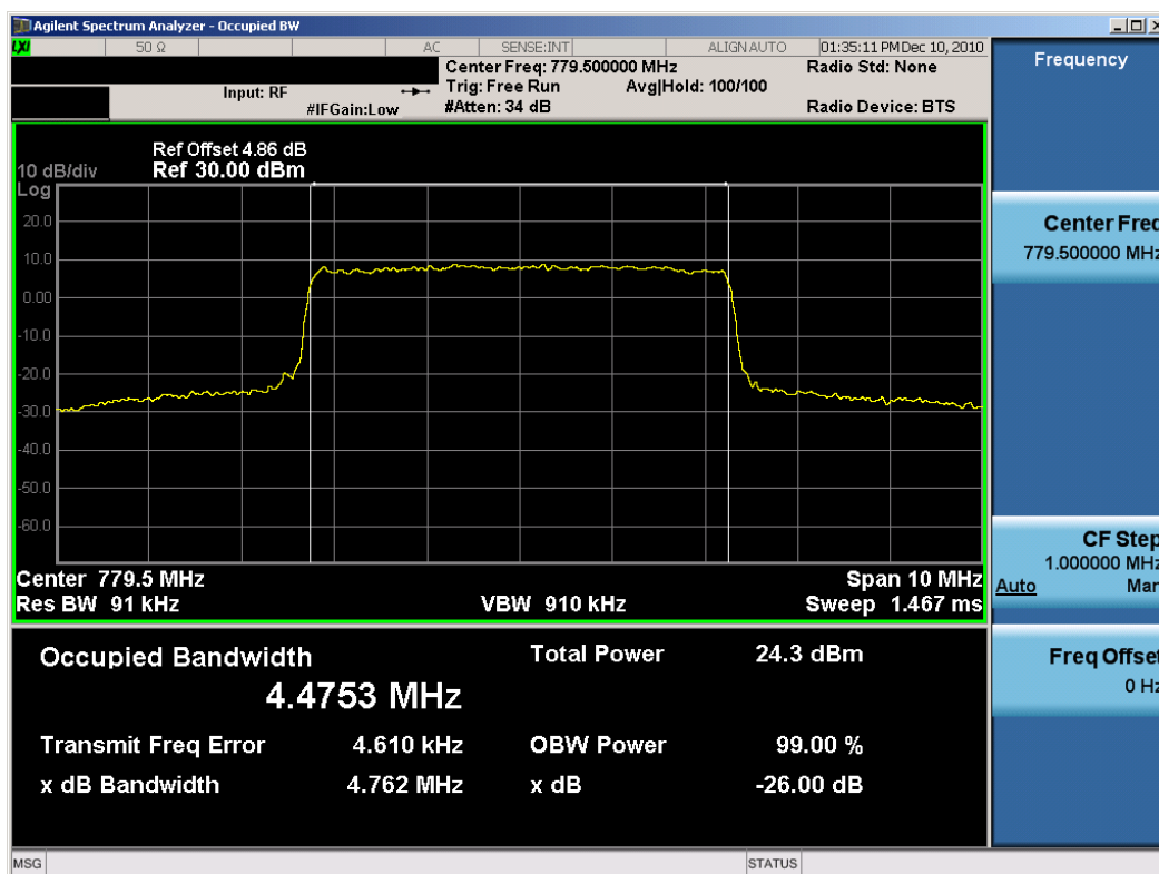
Plot 7-9. Occupied Bandwidth Plot (16-QAM – Low Channel, RB Size 25)
