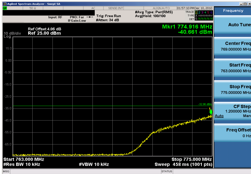
Plot 8-2. Lower Emission Mask (763 – 775 MHz) Plot (QPSK – RB Size 50)
