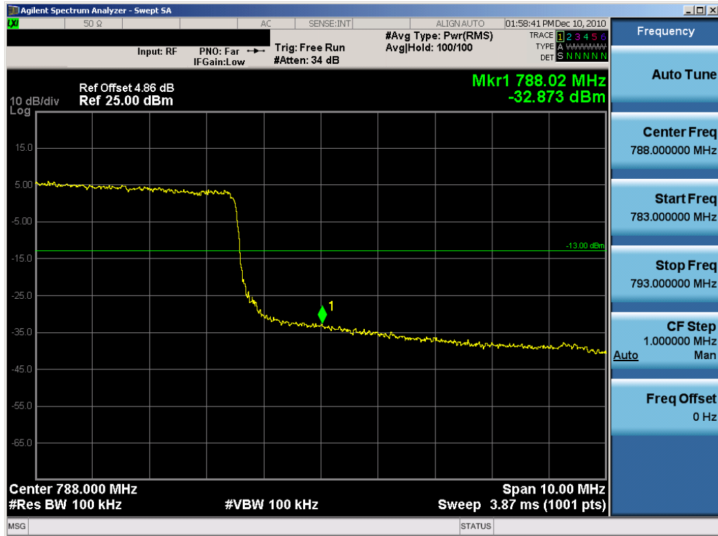
Plot 8-7. Upper Band Edge Plot (QPSK – RB Size 50)
