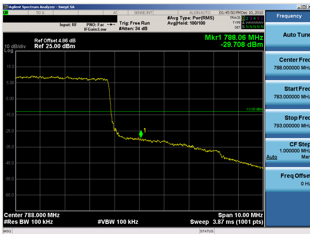
Plot 7-13. Upper Band Edge Plot (QPSK – High Channel, RB Size 25)
