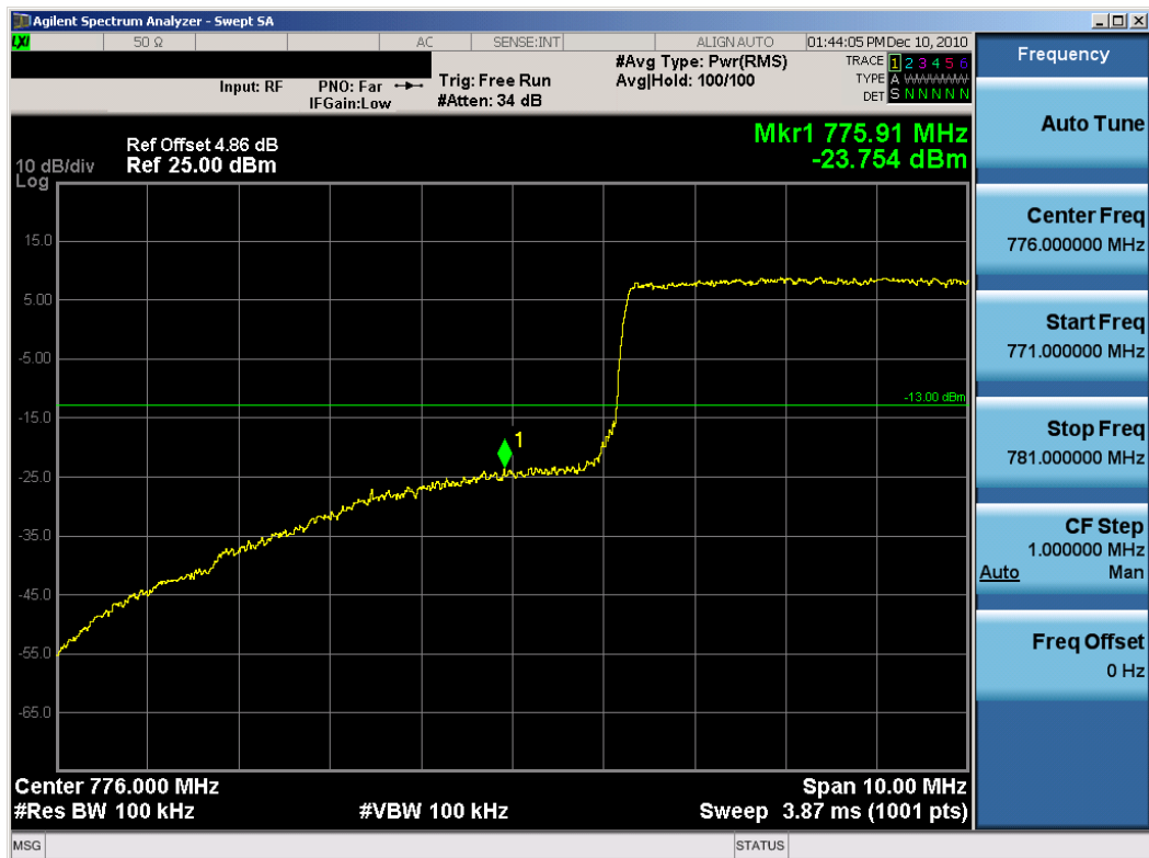
Plot 7-7. Band Edge Plot (16-QAM – Low Channel, RB Size 25)
