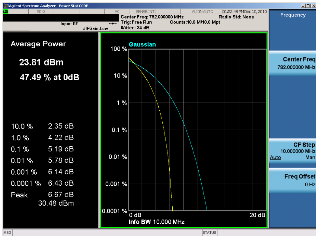
Plot 8-4. Peak-Average Ratio Plot (QPSK – RB Size 50)
