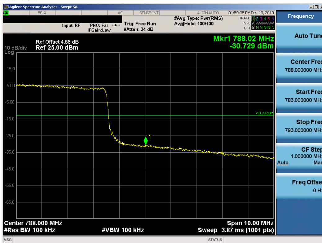
Plot 8-15. Upper Band Edge Plot (16-QAM – RB Size 50)
