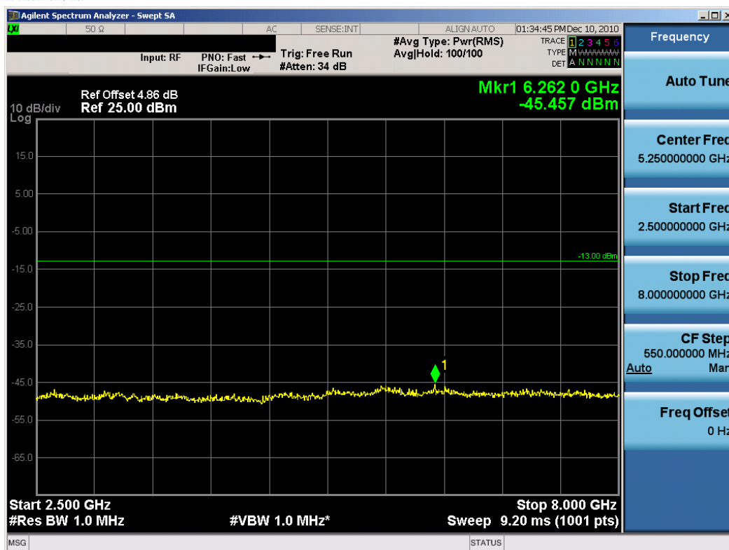
Plot 7-12. Conducted Spurious Plot (16-QAM – Low Channel, RB Size 25)
