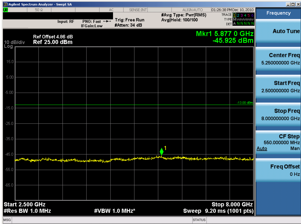
Plot 7-6. Conducted Spurious Plot (QPSK – Low Channel, RB Size 25)
