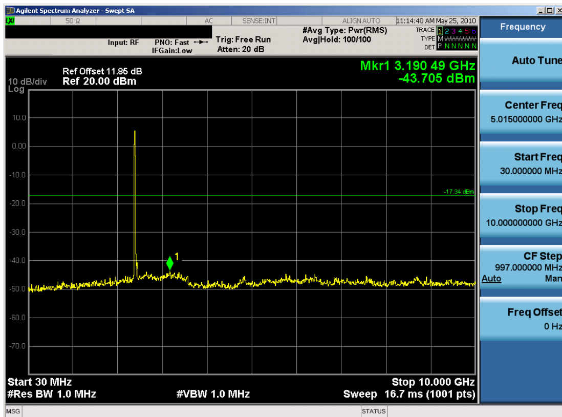
Plot 6-13. Conducted Spurious Plot (802.11b – Ch. 1)
