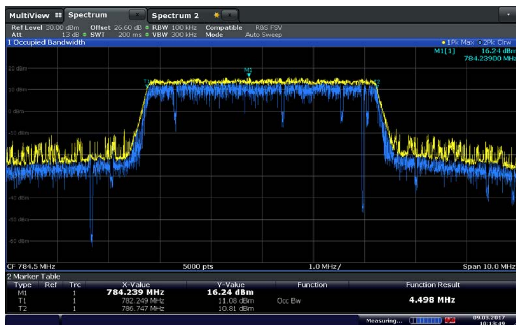
LTE Band 13 High Channel 99% OBW showing T_2 (F_H)
