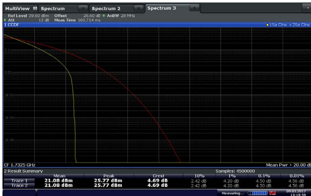
LTE Band 4 10MHz OBW Mid Channel QPSK PAPR
