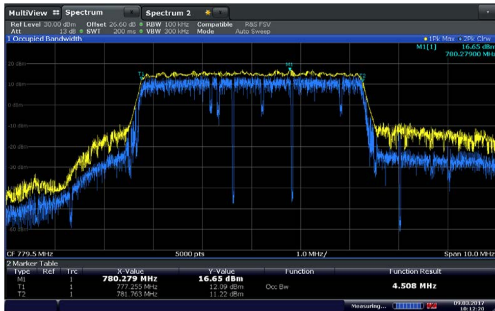
LTE Band 13 Low Channel 99% OBW showing T_1 (F_L)
