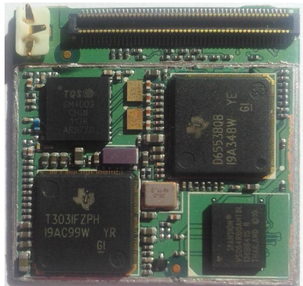
GSM0308 Internal
