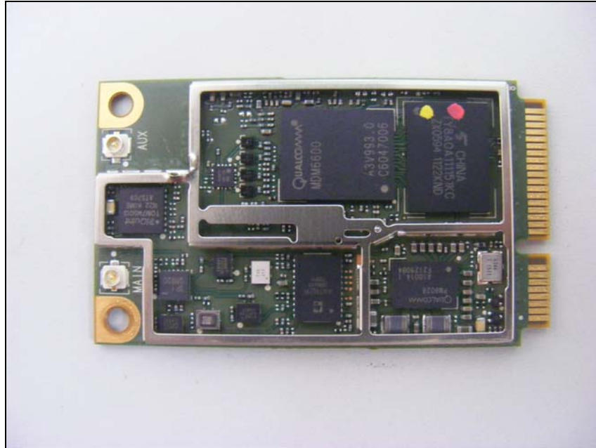
Top view of 2G, 3G Module
