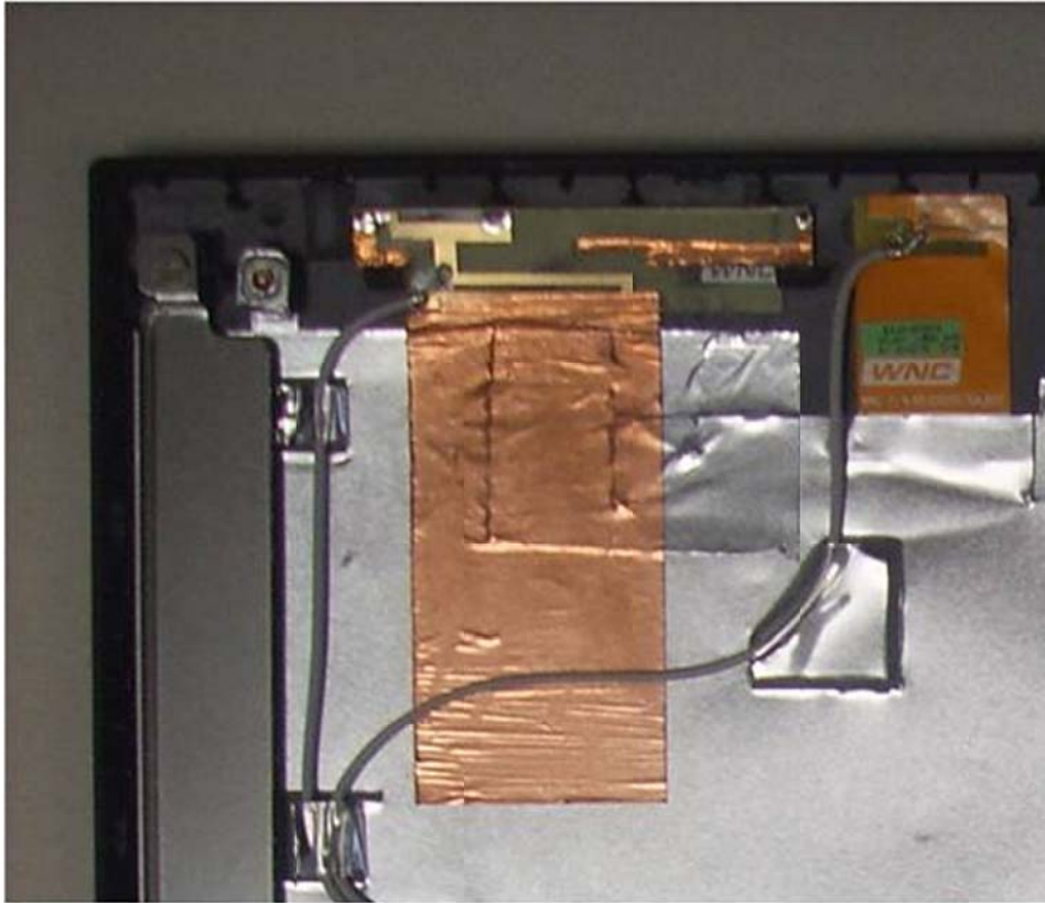
Main Antenna
