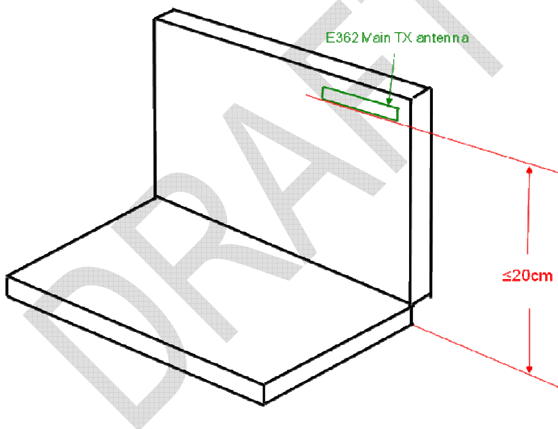
Figure 1-1 Determining Portable Antenna Locations
