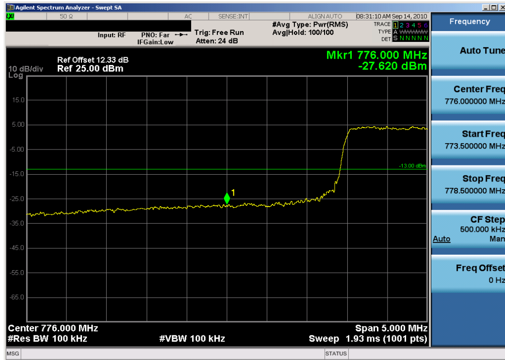
Plot 8-1. Lower Band Edge Plot (16-QAM – RB Size 50)
