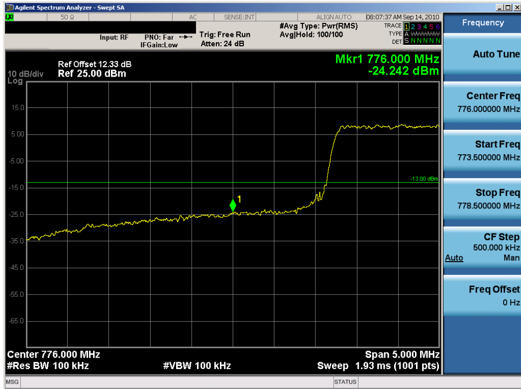
Plot 7-1. Lower Band Edge Plot (16-QAM – Low Channel, RB Size 25)
