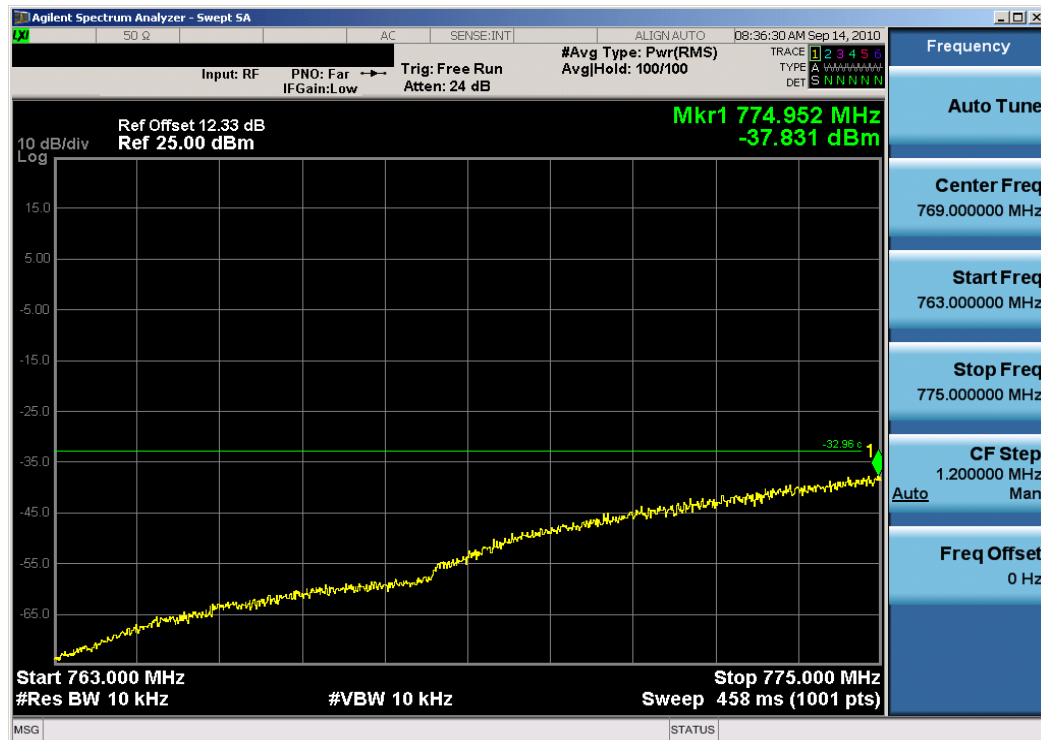
Plot 8-2. Lower Emission Mask (763 – 775MHz) Plot (16-QAM – RB Size 50)
